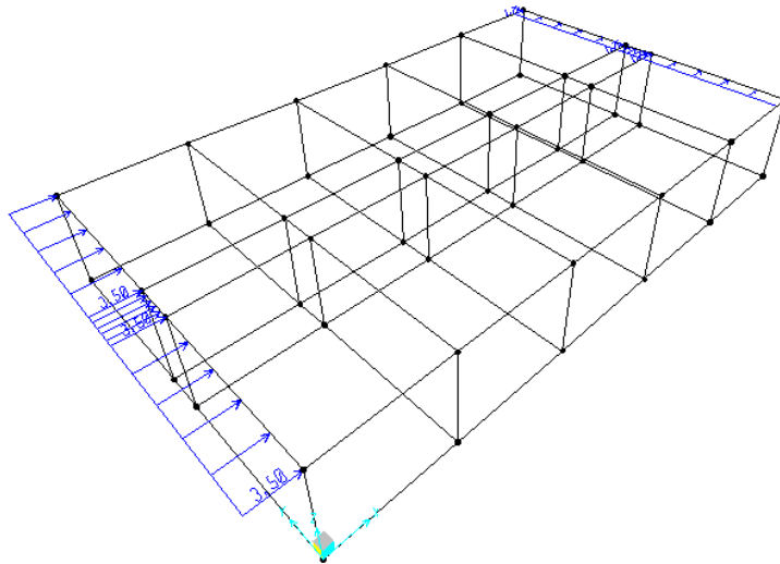
Vx+ – Vento X+
