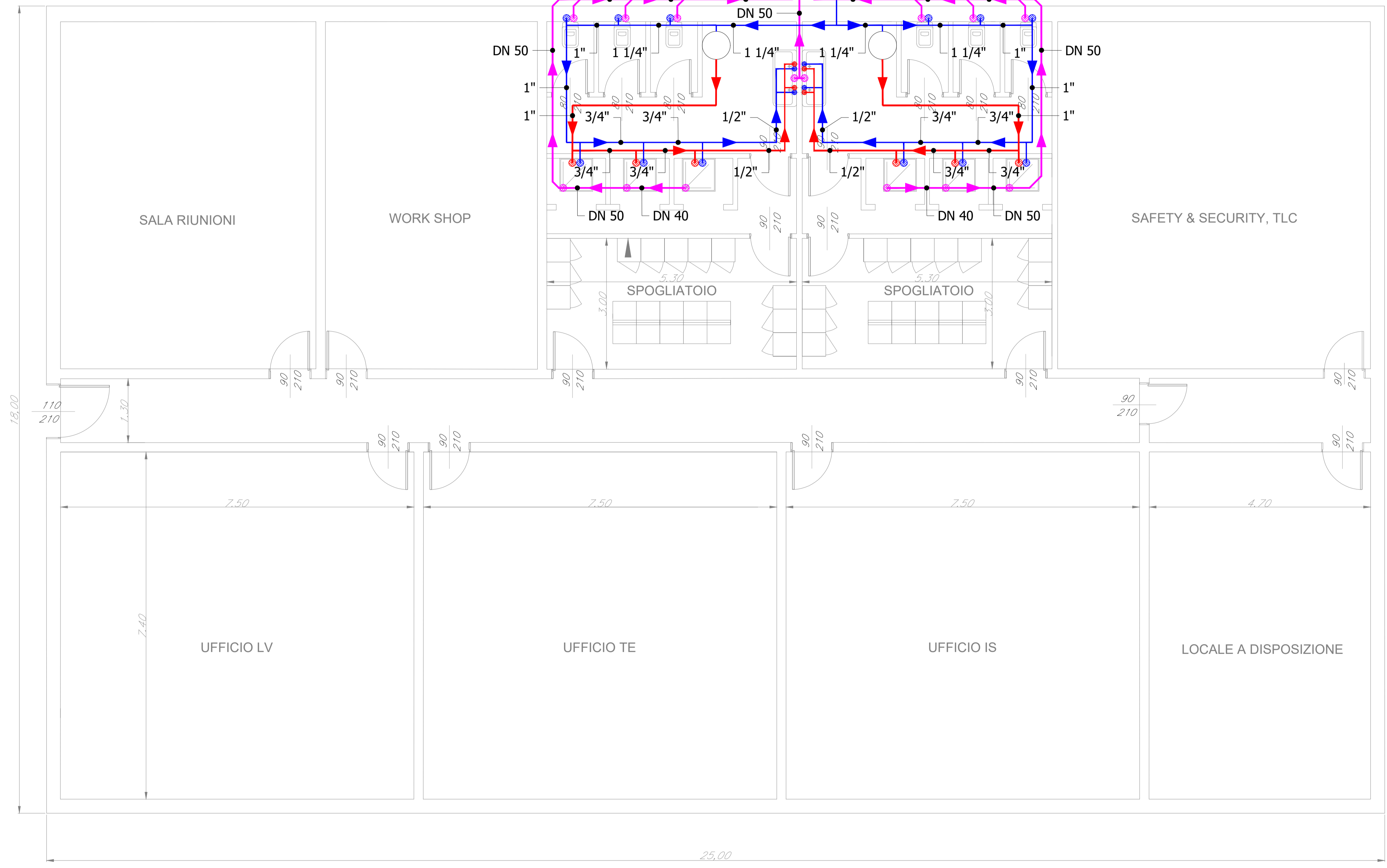
LAYOUT IMPIANTO IS
