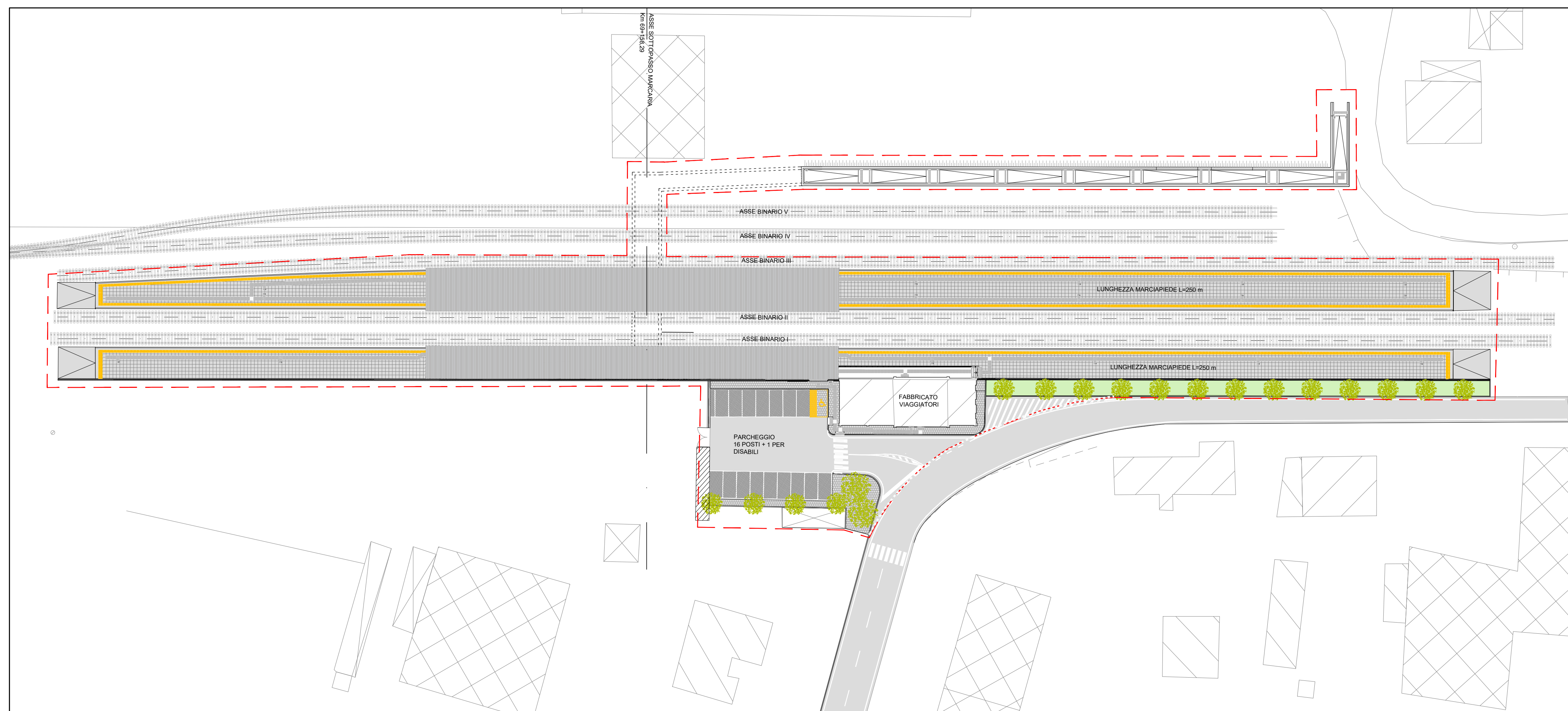
2 PLANIMETRIA POST OPERAM scala 1:500
