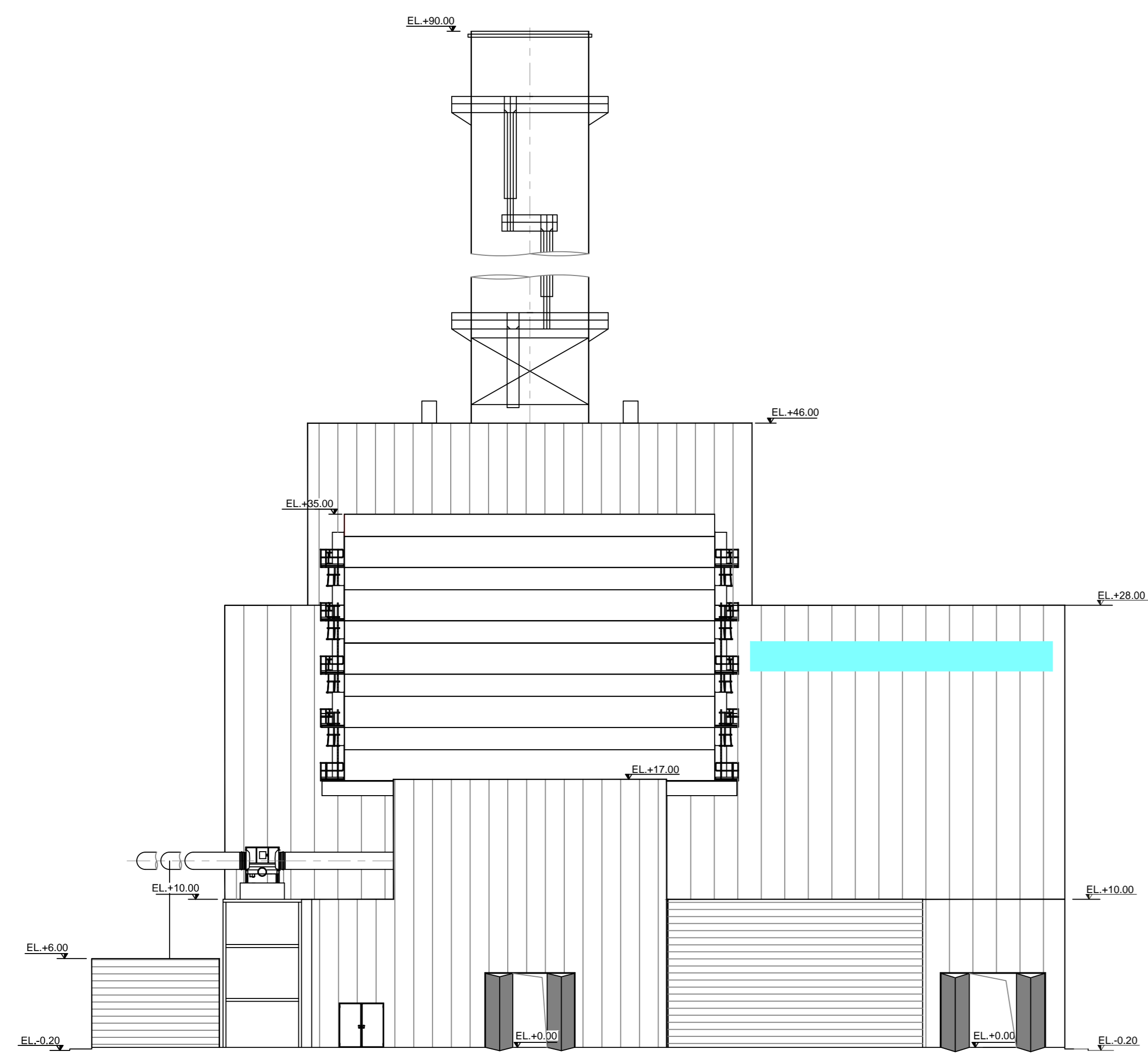
VIEW "B-B"
