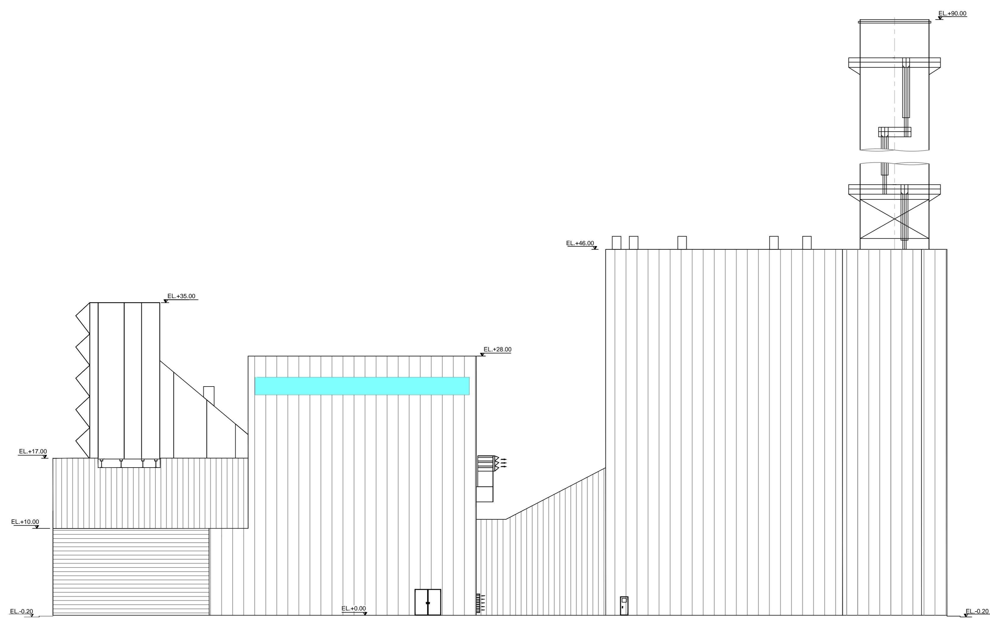
VIEW "C-C"
