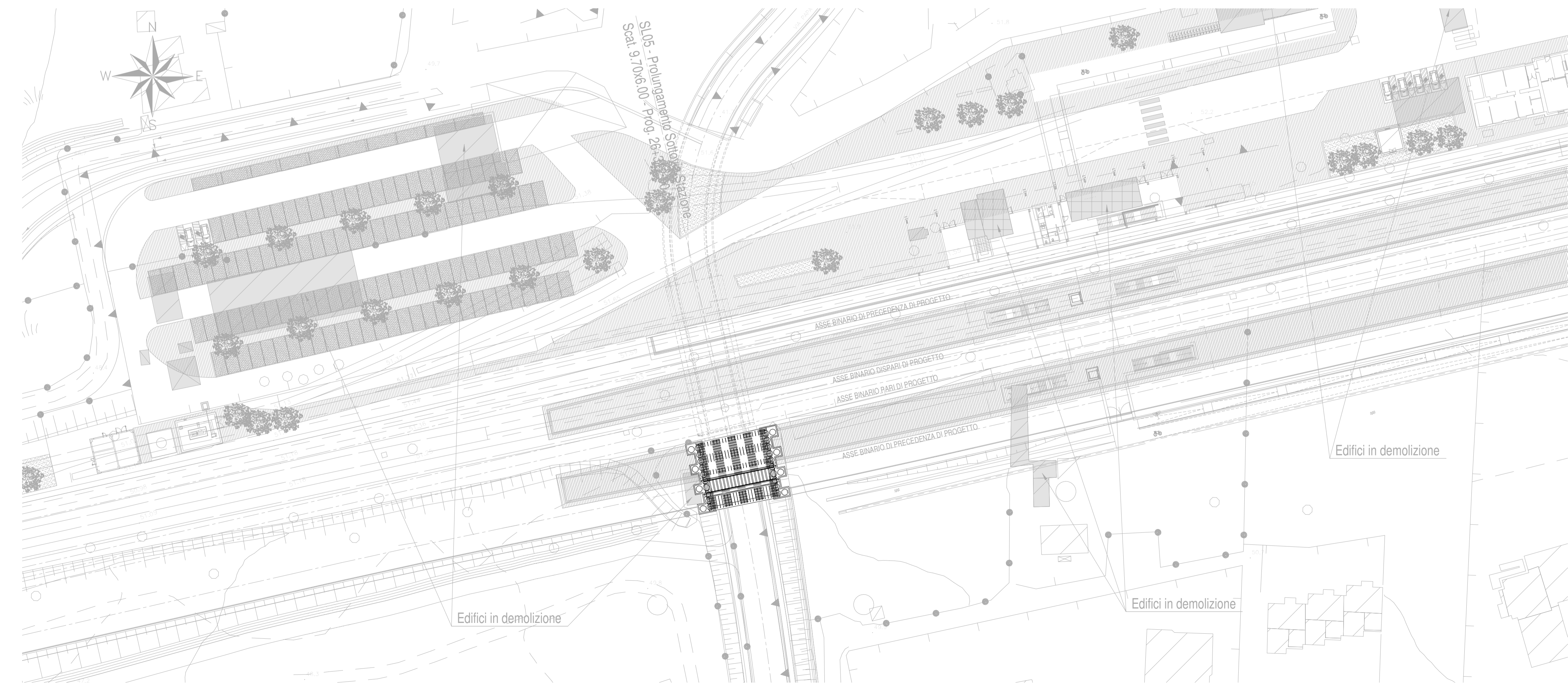
2 Planimetria Post Operam B8.SL.05.0.0.001 1 : 500
