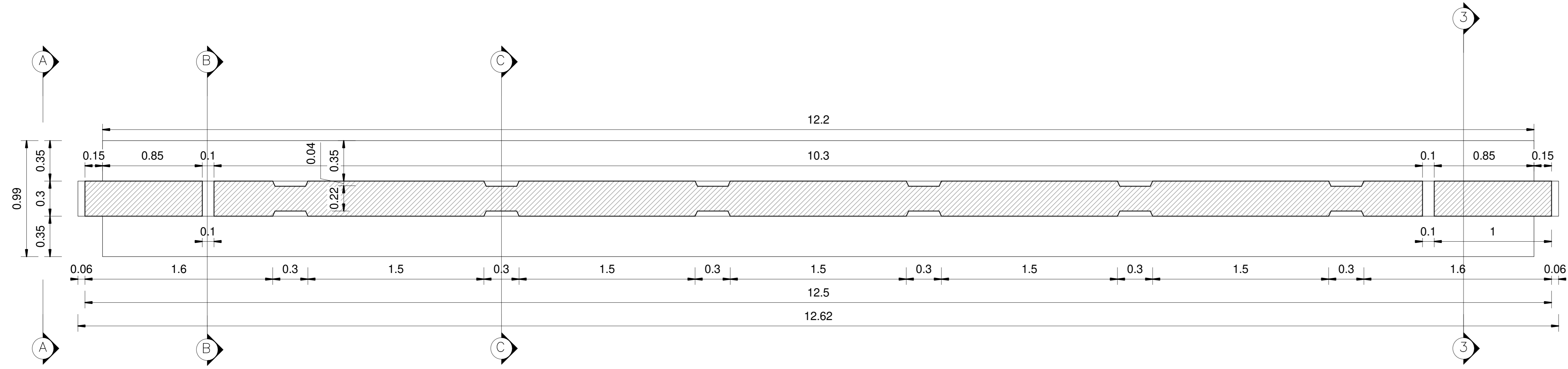
1 Trave in c.a.p. - Pianta 1 : 20
