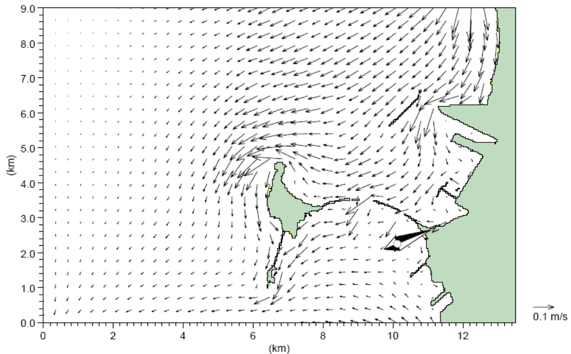
figure 8. Hydrodynamic simulation results considering wind conditions of 10 m/s with direction of 315°
