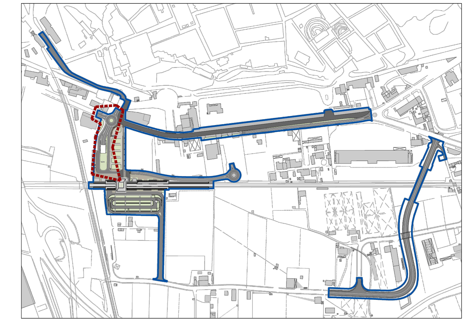
KEY PLAN - scala 1:5000
