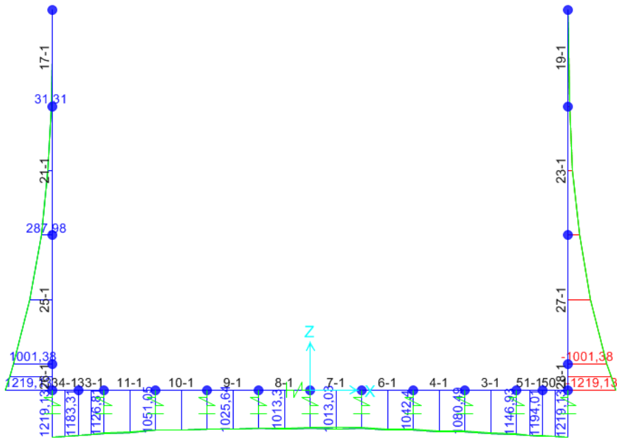
Figura 17: M – SLE RARA
