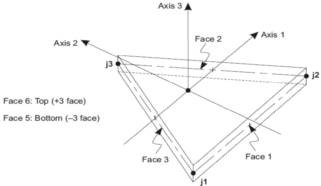
Three-node Triangular Shell Element
