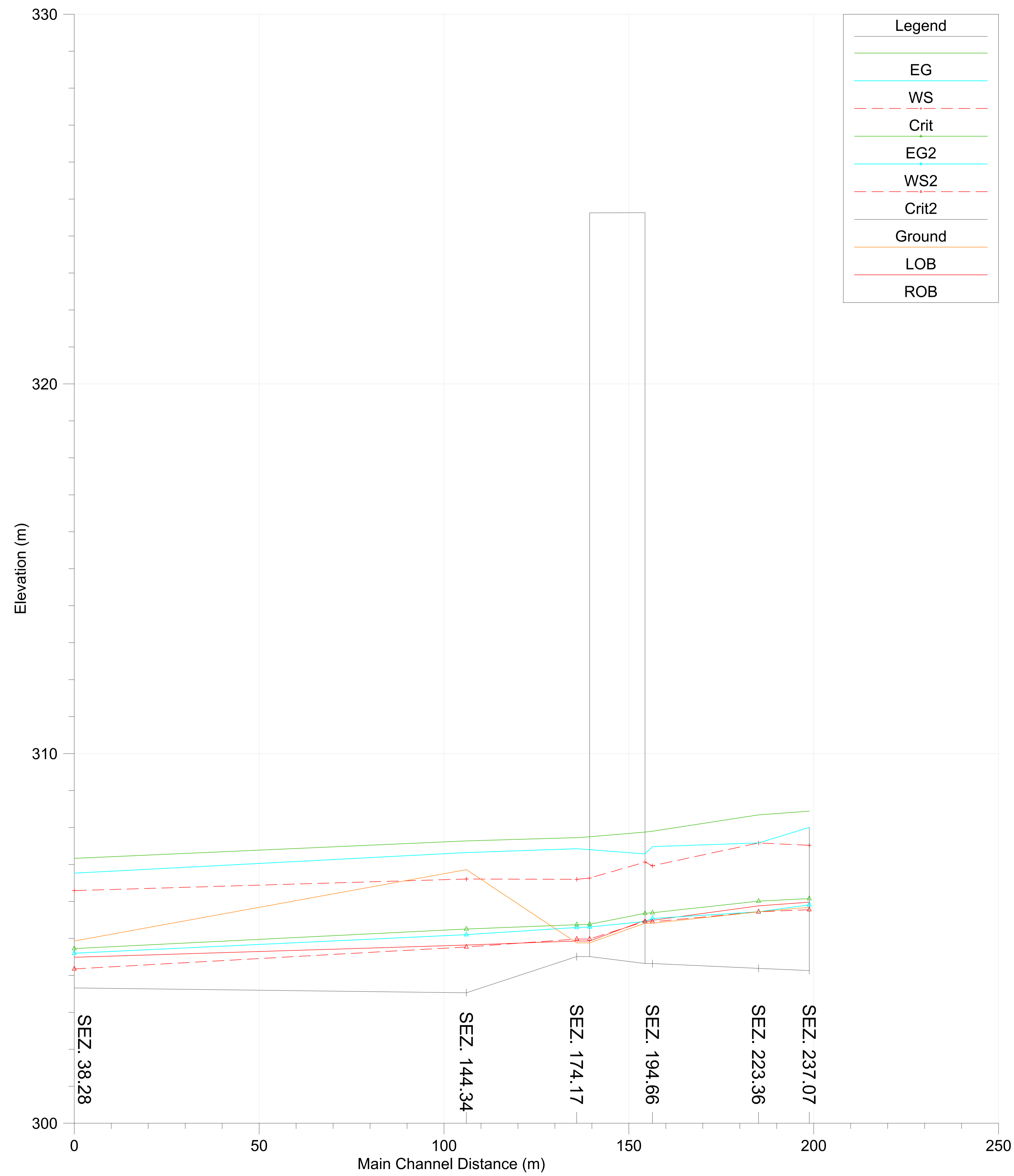
Profilo Post Operam - Scala 1:500/50 -
