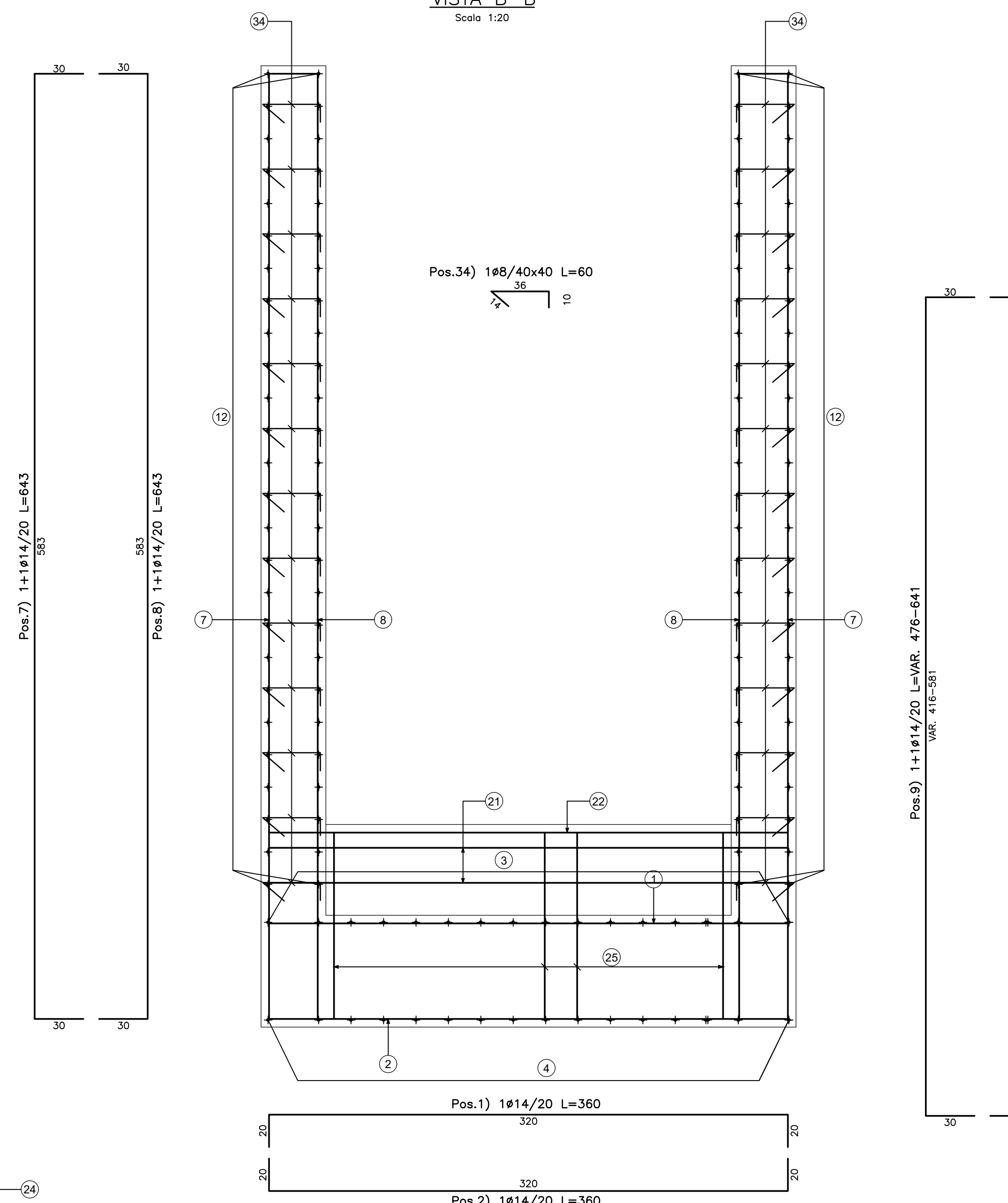
VISTA B-B Scale 1:20
