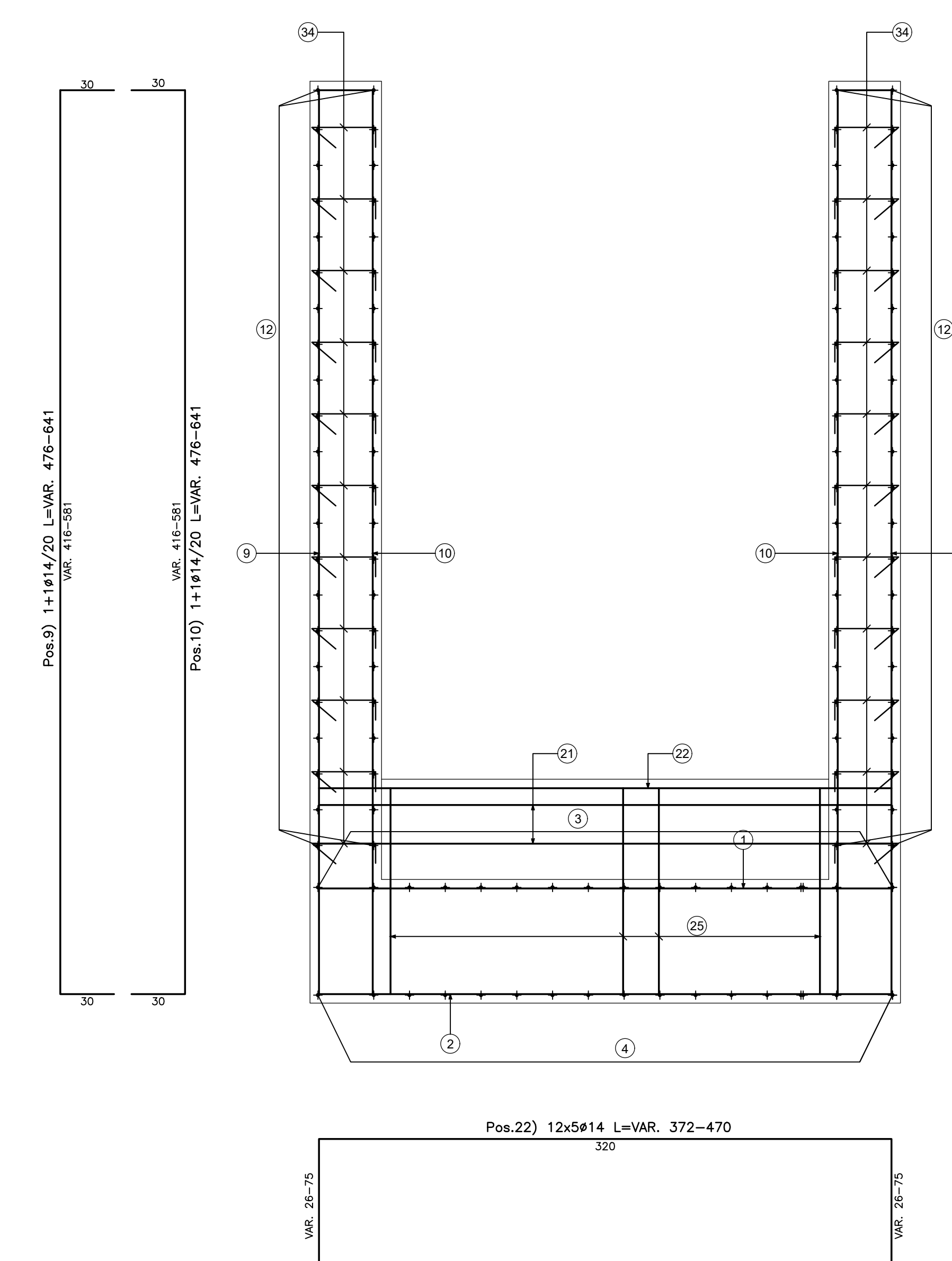
VISTA C-C Scale 1:20
