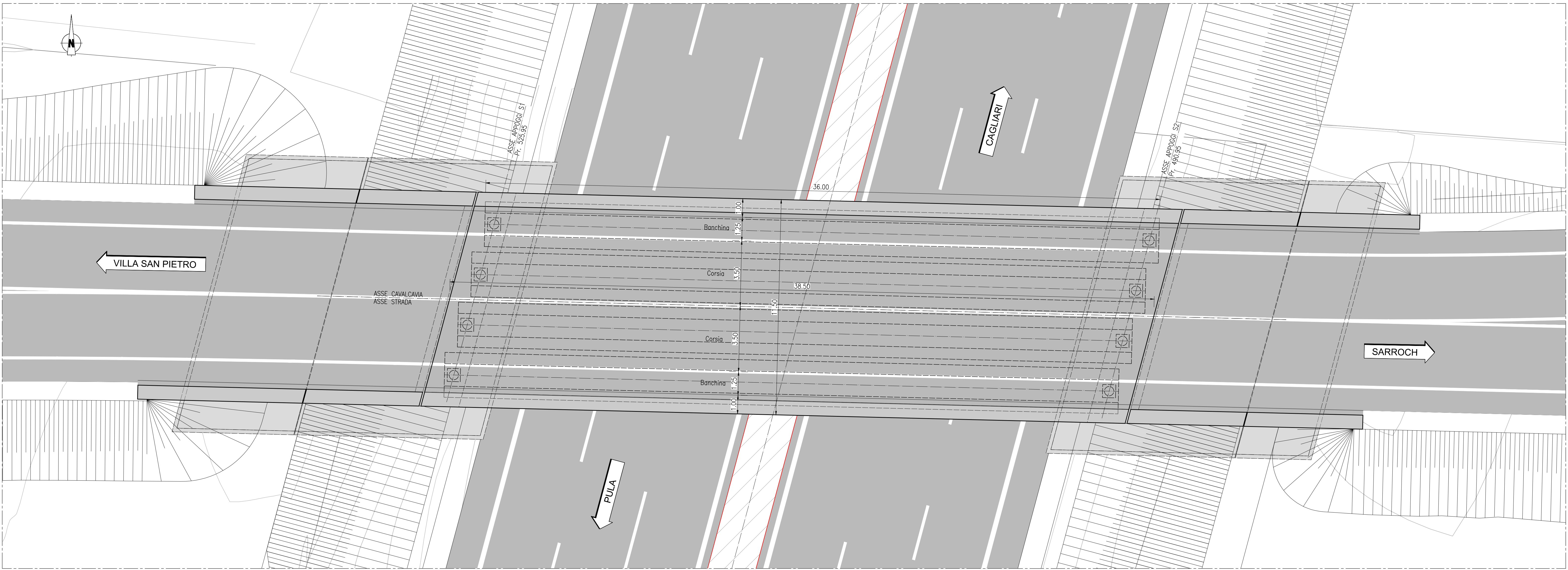
PLANIMETRIA (1:100)
