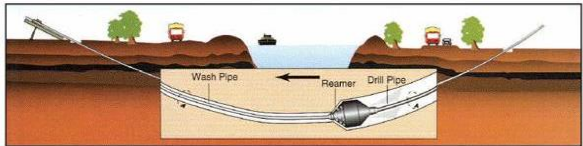
PRE-REAMING
