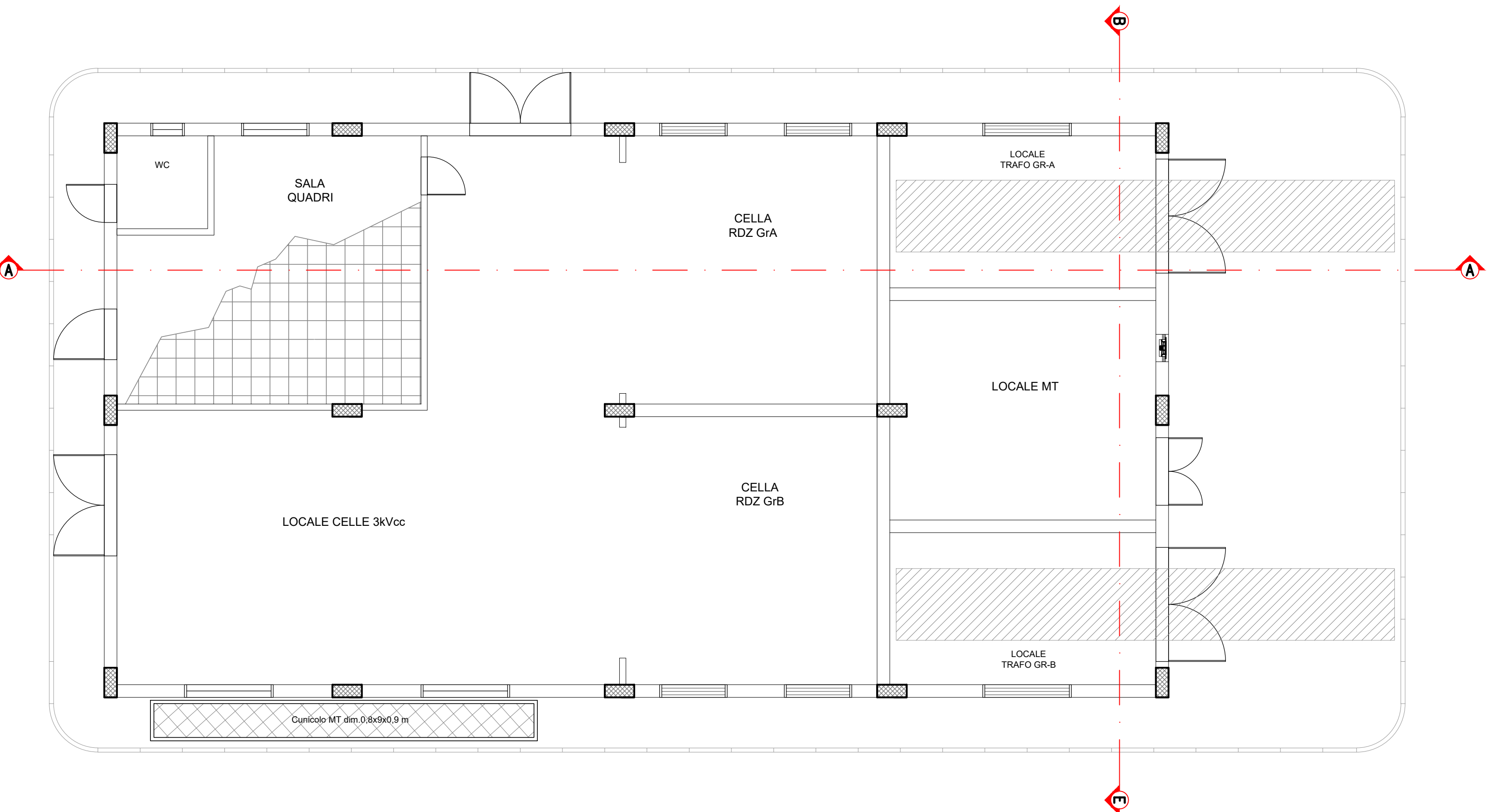
KEYPLAN (Scala 1:50)
