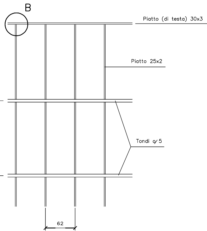
Part. B
