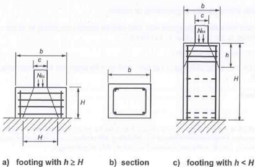
Figure 9.14: Splitting reinforcement in footing on rock
