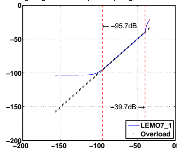
Level Linearity Test at 15.849Hz for Channel LEMO7_1 A-weighting Gain 0dB passed (Range: 48dB Tol.: 36dB)
