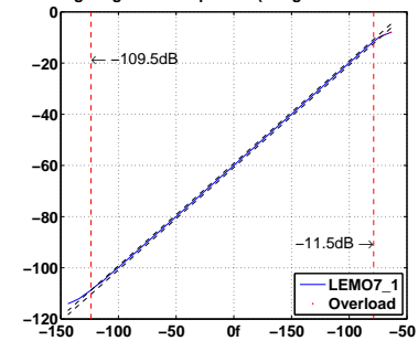
Level Linearity Test at 15.849Hz for Channel LEMO7_1 C-weighting Gain 0dB passed (Range: 98dB Tol.: 80dB)
