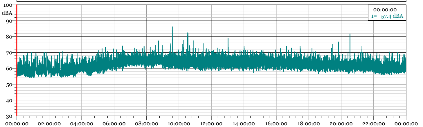
19121000.LD0 1/3 Leq Spectrum + SLM - LAeq
