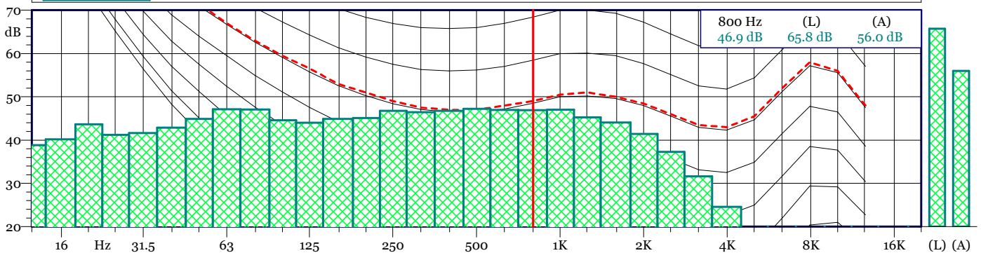
TRD 19121100.LD0 1/3 All Min Spectrum - Min
