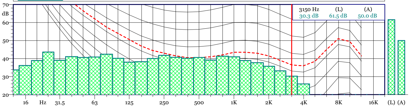
TRD 19120600.LD0 1/3 All Min Spectrum - Min
