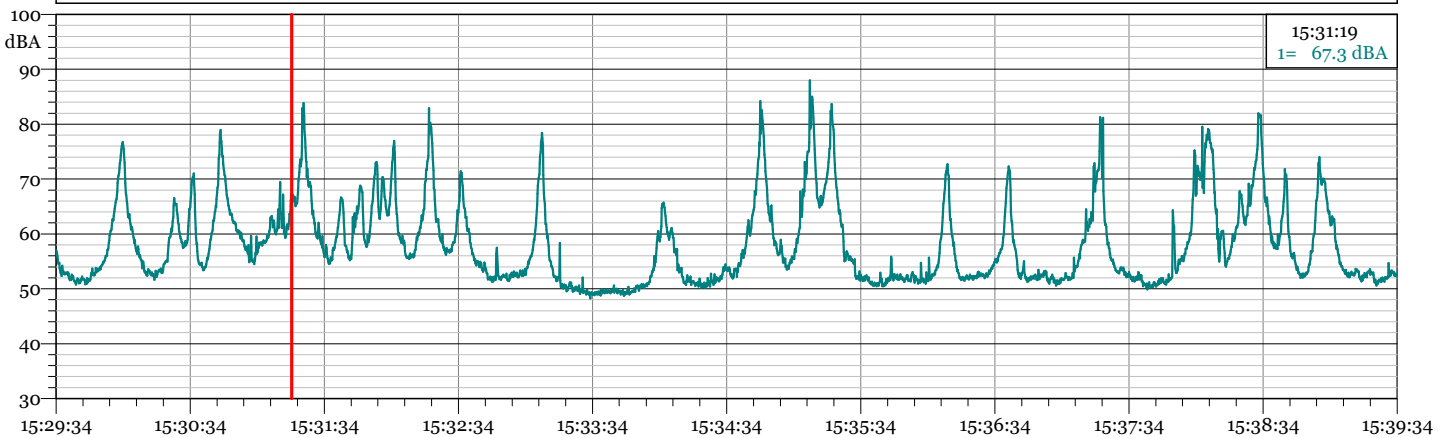
Esterne_.231 1/3 Leq Spectrum + SLM - LAeq L 90 = 51.0 dB(A) L95 = 50.2 dB(A)
