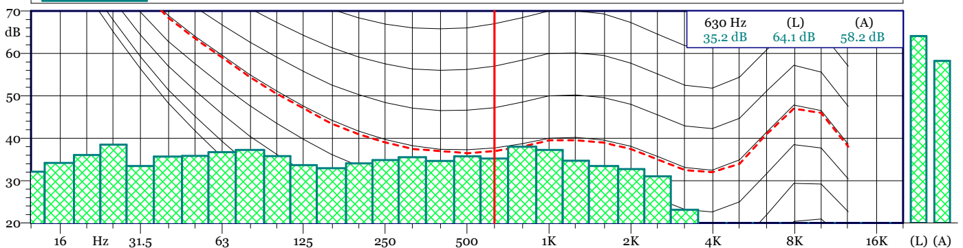
19120800.LD0 1/3 All Min Spectrum - Min
