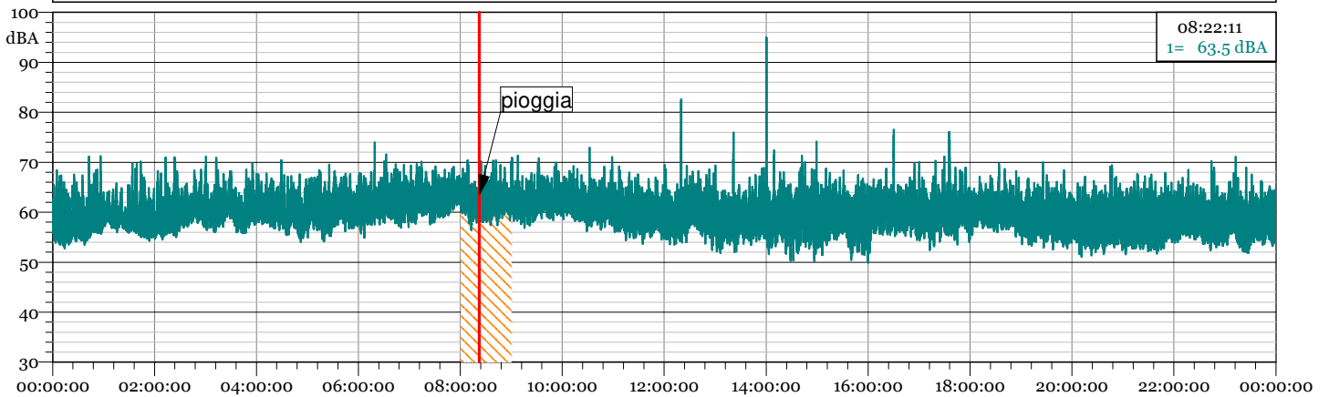
19120700.LD0 1/3 Leq Spectrum + SLM - LAeq
