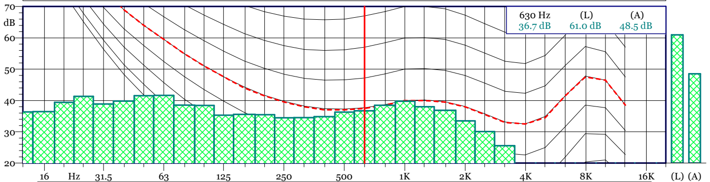
TRD 19120600.LD0 1/3 SPL Spectrum - Min
