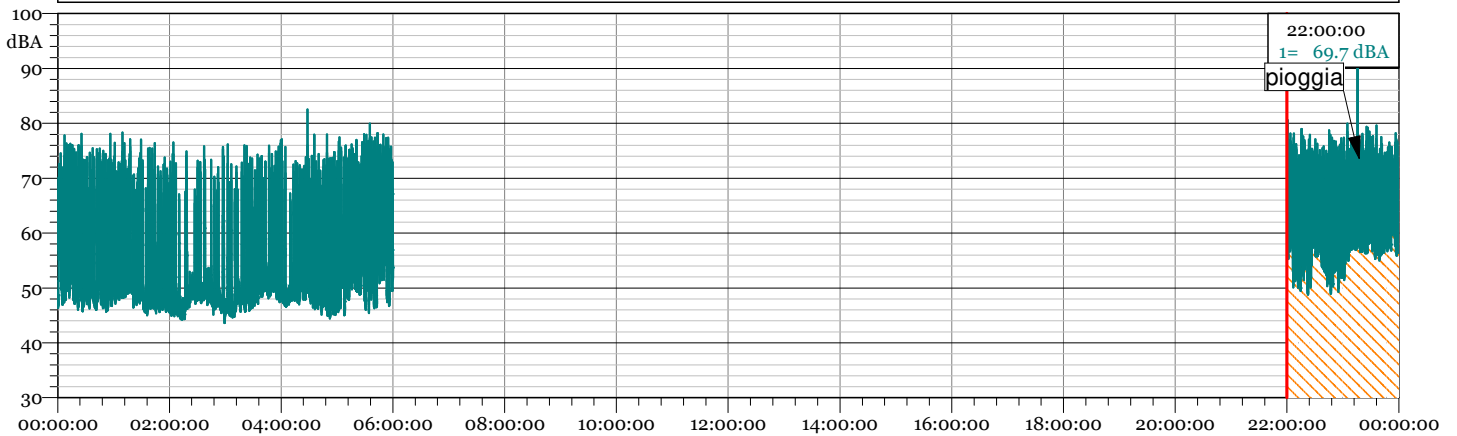
1 - TRN 19120600.LDo - 1/3 Leq Spectrum + SLM - LAeq
