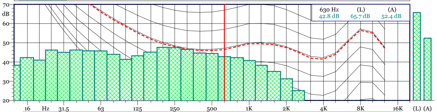
TRD 19121100.LDo 1/3 SPL Spectrum - Min
