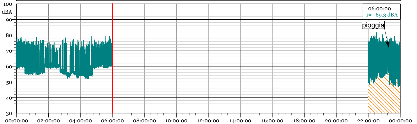
1 - TRN 19120500.LDo - 1/3 Leq Spectrum + SLM - LAeq
