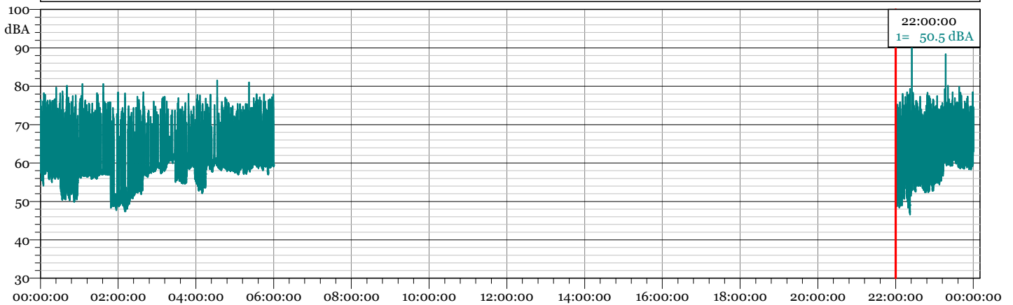
1 - TRN 19120700.LDo - 1/3 Leq Spectrum + SLM - LAeq
