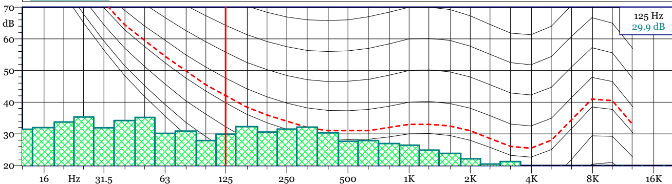
19120300.LD0 Intv 1/3 All Min Spectrum - Min
