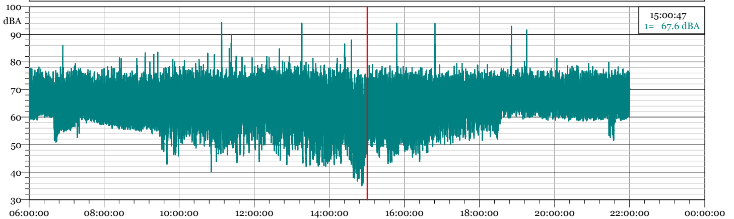
1 - TRD 19120800.LDo - 1/3 Leq Spectrum + SLM - LAeq
