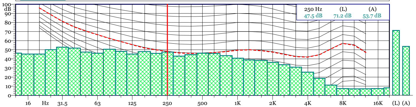
Esterne_.173 - 1/3 All Min Spectrum - Min
