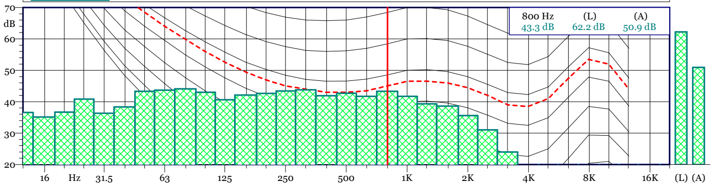
TRN 19120500.LD0 1/3 All Min Spectrum - Min
