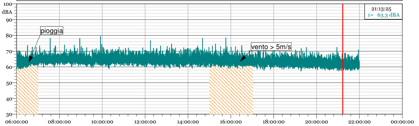
1 - TRD 19121100.LD0 - 1/3 Leq Spectrum + SLM - LAeq
