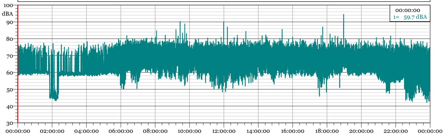
19120900.LD0 1/3 Leq Spectrum + SLM - LAeq
