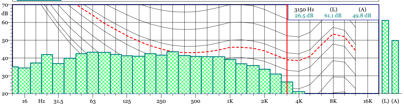
TRN 19120600.LD0 1/3 All Min Spectrum - Min
