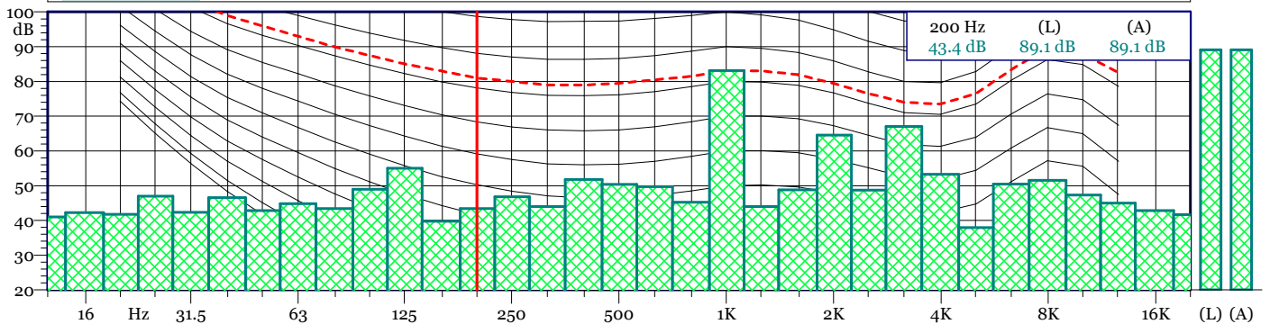
19120400.LD0 - 1/3 All Min Spectrum - Min
