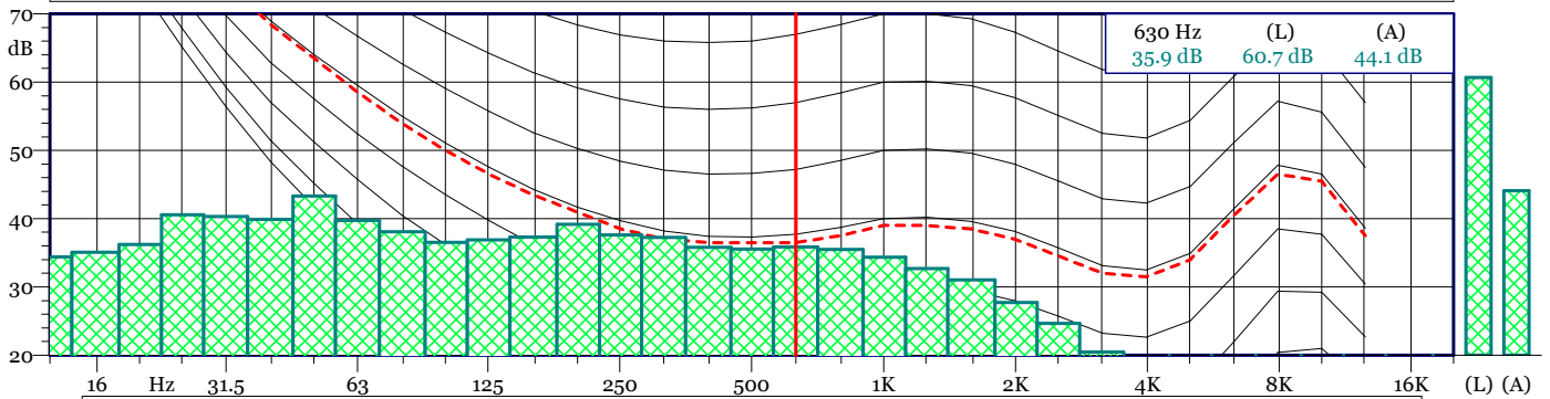
TRN 19120800.LDo 1/3 SPL Spectrum - Min
