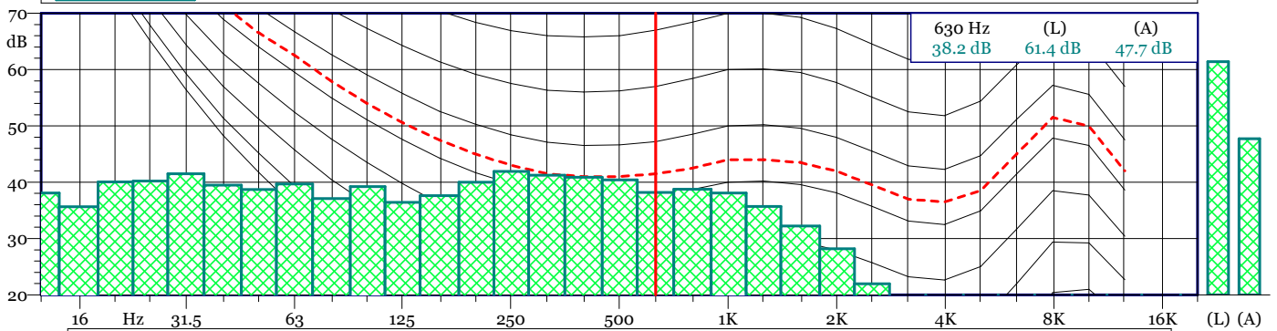
TRN 19121200.LD0 1/3 SPL Spectrum - Min
