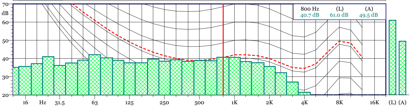
TRD 19120500.LDo - 1/3 All Min Spectrum - Min
