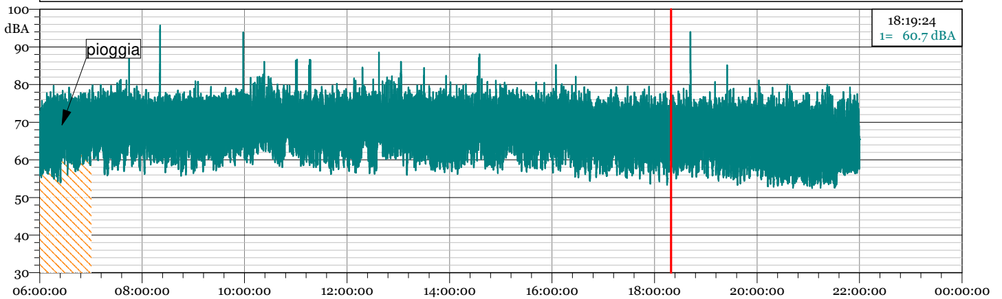
1 - TRD 19121100.LDo - 1/3 Leq Spectrum + SLM - LAeq
