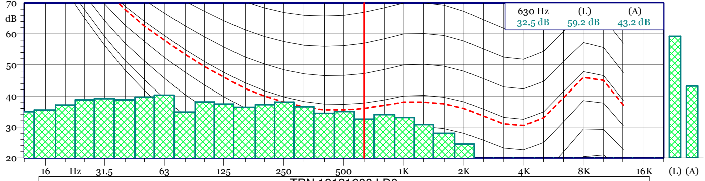
TRN 19121000.LDo 1/3 SPL Spectrum - Min
