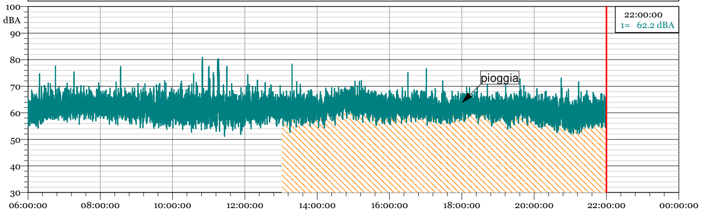
1 - TRD 19120600.LD0 - 1/3 Leq Spectrum + SLM - LAeq
