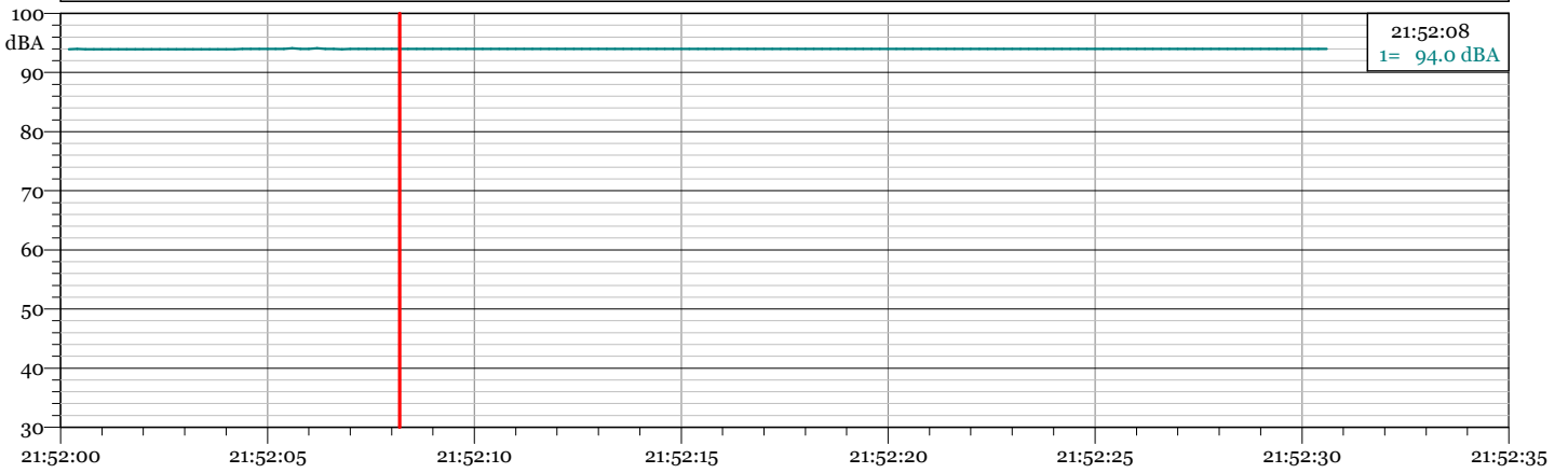
Esterne_.156 1/3 Leq Spectrum + SLM - LAeq
