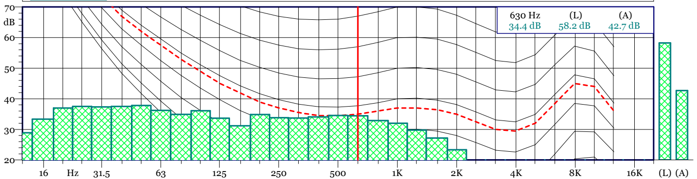
19120600.LD0 1/3 All Min Spectrum - Min
