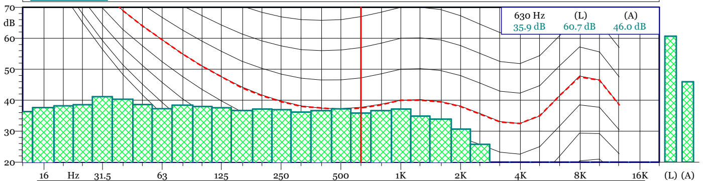
TRD 19120900.LDo 1/3 SPL Spectrum - Min
