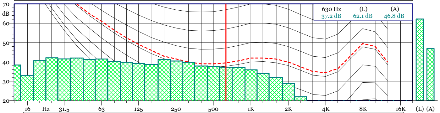
TRN 19120500.LDo 1/3 SPL Spectrum - Min
