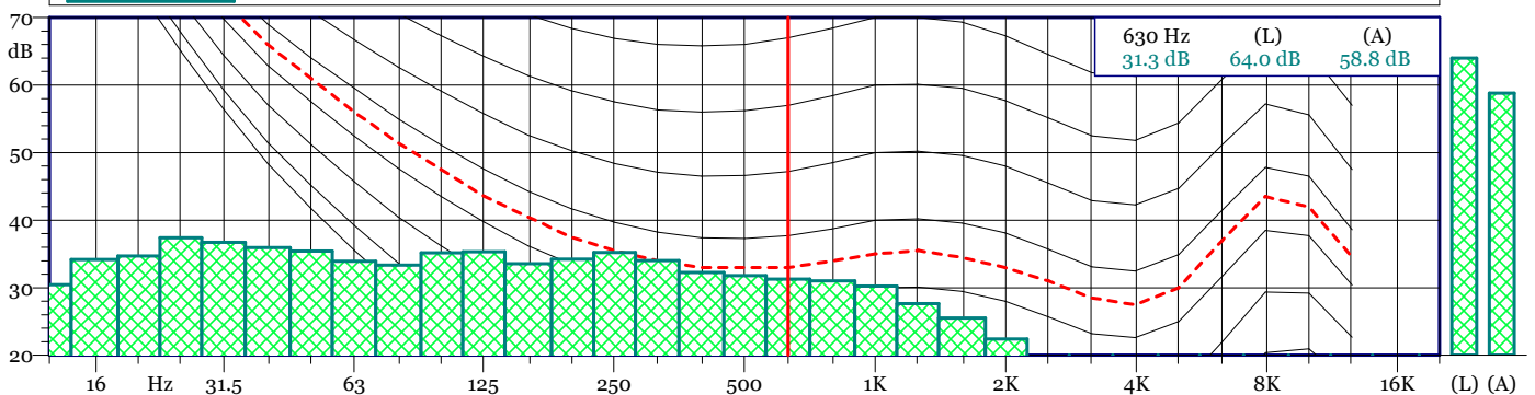
19120900.LD0 1/3 All Min Spectrum - Min
