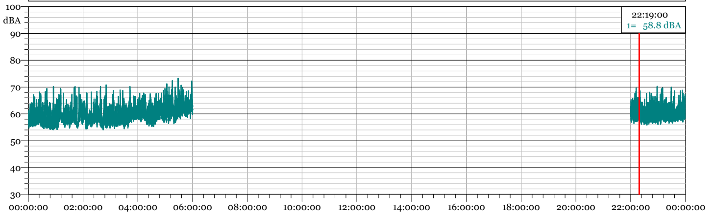
1 - TRN 19121000.LD0 - 1/3 Leq Spectrum + SLM - LAeq
