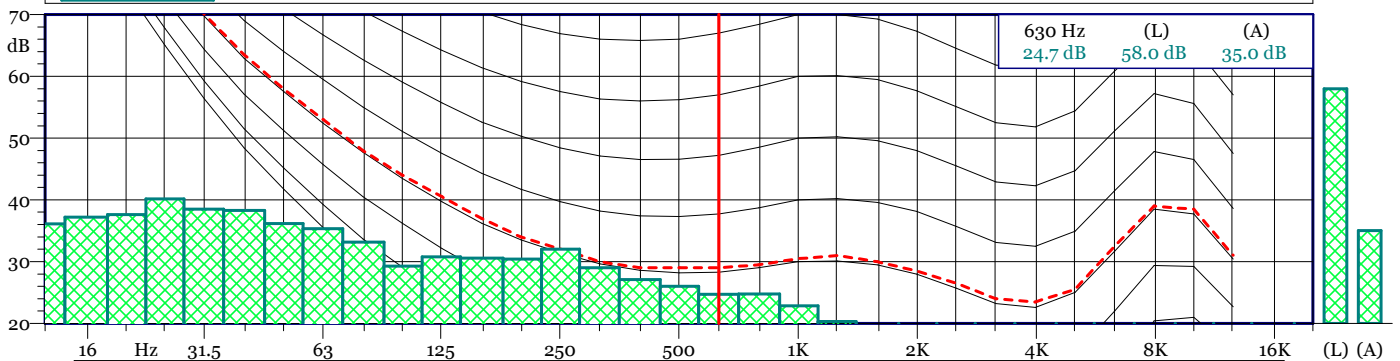
TRD 19120800.LDo 1/3 SPL Spectrum - Min
