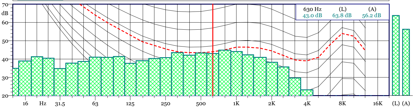
19121000.LD0 1/3 All Min Spectrum - Min
