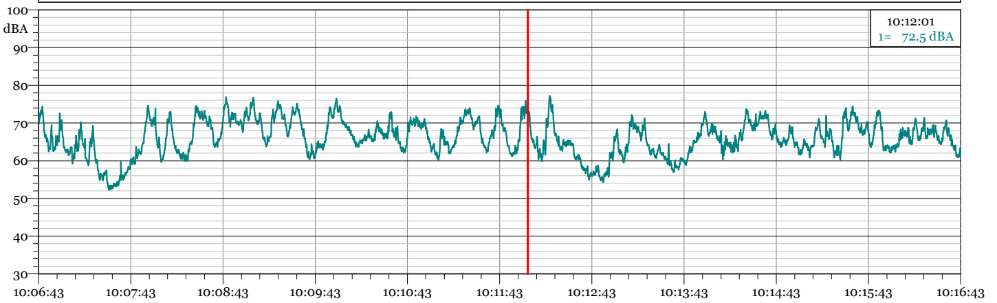
Esterne_.226 1/3 Leq Spectrum + SLM - LAeq L 90 = 60.2 dB(A) L95 = 57.1 dB(A)
