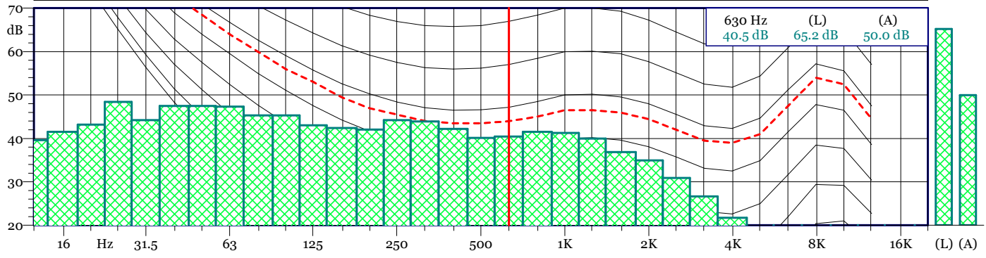
TRN 19120500.LD0 - 1/3 All Min Spectrum - Min
