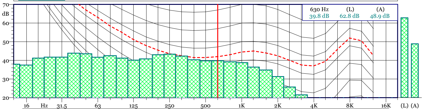
TRD 19121000.LDo 1/3 SPL Spectrum - Min
