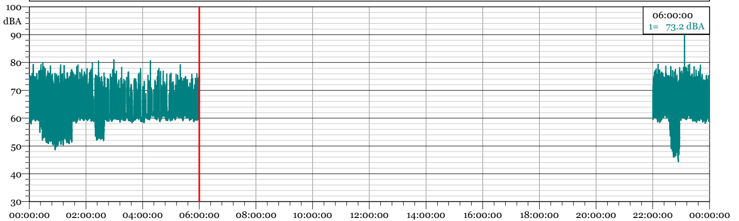
1 - TRN 19120800.LDo - 1/3 Leq Spectrum + SLM - LAeq
