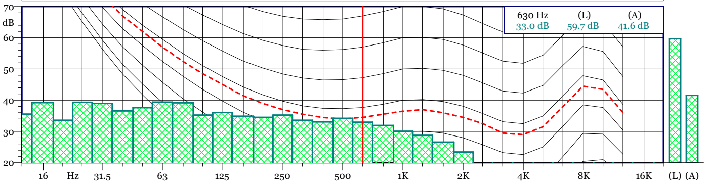
TRD 19120700.LD0 1/3 SPL Spectrum - Min
