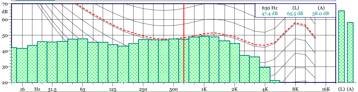
TRD 19121300.LDo 1/3 SPL Spectrum - Min
