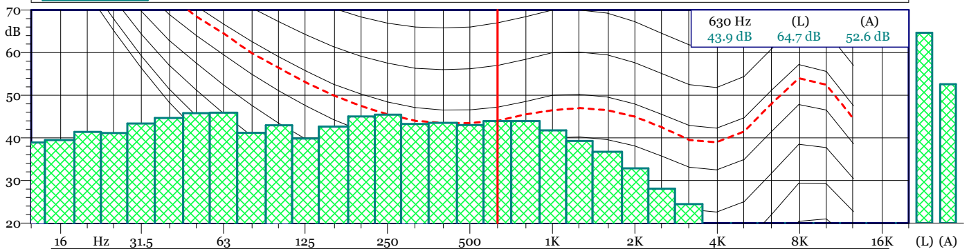
TRN 19120401.LD0 1/3 SPL Spectrum - Min
