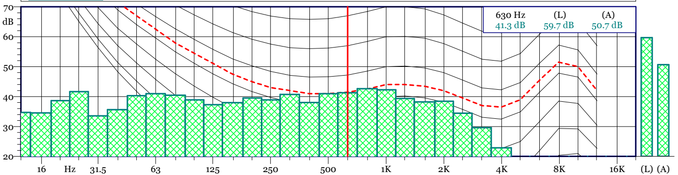
TRN 19120700.LD0 1/3 All Min Spectrum - Min
