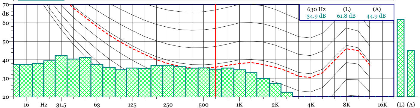
TRD 19120500.LD0 1/3 SPL Spectrum - Min
