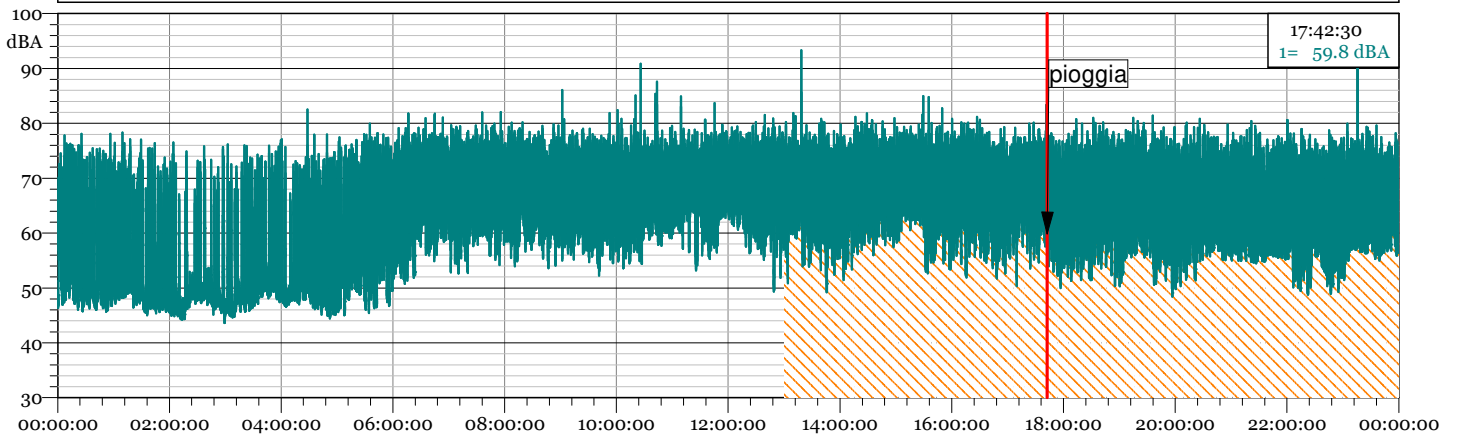
19120600.LD0 1/3 Leq Spectrum + SLM - LAeq
