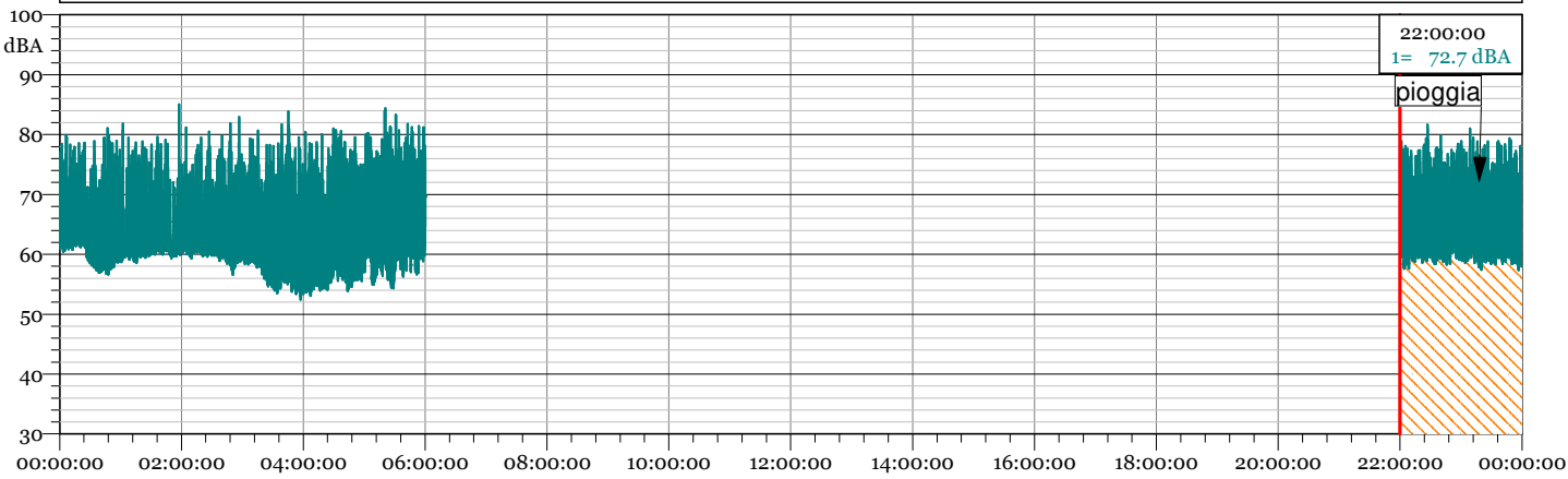
1 - TRN 19120500.LD0 - 1/3 Leq Spectrum + SLM - LAeq
