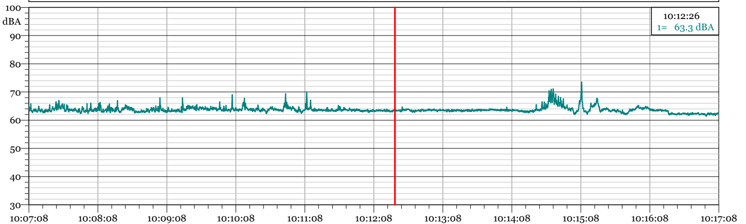
Esterne_.144 1/3 Leq Spectrum + SLM - LAeq L 90 = 62.8 dB(A) L 95 = 62.3 dB(A)
