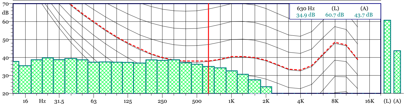
TRN 19120600.LDo 1/3 SPL Spectrum - Min
