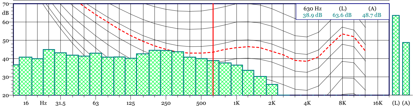
TRN 19121100.LD0 1/3 SPL Spectrum - Min
