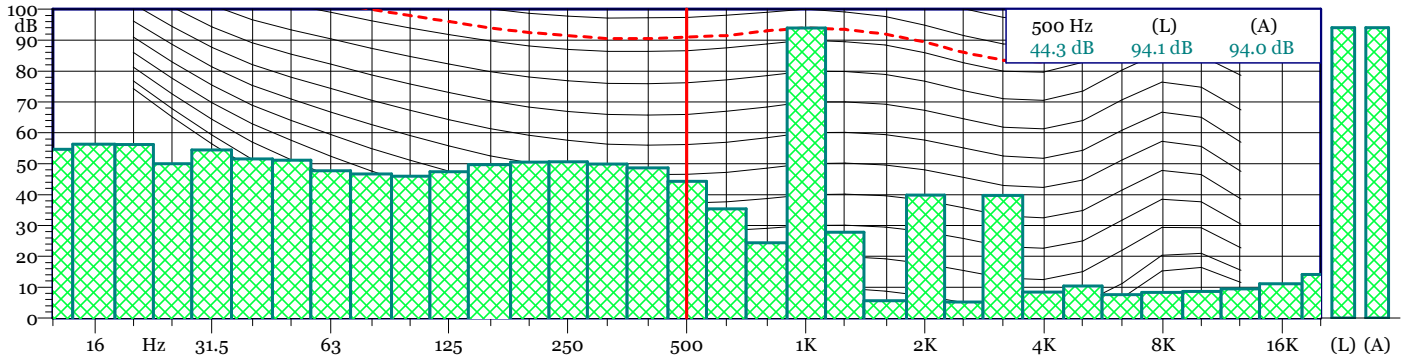
Esterne_.156 - 1/3 All Min Spectrum - Min
