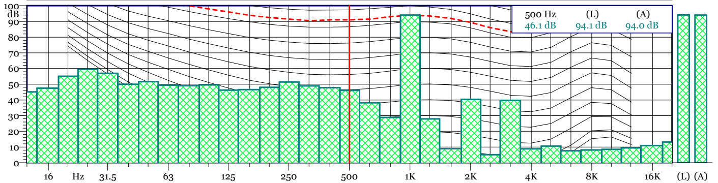
Esterne_.137 - 1/3 All Min Spectrum - Min
