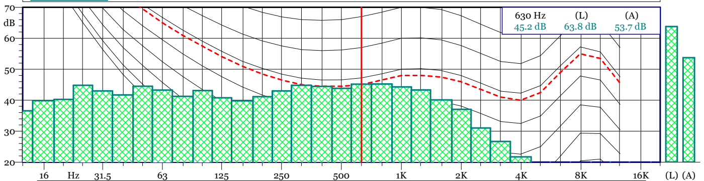
TRD 19120401.LD0 1/3 SPL Spectrum - Min
