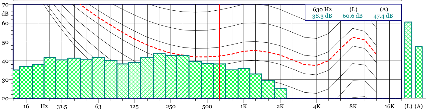
19121100.LD0 1/3 All Min Spectrum - Min
