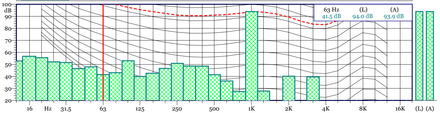
19121301.LD0 - 1/3 All Min Spectrum - Min
