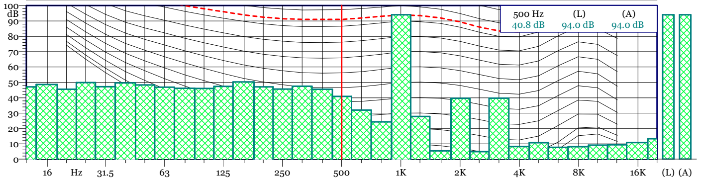
Esterne_.236 - 1/3 All Min Spectrum - Min
