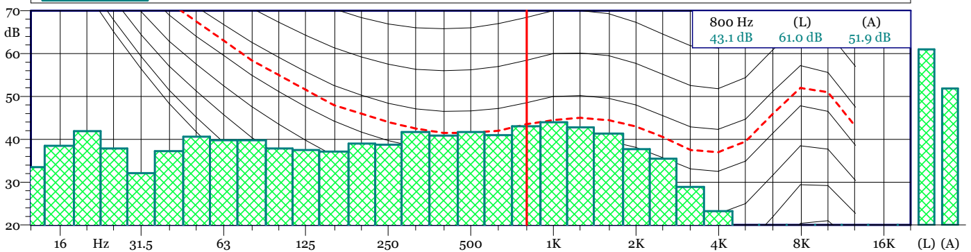
TRD 19121200.LD0 - 1/3 All Min Spectrum - Min
