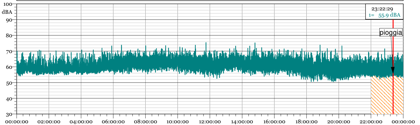
19120500.LD0 1/3 Leq Spectrum + SLM - LAeq
