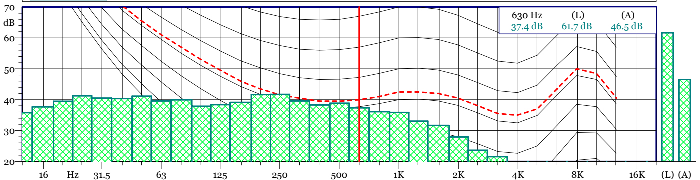
TRN 19120700.LDo 1/3 SPL Spectrum - Min
