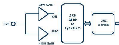
BLOCK DIAGRAM of DIGITAL HYDROPHONE
