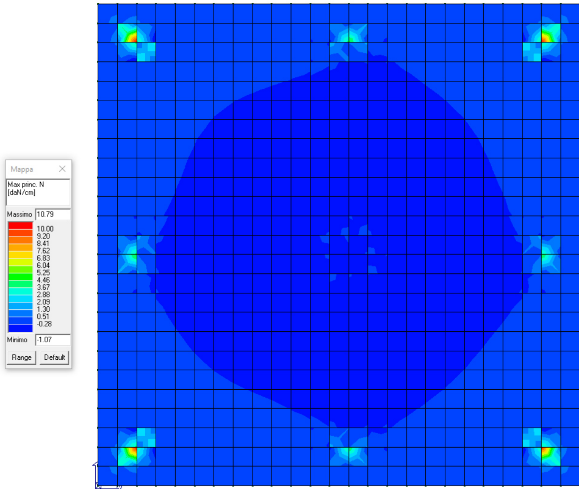
Figura 5 – Von Mises: Max princ. N (daN/cm)
