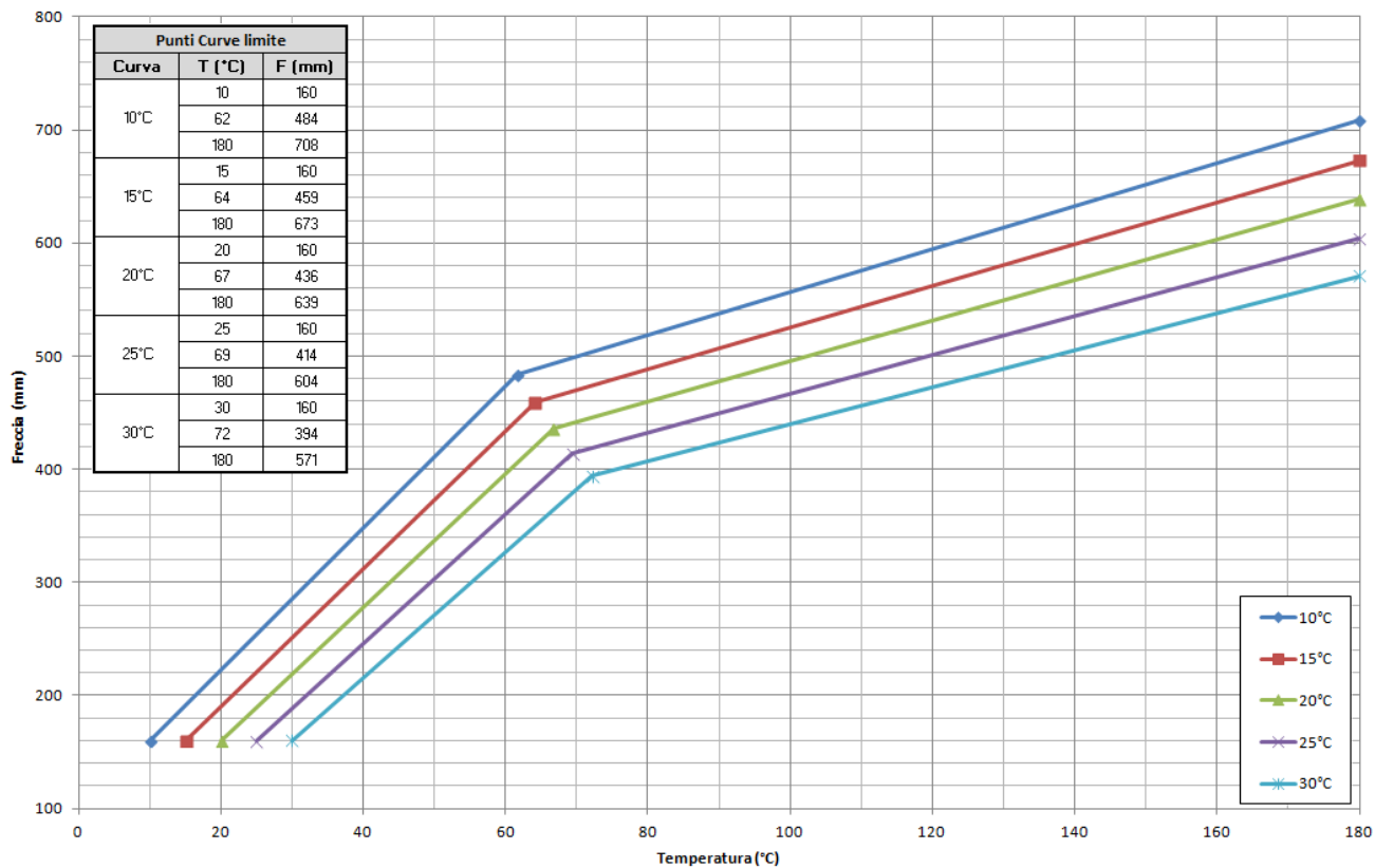
Figura 2 – Curve limite
