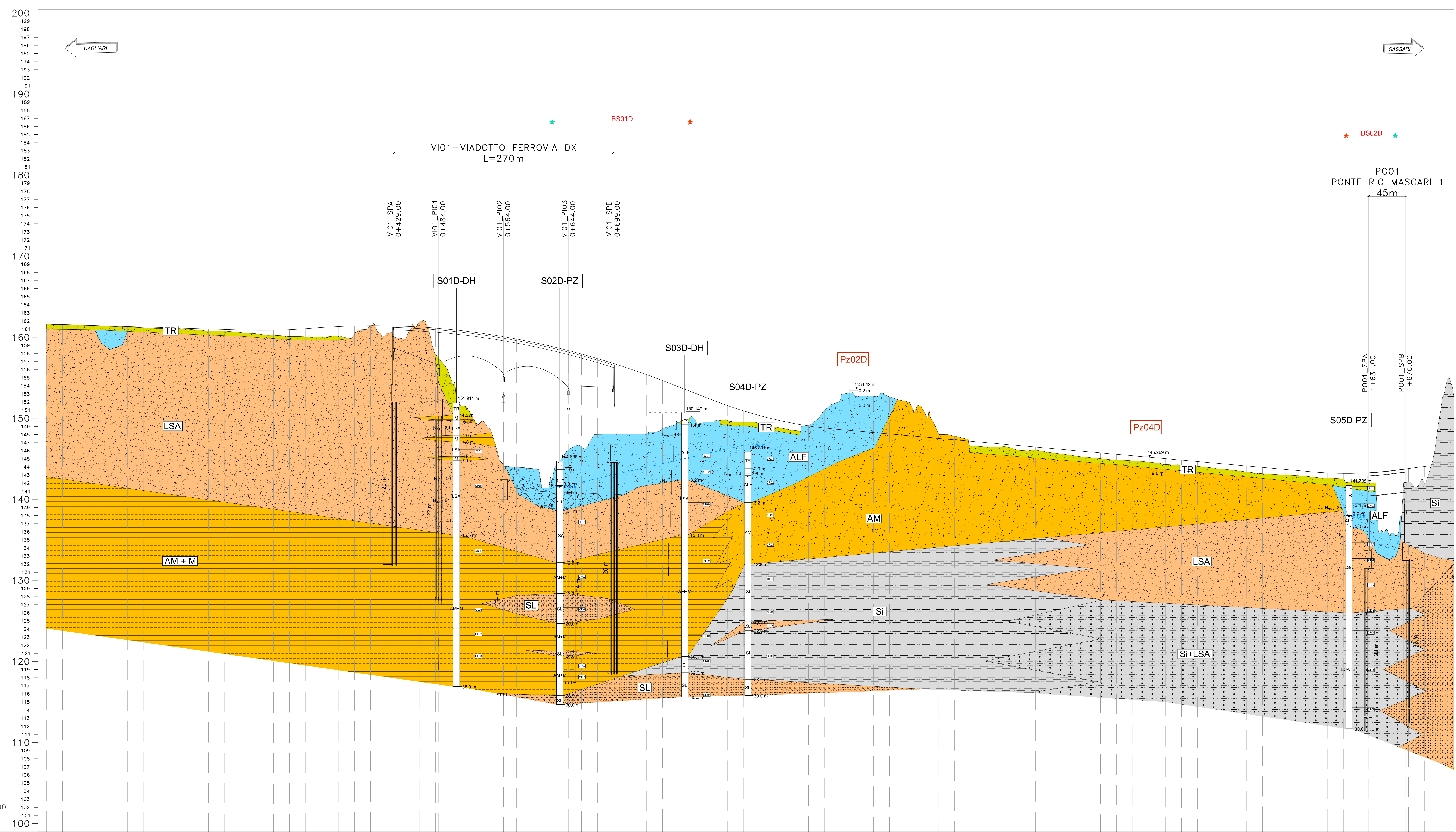
Profilo AP_DX Km = 0+000.00 - 6+711.00 Scala: 2000:200 Q.Rif.: 99.00
