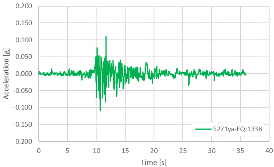
Figura 11 – Accelerogramma naturale: Waveform 5271ya – Eartquake 1338
