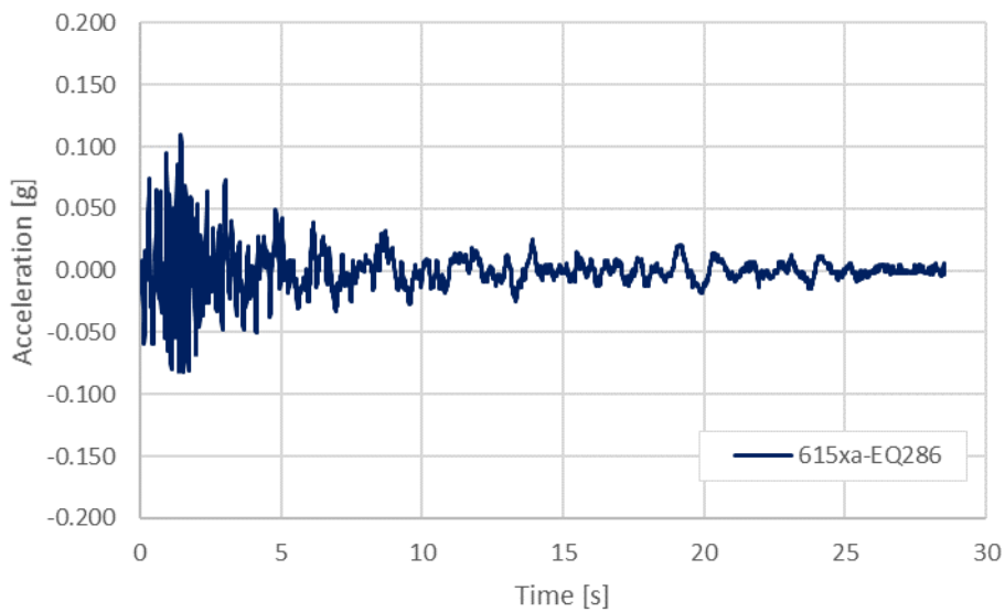
Figura 9 – Accelerogramma naturale: Waveform 615xa – Eartquake 286
