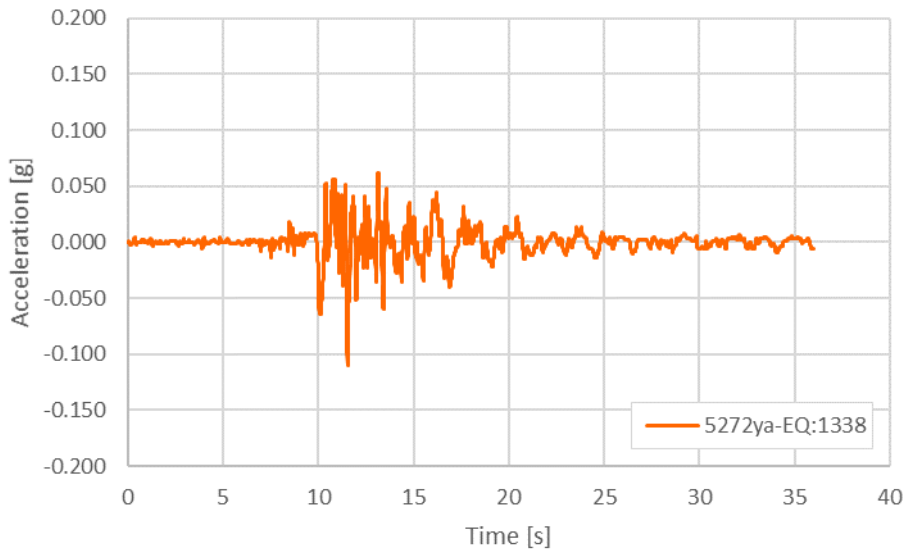
Figura 12 – Accelerogramma naturale: Waveform 5272xa – Eartquake 1338
