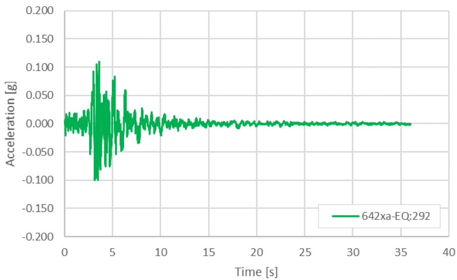
Figura 11 – Accelerogramma naturale: Waveform 642xa – Earthquake 292
