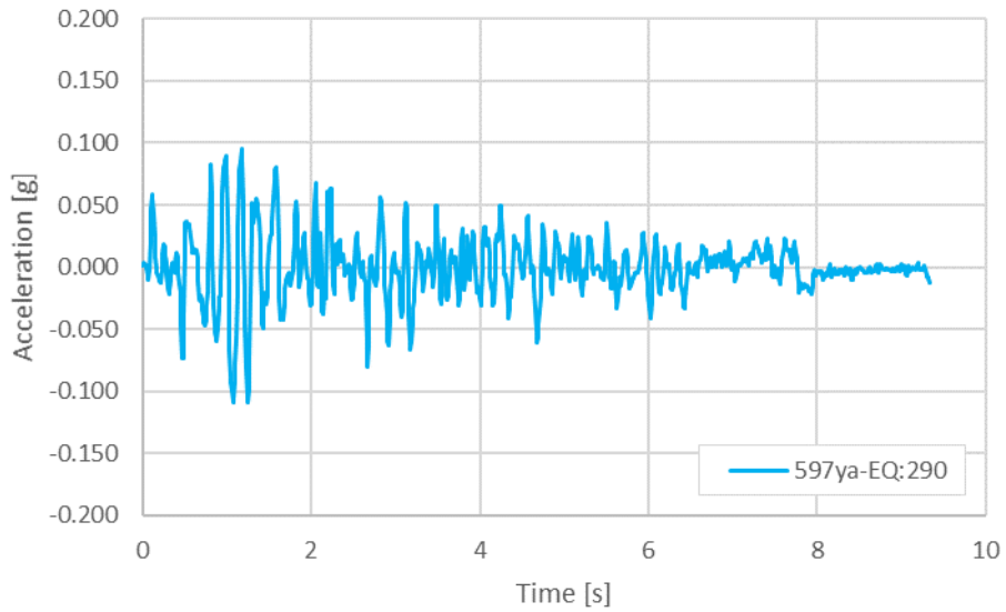
Figura 10 – Accelerogramma naturale: Waveform 597ya – Earthquake 290
