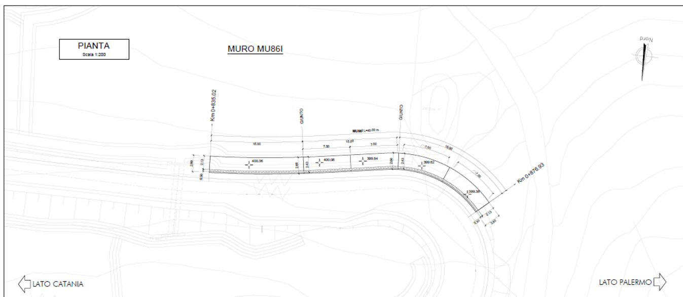
Figura 1-1 –Pianta MU861.
