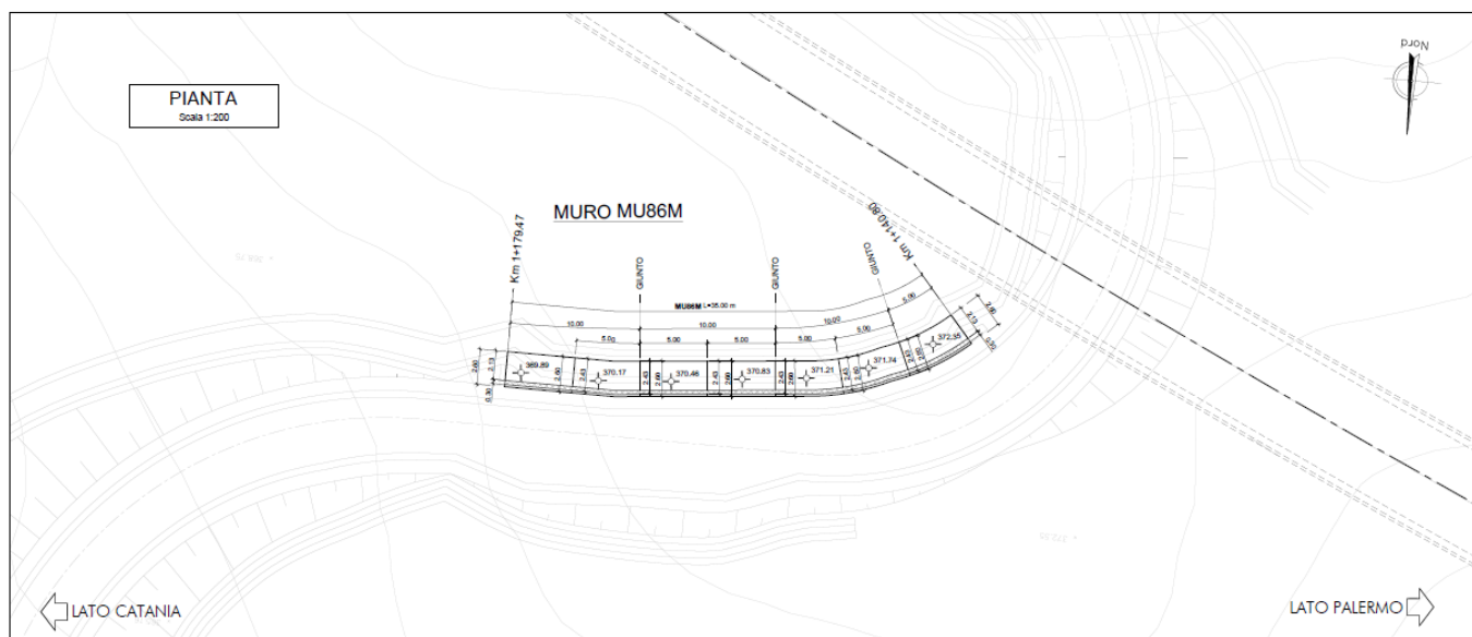
Figura 1-1 –Pianta MU86M.
