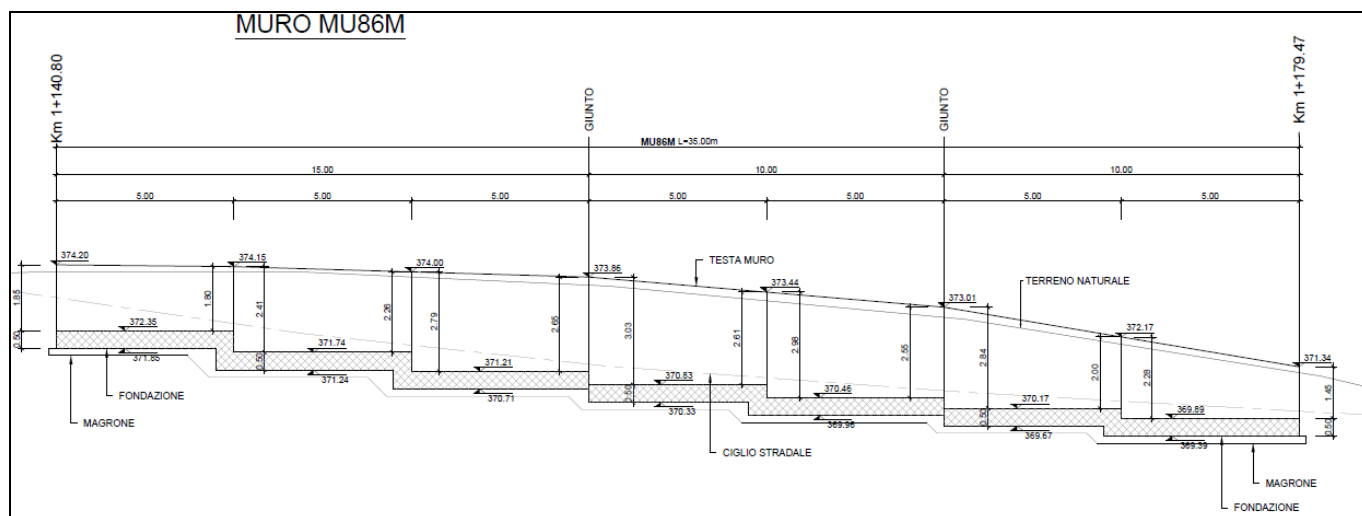
Figura 1-2 –Profilo MU86M.
