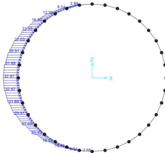
Frame Distributed Loads (spinta_EQ+X)
