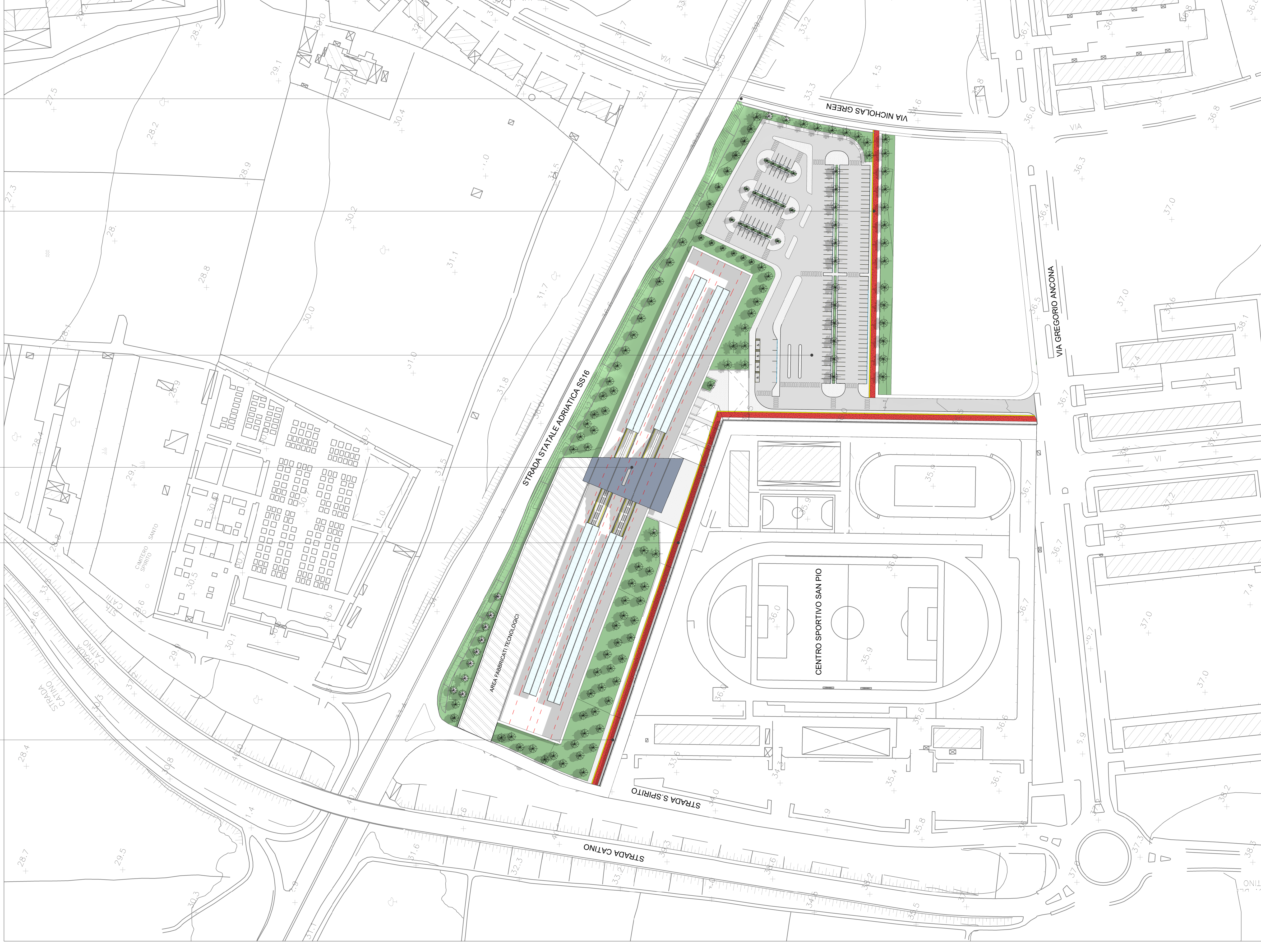
Planimetria Post Operam Scala 1:1000
