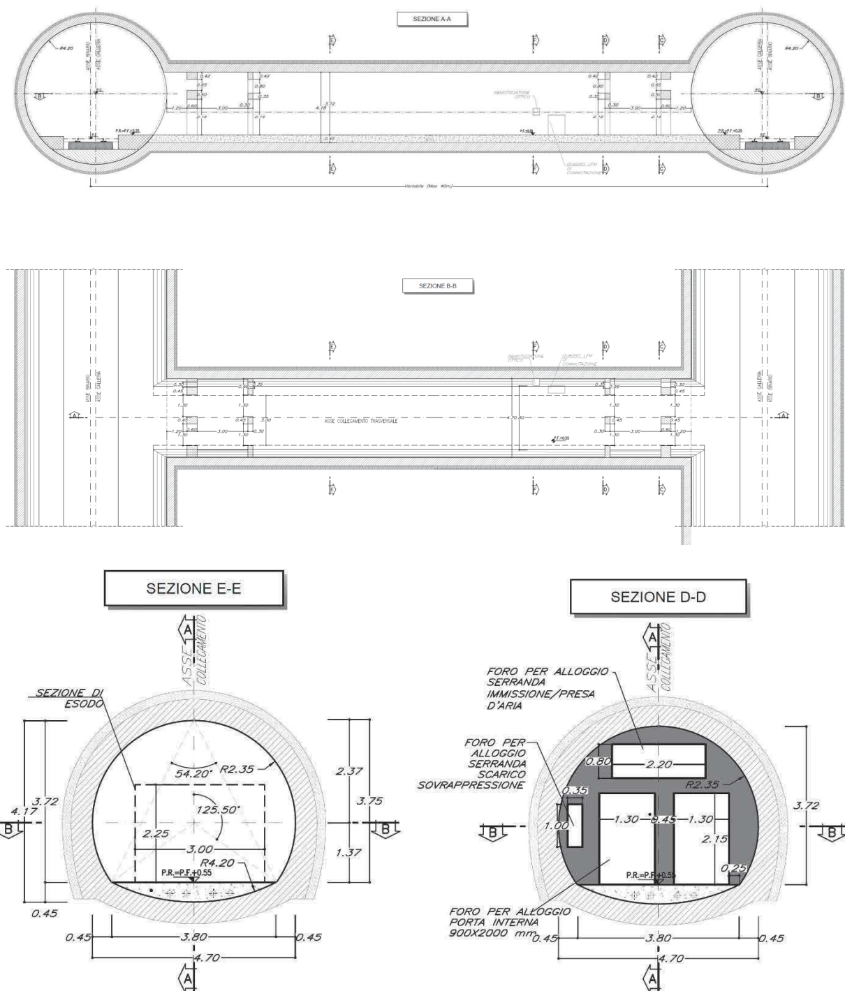
Figura 3. By-Pass trasversali
