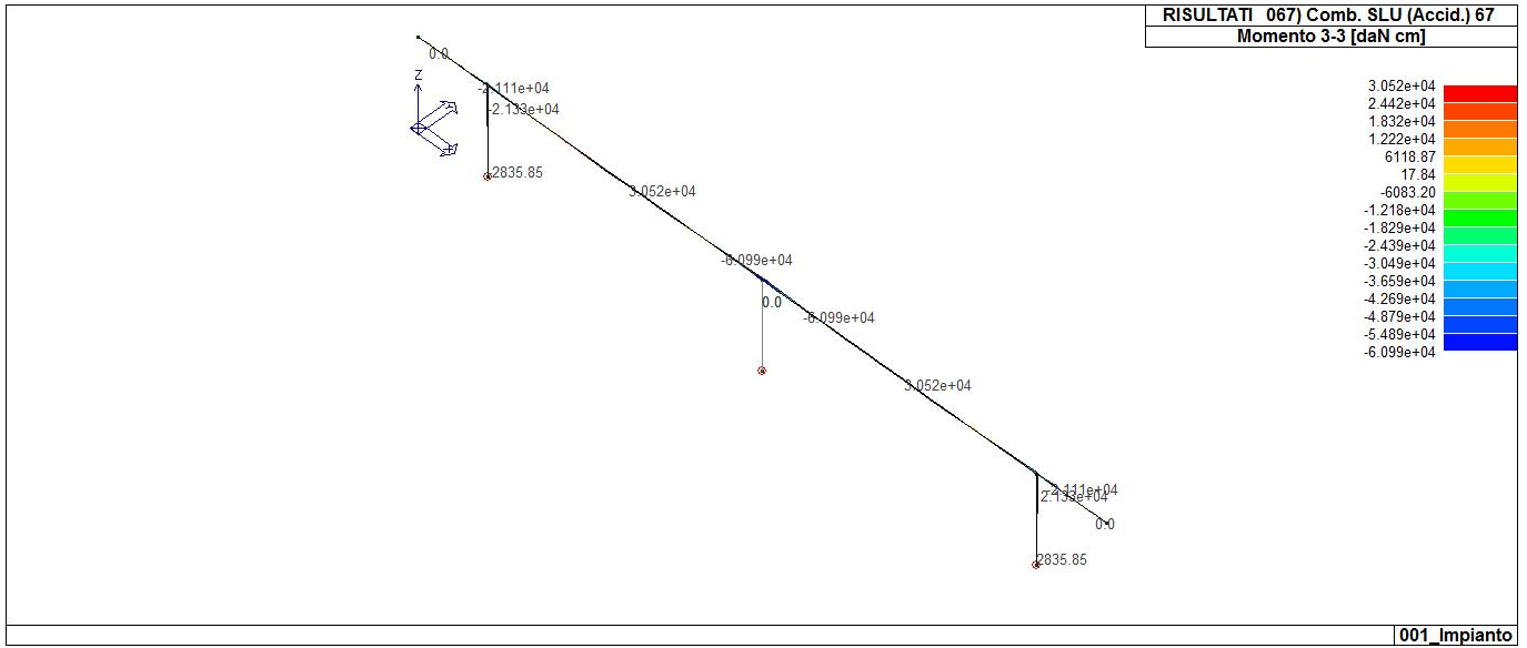
43_RIS_M3_067_Comb. SLU (Accid.) 67
