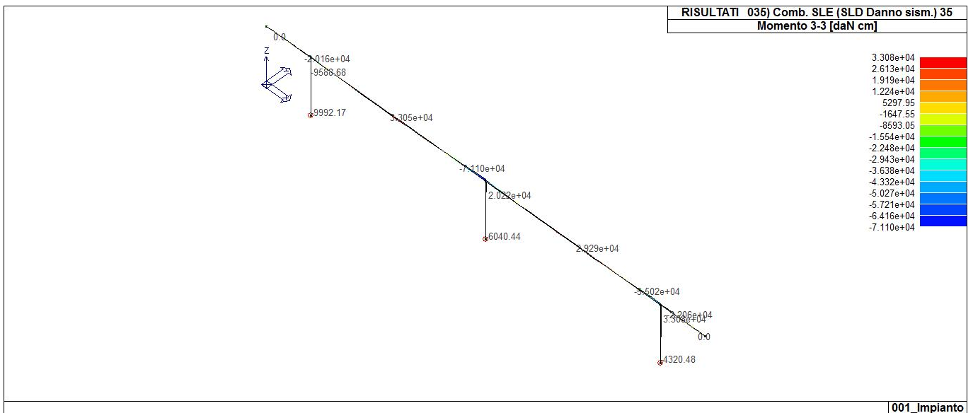
43_RIS_M3_035_Comb. SLE (SLD Danno sism.) 35
