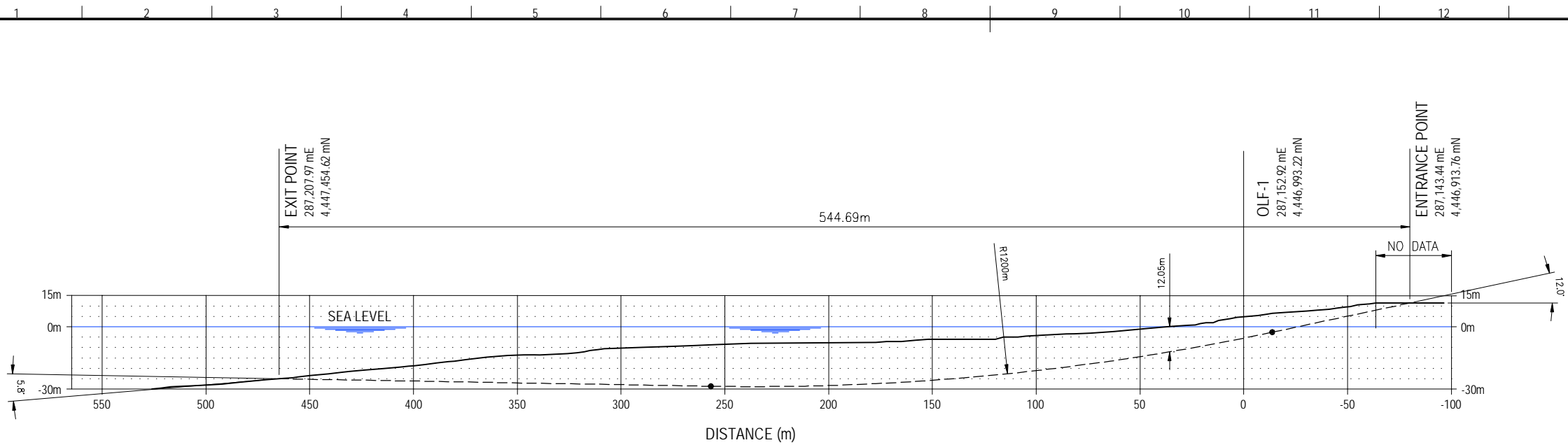
LONGITUDINAL PROFILE ALONG HDD TRAJECTORY (NO EXAGGERATION)
