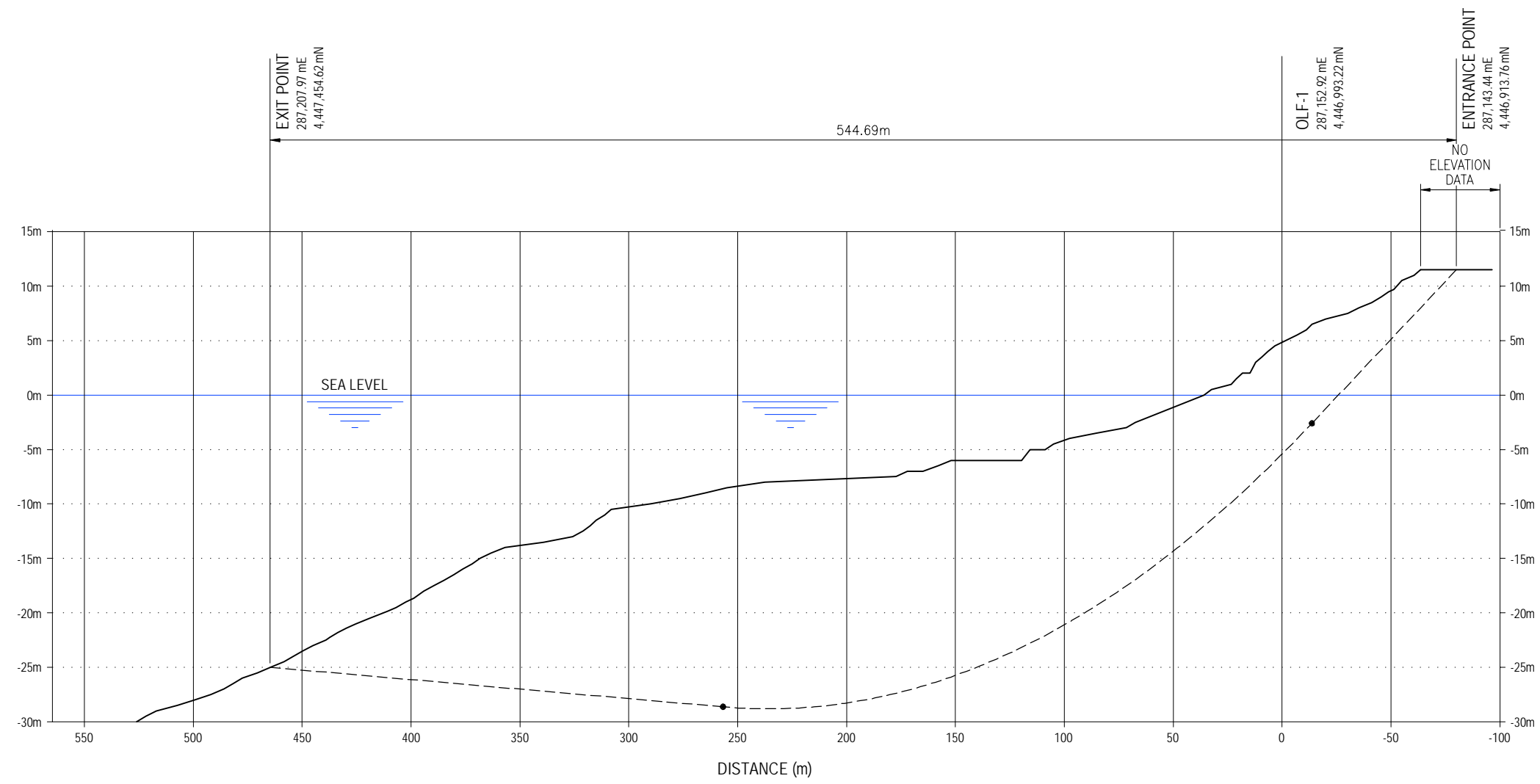
LONGITUDINAL PROFILE ALONG HDD TRAJECTORY (VERTICAL EXAGGERATION = 5x)
