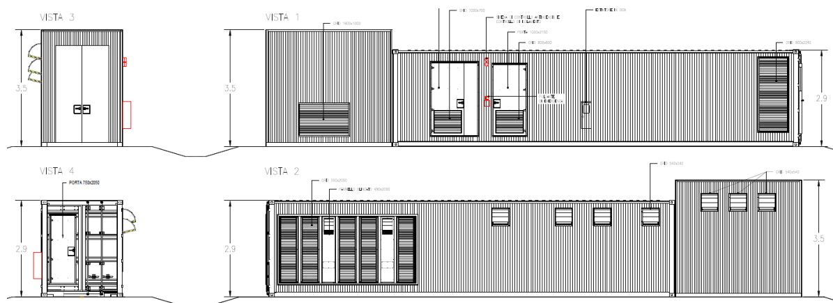
Figura 2.9: Tipologico Power Station
