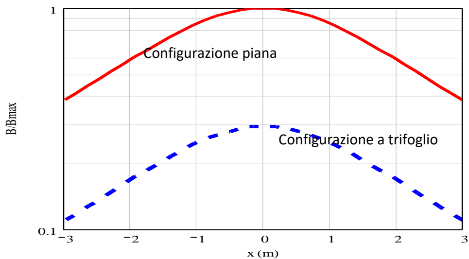
Figura 18 - Lateral profile of the magnetic flux density (in p.u.) generated by: the flat configuration (continuous line) or the trefoil configuration (broken line).
