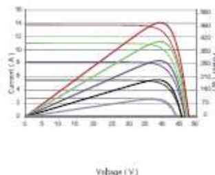
Current-Voltage & Power-Voltage Curves (515W)
