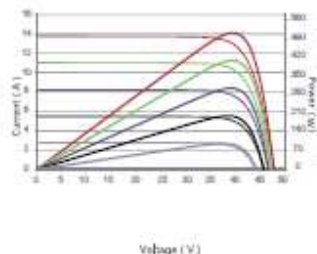
Current-Voltage & Power-Voltage Curves (515W)
