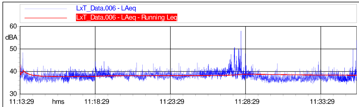
TIME HISTORY
