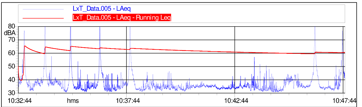
TIME HISTORY
