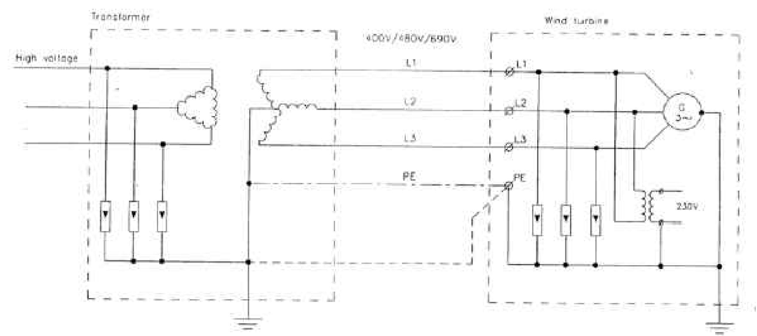
TN-system : IEC 364 312.2.1. (Electrical installation)
