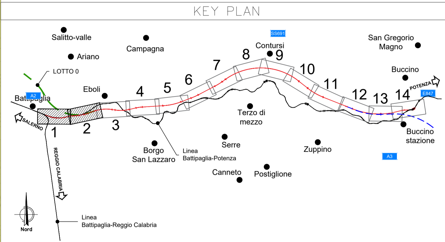
LAYOUT 1
