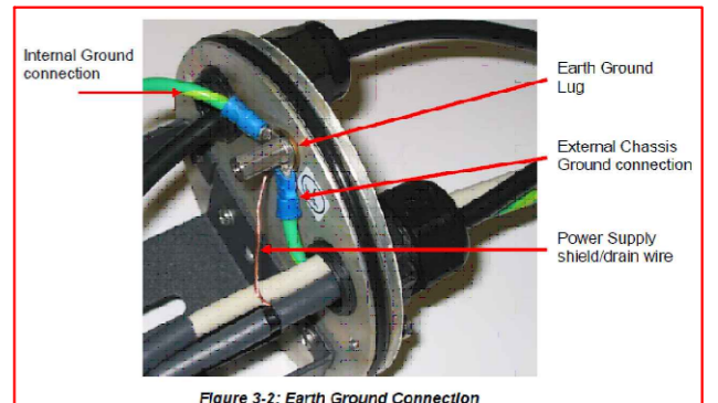
Figure 3-2: Earth Ground Connection
