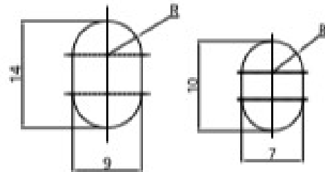
Mounting Hole
