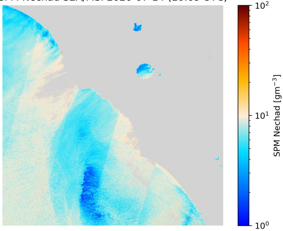
SPM Nechad S2A/MSI 2020-07-14 (10:09 UTC)
