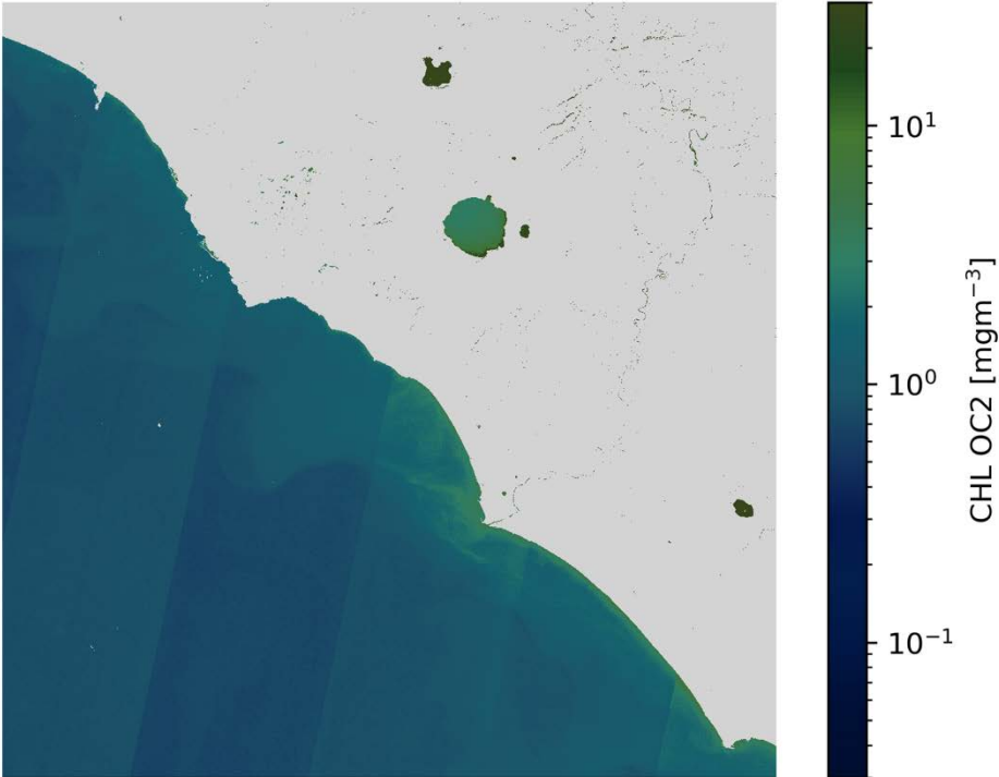
CHL OC2 S2A/MSI 2020-12-21 (10:09 UTC)
