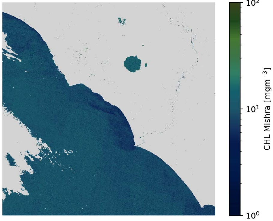
CHL Mishra S2B/MSI 2020-12-16 (10:09 UTC)
