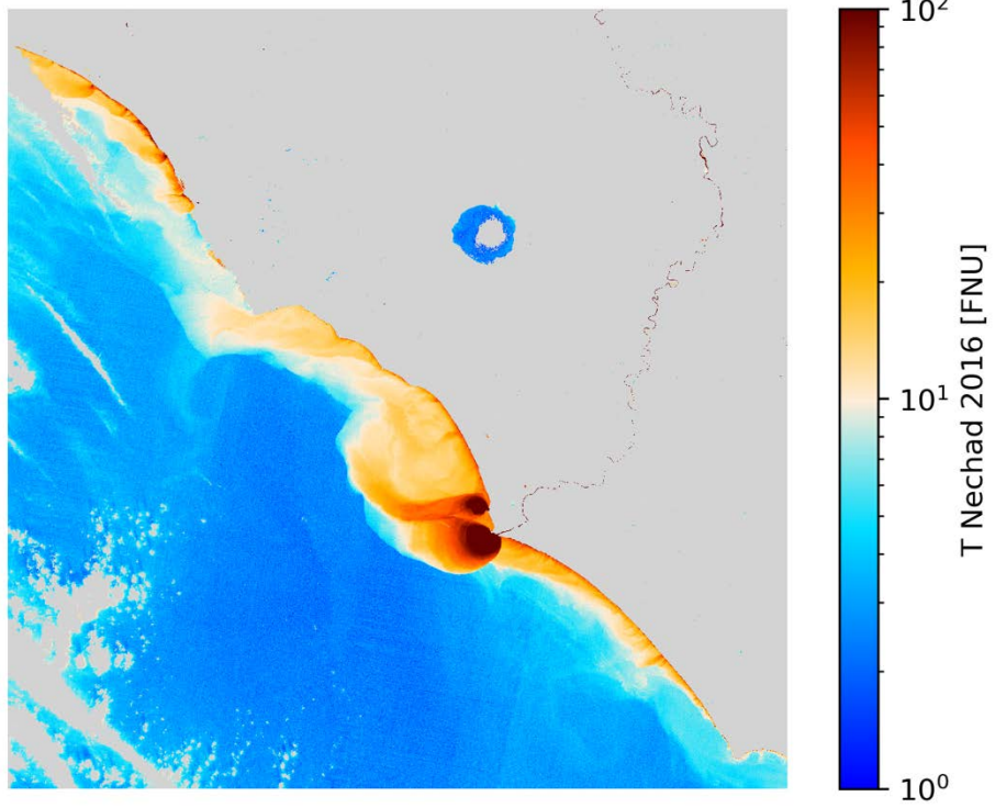
T Nechad 2016 S2A/MSI 2020-12-11 (10:09 UTC)
