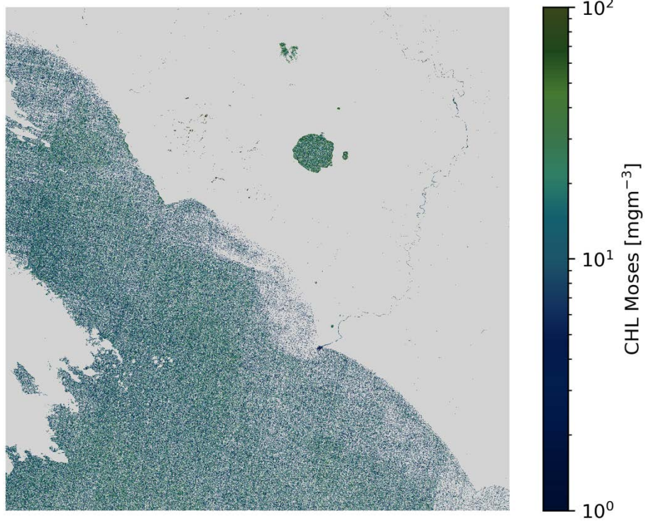
CHL Moses S2B/MSI 2020-12-16 (10:09 UTC)
