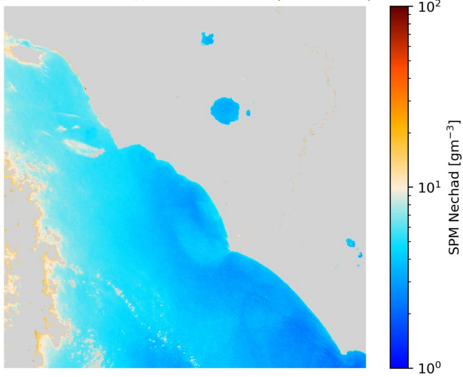
SPM Nechad S2B/MSI 2020-09-07 (10:09 UTC)
