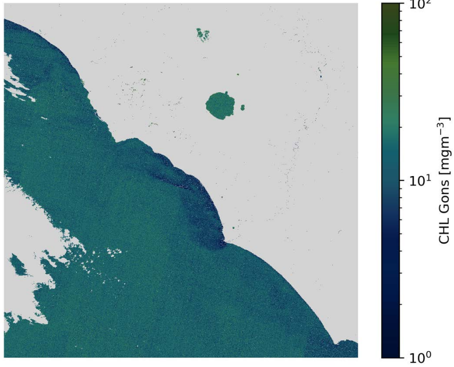
CHL Gons S2B/MSI 2020-12-16 (10:09 UTC)
