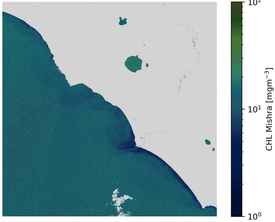
CHL Mishra S2A/MSI 2020-04-15 (10:09 UTC)
