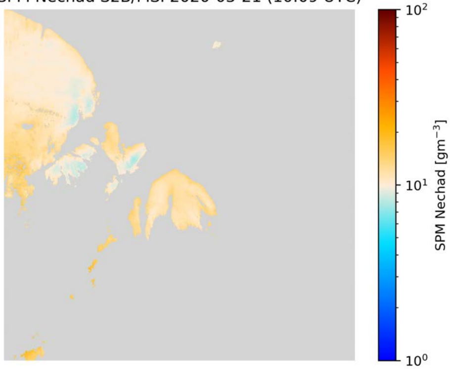
SPM Nechad S2B/MSI 2020-03-21 (10:09 UTC)
