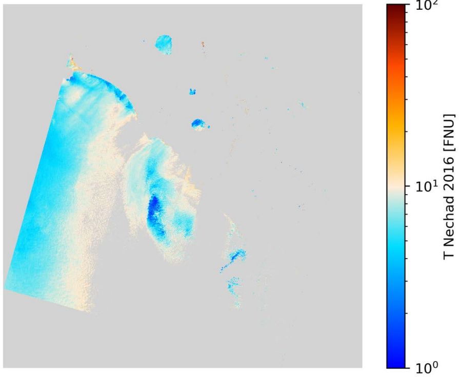
T Nechad 2016 L8/OLI 2020-07-14 (09:53 UTC)
