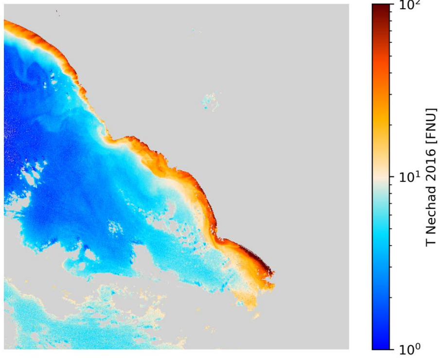
T Nechad 2016 S2A/MSI 2020-03-06 (10:09 UTC)
