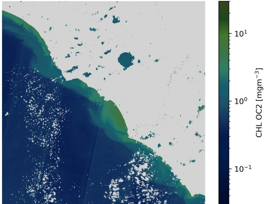
CHL OC2 S2B/MSI 2020-10-17 (10:09 UTC)
