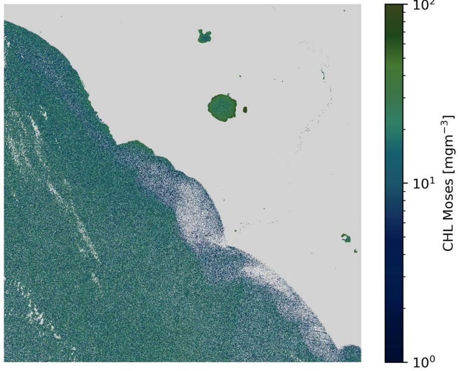
CHL Moses S2A/MSI 2020-04-25 (10:09 UTC)
