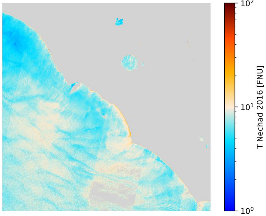
T Nechad 2016 S2B/MSI 2020-08-08 (10:09 UTC)
