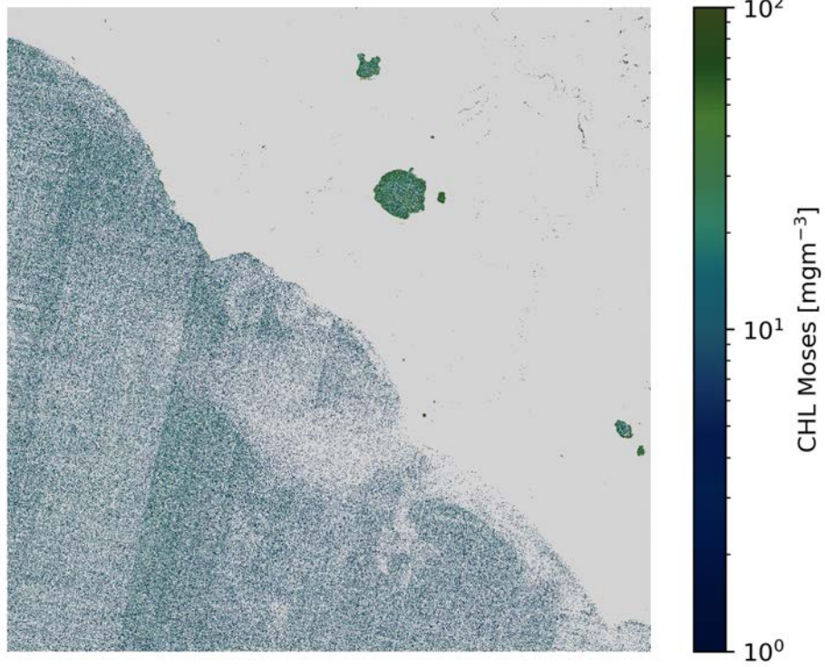
CHL Moses S2B/MSI 2020-11-06 (10:09 UTC)
