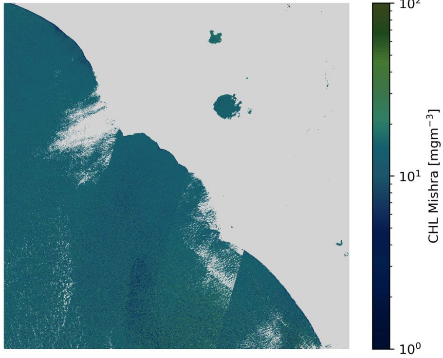
CHL Mishra S2A/MSI 2020-07-14 (10:09 UTC)
