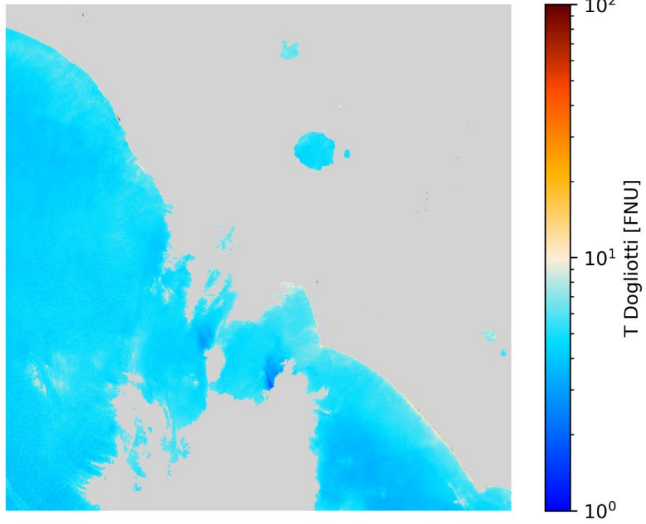
T Dogliotti S2A/MSI 2020-04-05 (10:09 UTC)
