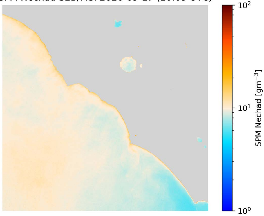
SPM Nechad S2B/MSI 2020-09-17 (10:09 UTC)
