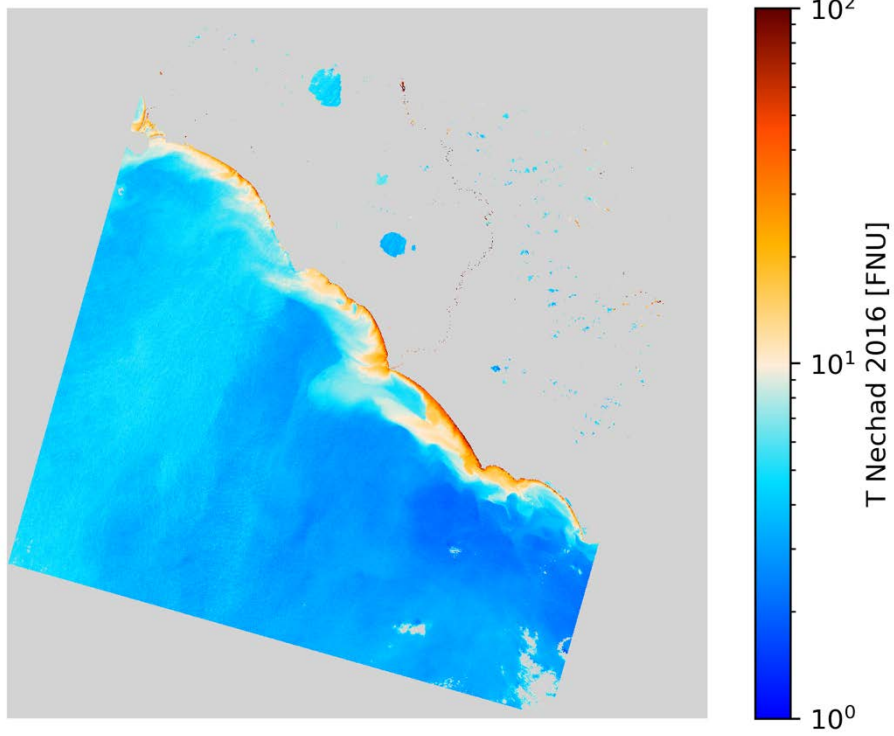
T Nechad 2016 L8/OLI 2020-03-08 (09:53 UTC)
