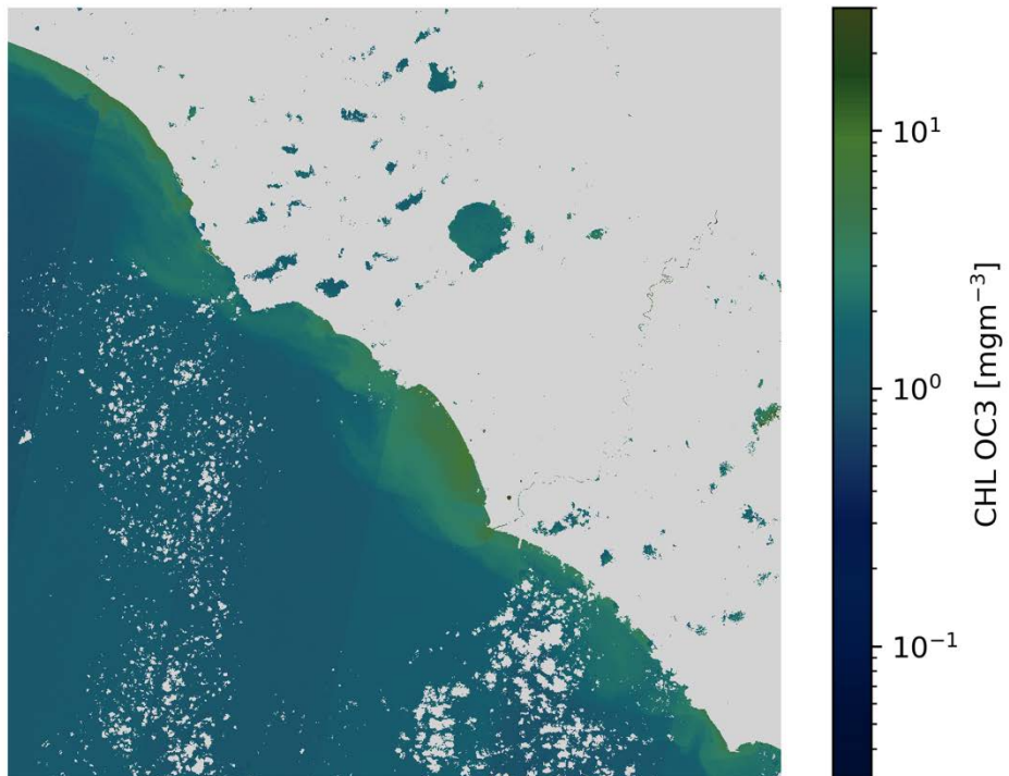
CHL OC3 S2B/MSI 2020-10-17 (10:09 UTC)
