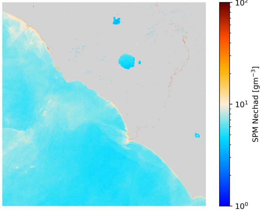
SPM Nechad S2A/MSI 2020-12-21 (10:09 UTC)
