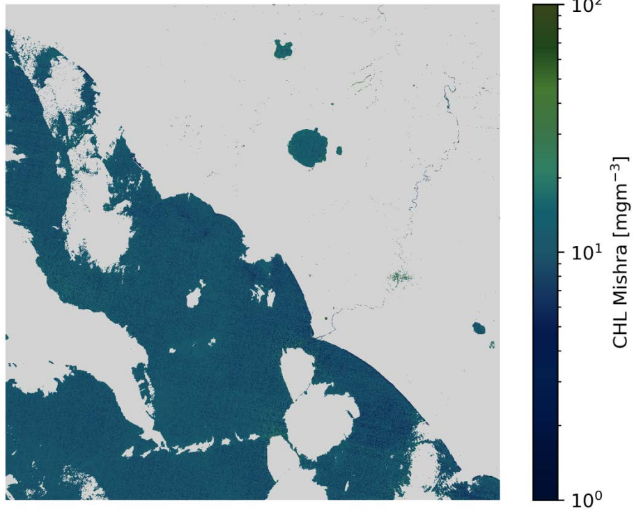
CHL Mishra S2B/MSI 2020-11-26 (10:09 UTC)
