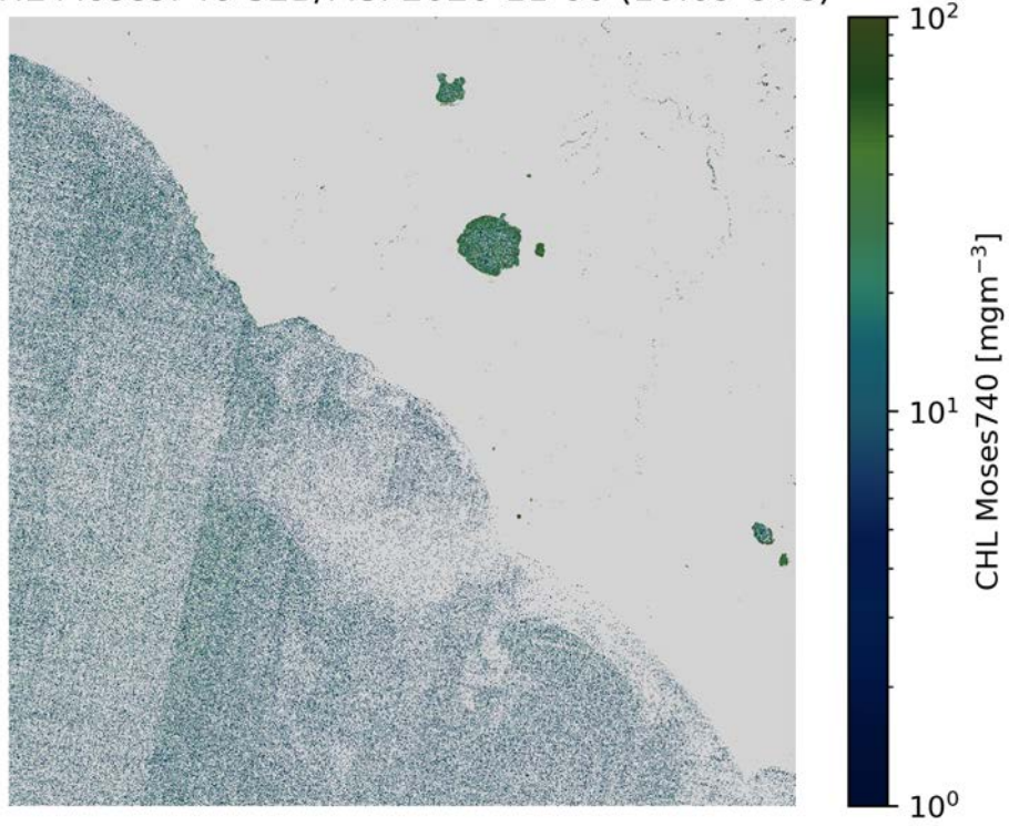
CHL Moses740 S2B/MSI 2020-11-06 (10:09 UTC)
