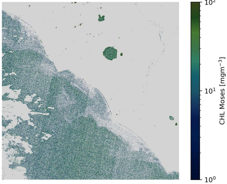
CHL Moses S2A/MSI 2020-10-22 (10:09 UTC)
