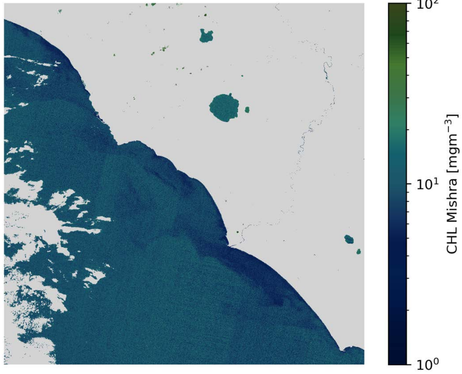
CHL Mishra S2A/MSI 2020-10-22 (10:09 UTC)
