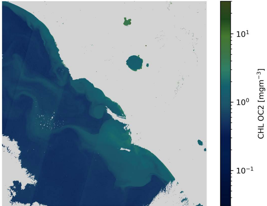
CHL OC2 S2A/MSI 2020-11-01 (10:09 UTC)
