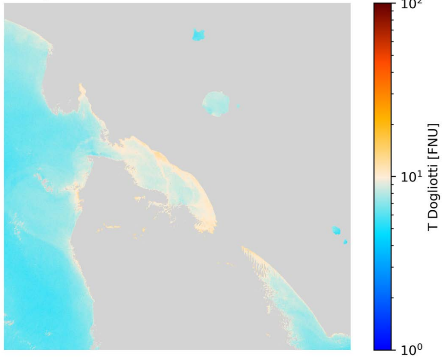
T Dogliotti S2A/MSI 2020-11-11 (10:09 UTC)
