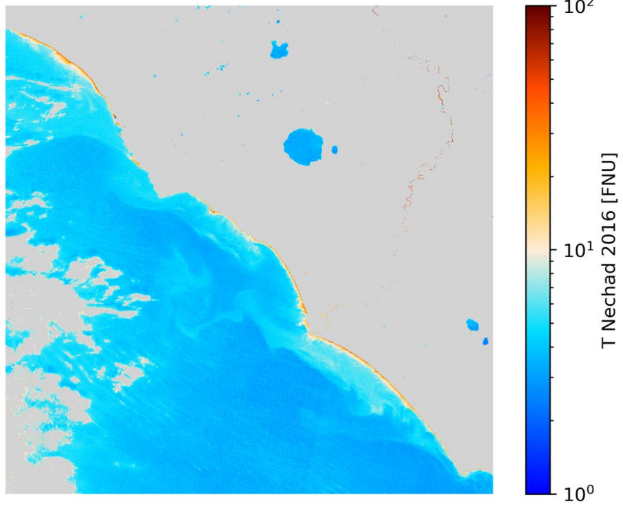
T Nechad 2016 S2A/MSI 2020-10-22 (10:09 UTC)
