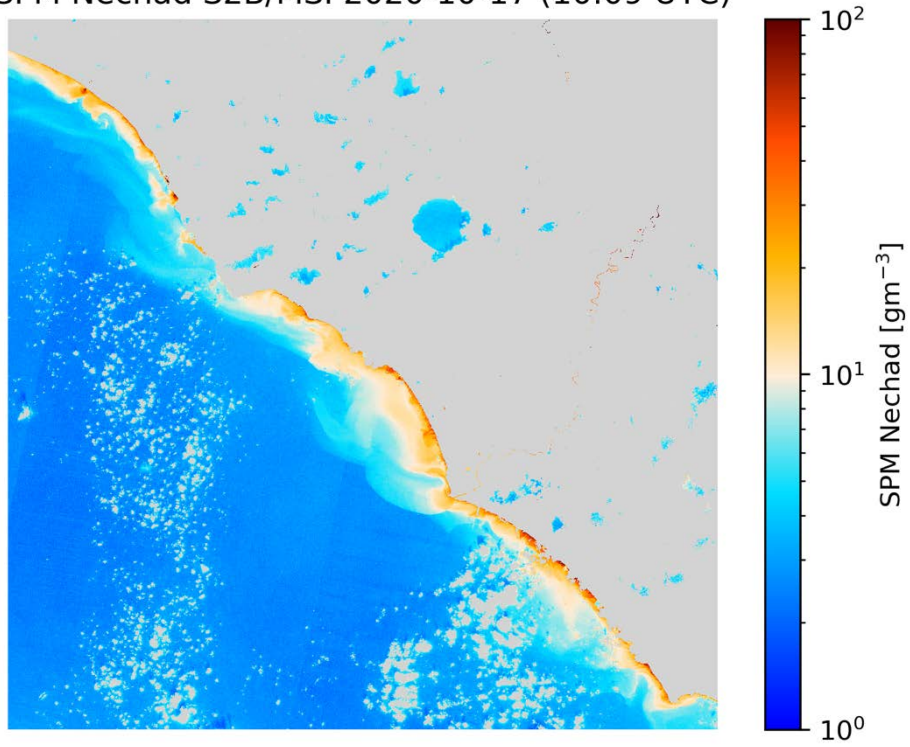
SPM Nechad S2B/MSI 2020-10-17 (10:09 UTC)
