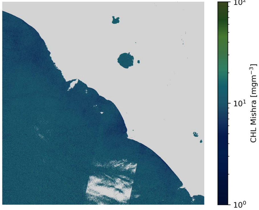
CHL Mishra S2B/MSI 2020-08-08 (10:09 UTC)
