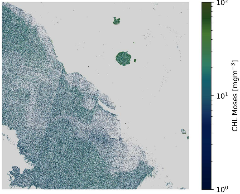
CHL Moses S2A/MSI 2020-11-01 (10:09 UTC)
