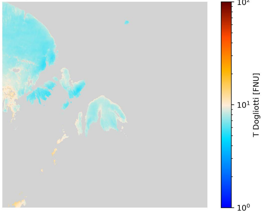
T Dogliotti S2B/MSI 2020-03-21 (10:09 UTC)
