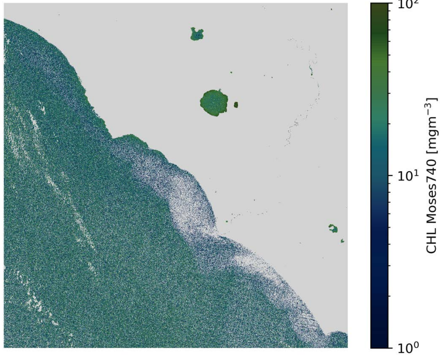
CHL Moses740 S2A/MSI 2020-04-25 (10:09 UTC)
