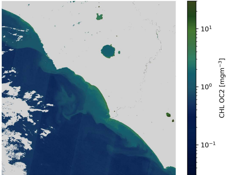
CHL OC2 S2A/MSI 2020-10-22 (10:09 UTC)
