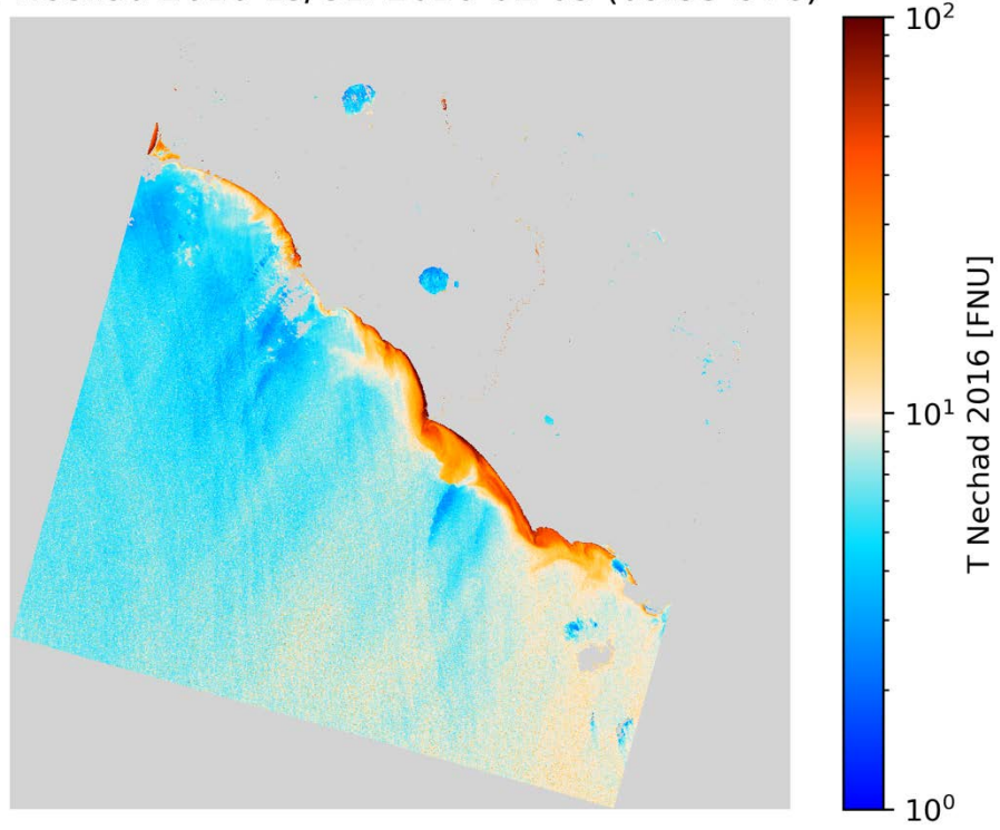
T Nechad 2016 L8/OLI 2020-02-05 (09:53 UTC)
