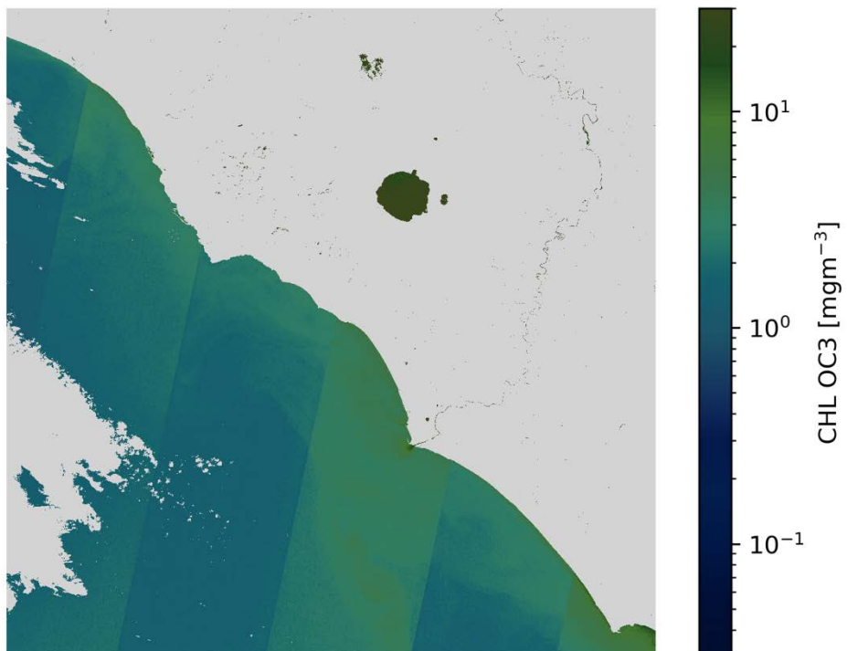
CHL OC3 S2B/MSI 2020-12-16 (10:09 UTC)
