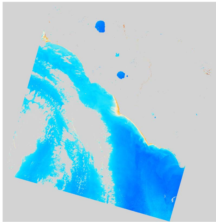
SPM Nechad L8/OLI 2020-02-21 (09:53 UTC)
