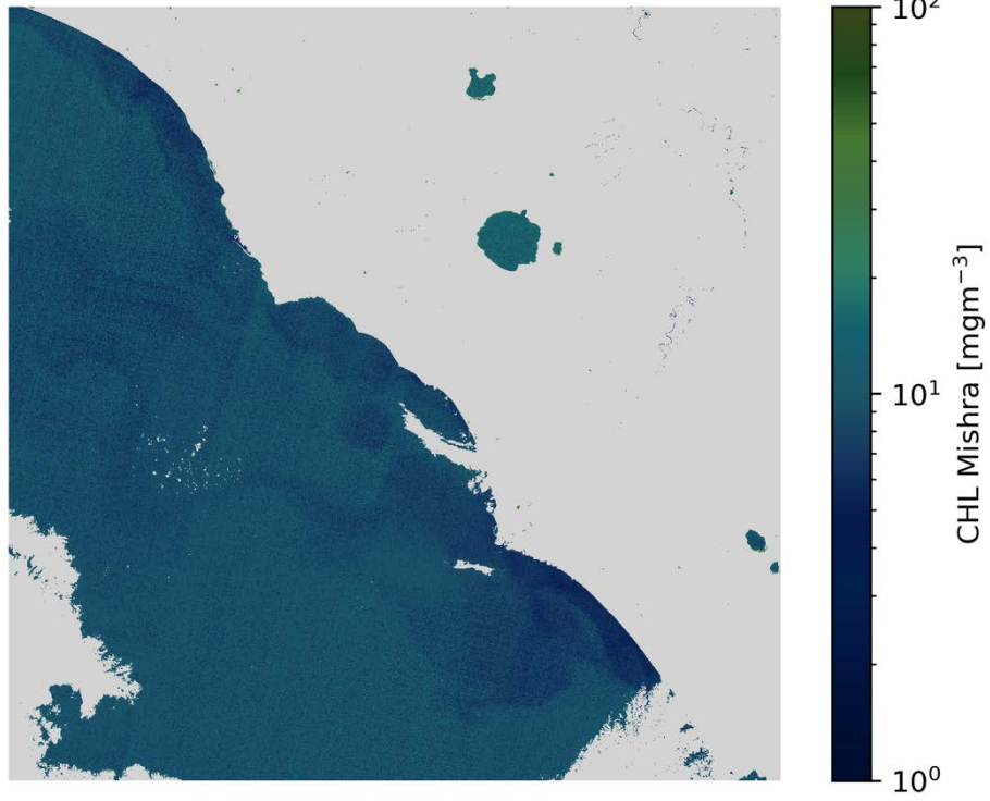
CHL Mishra S2A/MSI 2020-11-01 (10:09 UTC)
