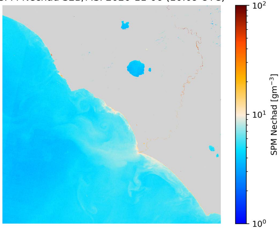
SPM Nechad S2B/MSI 2020-11-06 (10:09 UTC)
