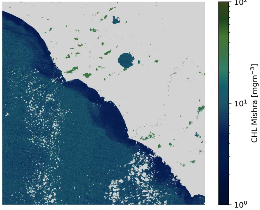
CHL Mishra S2B/MSI 2020-10-17 (10:09 UTC)
