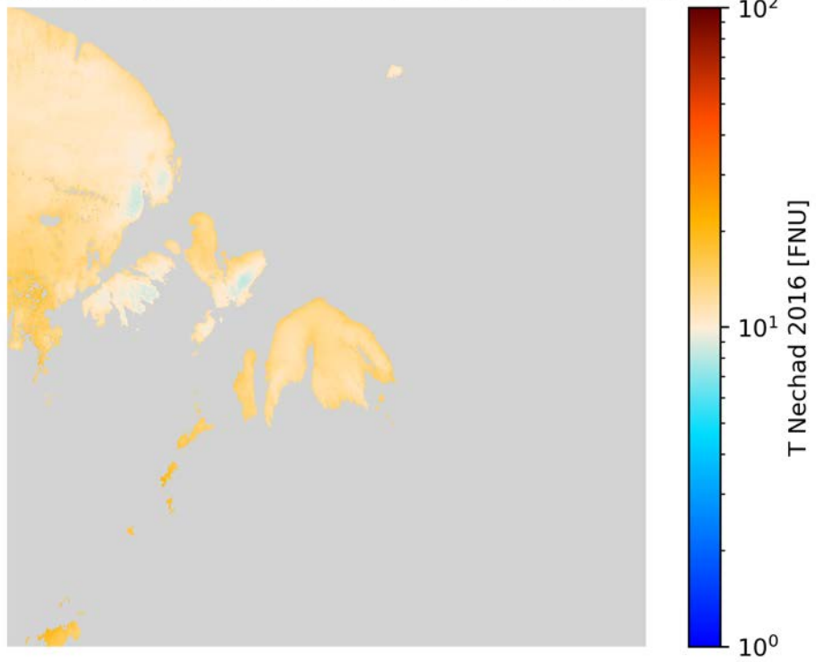
T Nechad 2016 S2B/MSI 2020-03-21 (10:09 UTC)
