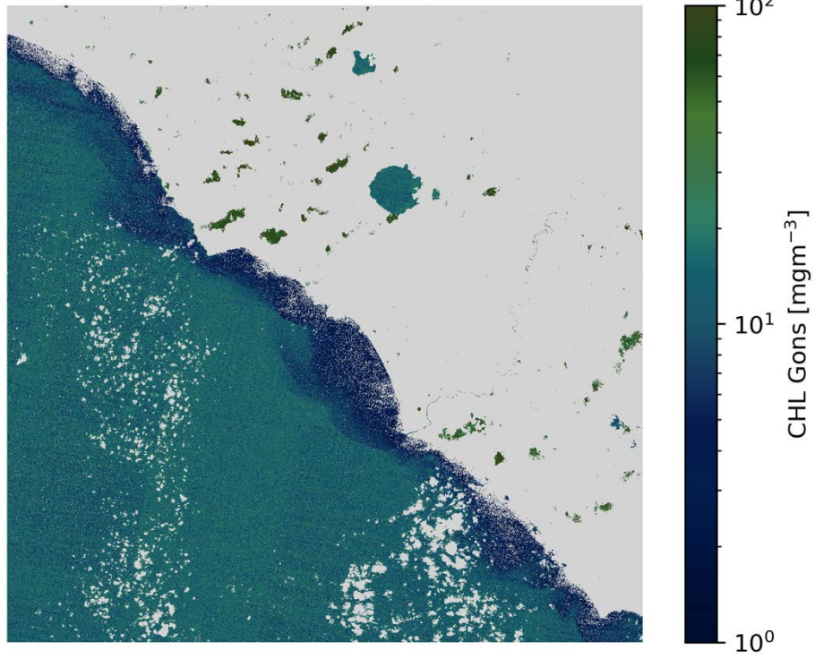
CHL Gons S2B/MSI 2020-10-17 (10:09 UTC)
