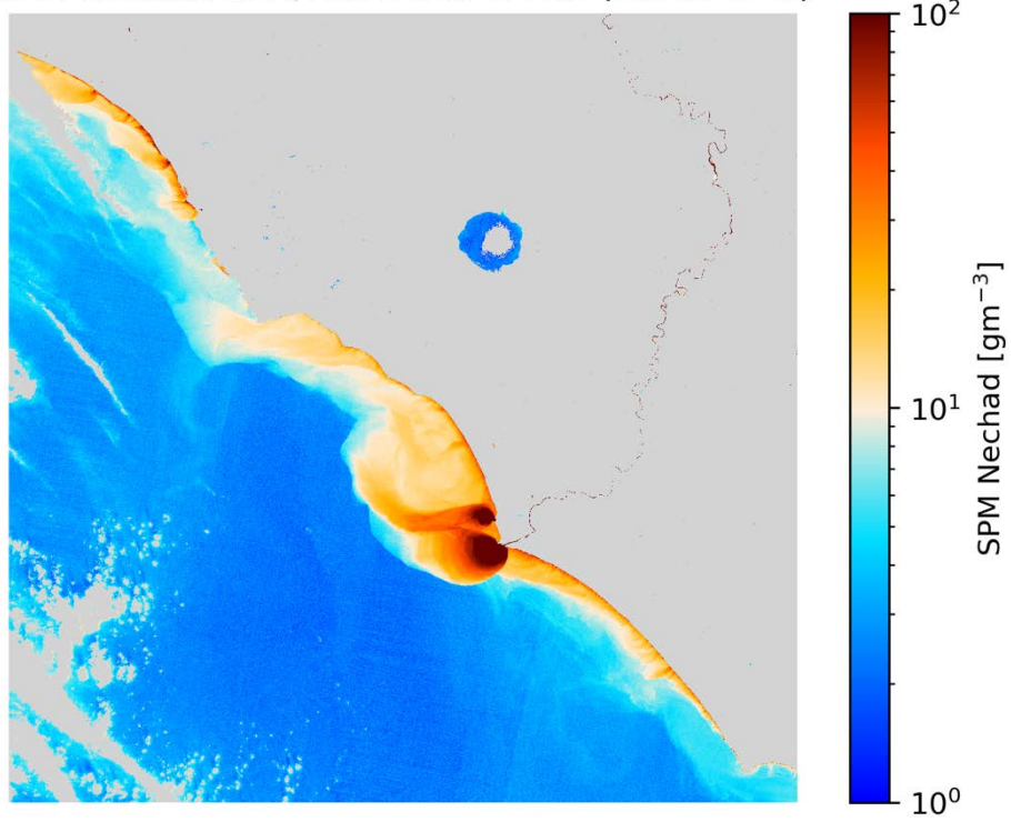
SPM Nechad S2A/MSI 2020-12-11 (10:09 UTC)
