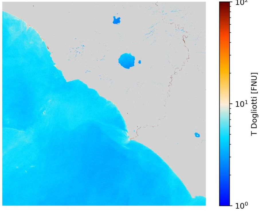
T Dogliotti S2A/MSI 2020-12-21 (10:09 UTC)
