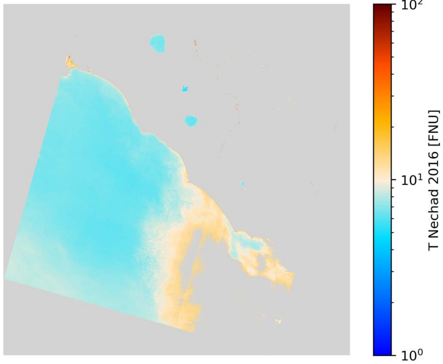
T Nechad 2016 L8/OLI 2020-07-30 (09:53 UTC)
