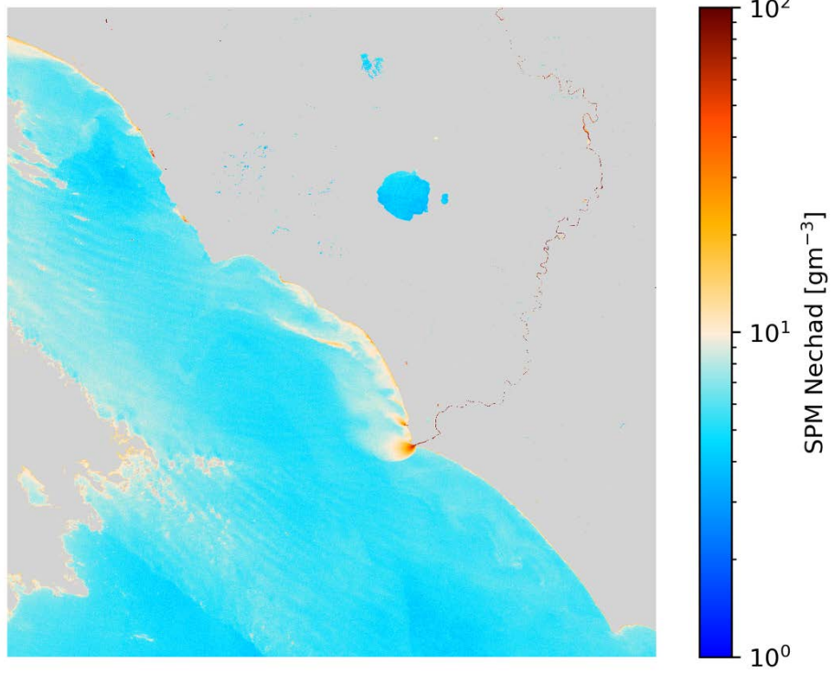
SPM Nechad S2B/MSI 2020-12-16 (10:09 UTC)
