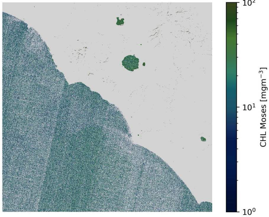
CHL Moses S2A/MSI 2020-12-21 (10:09 UTC)
