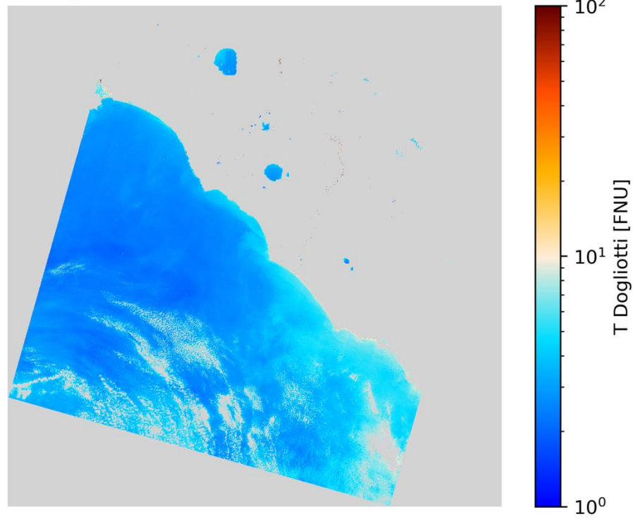
T Dogliotti L8/OLI 2020-08-15 (09:53 UTC)
