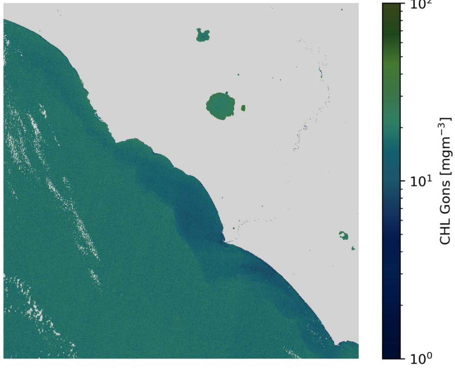
CHL Gons S2A/MSI 2020-04-25 (10:09 UTC)
