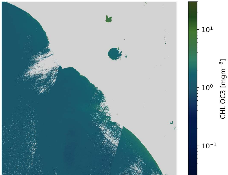
CHL OC3 S2A/MSI 2020-07-14 (10:09 UTC)
