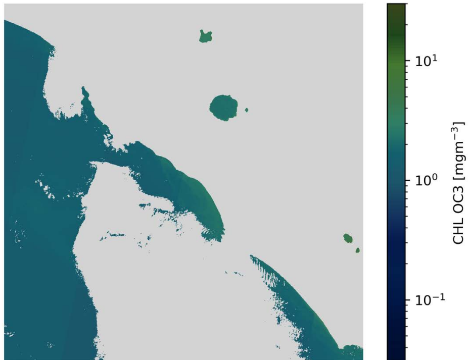
CHL OC3 S2A/MSI 2020-11-11 (10:09 UTC)
