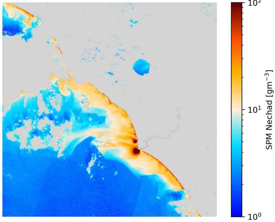
SPM Nechad S2A/MSI 2020-12-31 (10:09 UTC)
