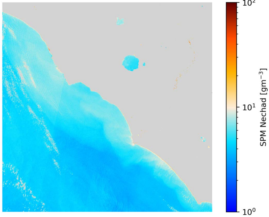
SPM Nechad S2A/MSI 2020-04-25 (10:09 UTC)
