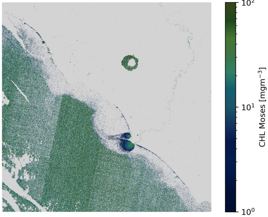
CHL Moses S2A/MSI 2020-12-11 (10:09 UTC)
