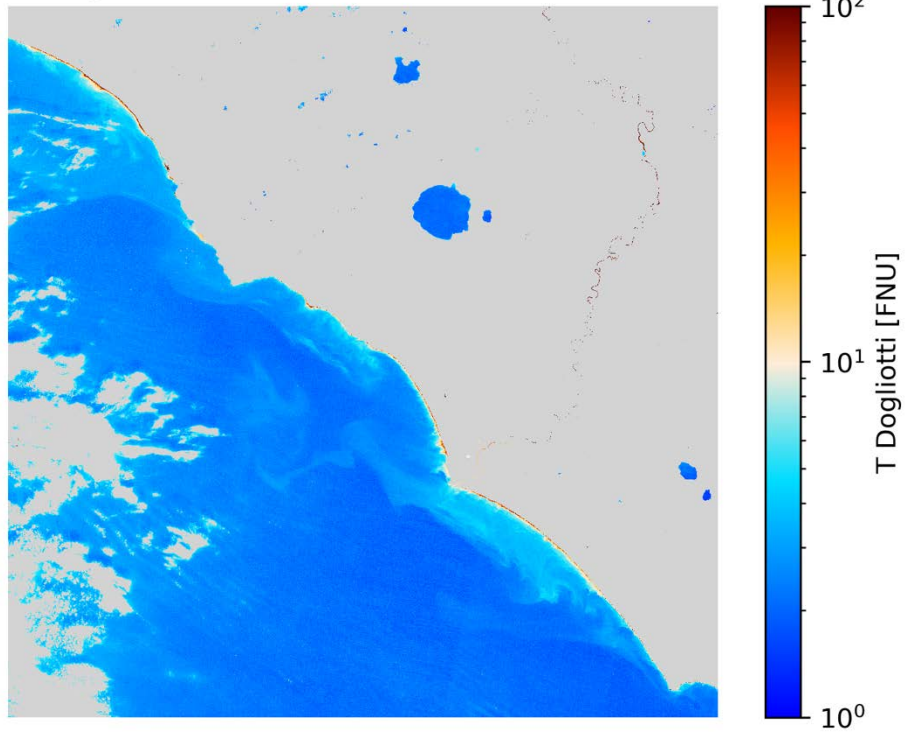
T Dogliotti S2A/MSI 2020-10-22 (10:09 UTC)
