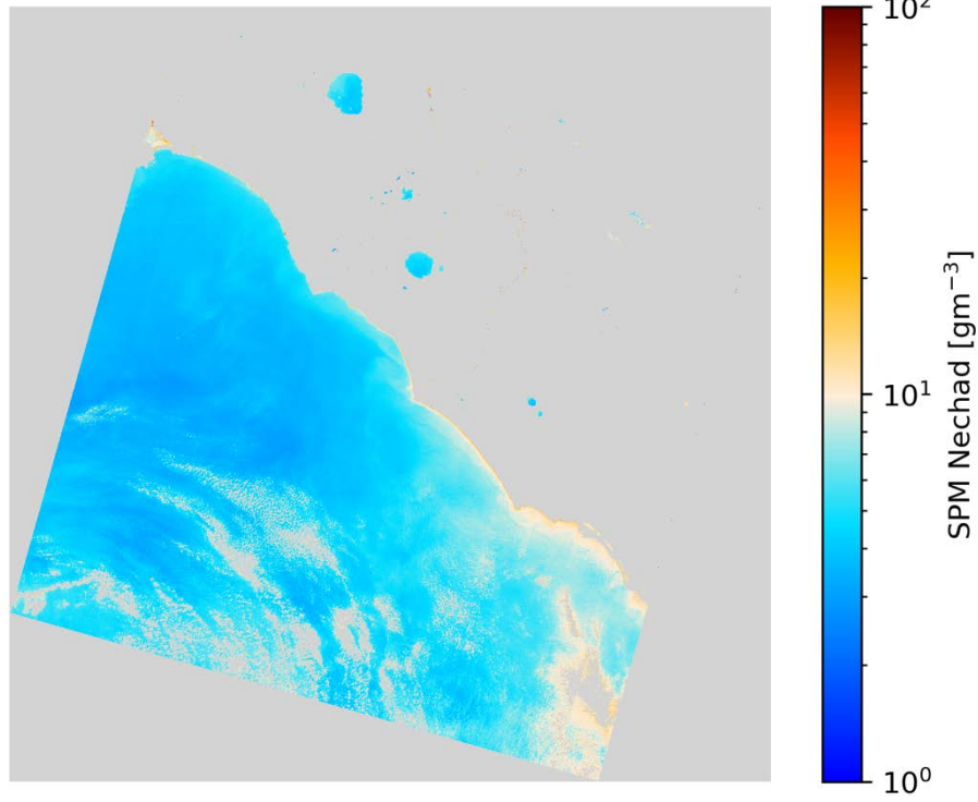
SPM Nechad L8/OLI 2020-08-15 (09:53 UTC)
