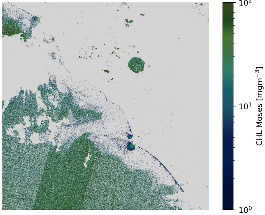
CHL Moses S2A/MSI 2020-12-31 (10:09 UTC)
