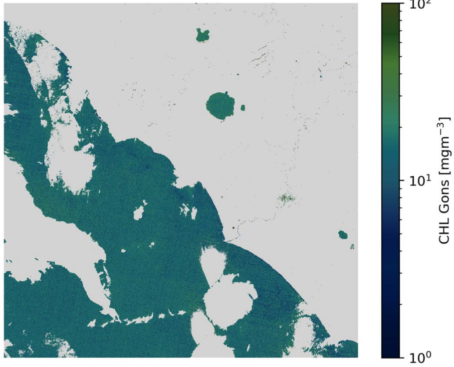
CHL Gons S2B/MSI 2020-11-26 (10:09 UTC)
