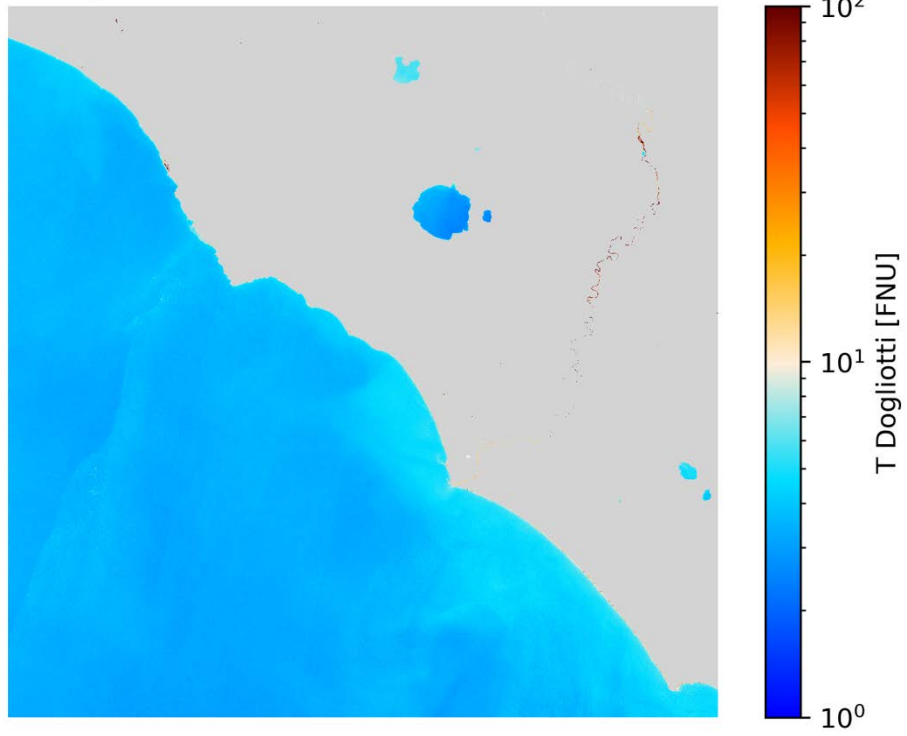
T Dogliotti S2B/MSI 2020-04-10 (10:09 UTC)
