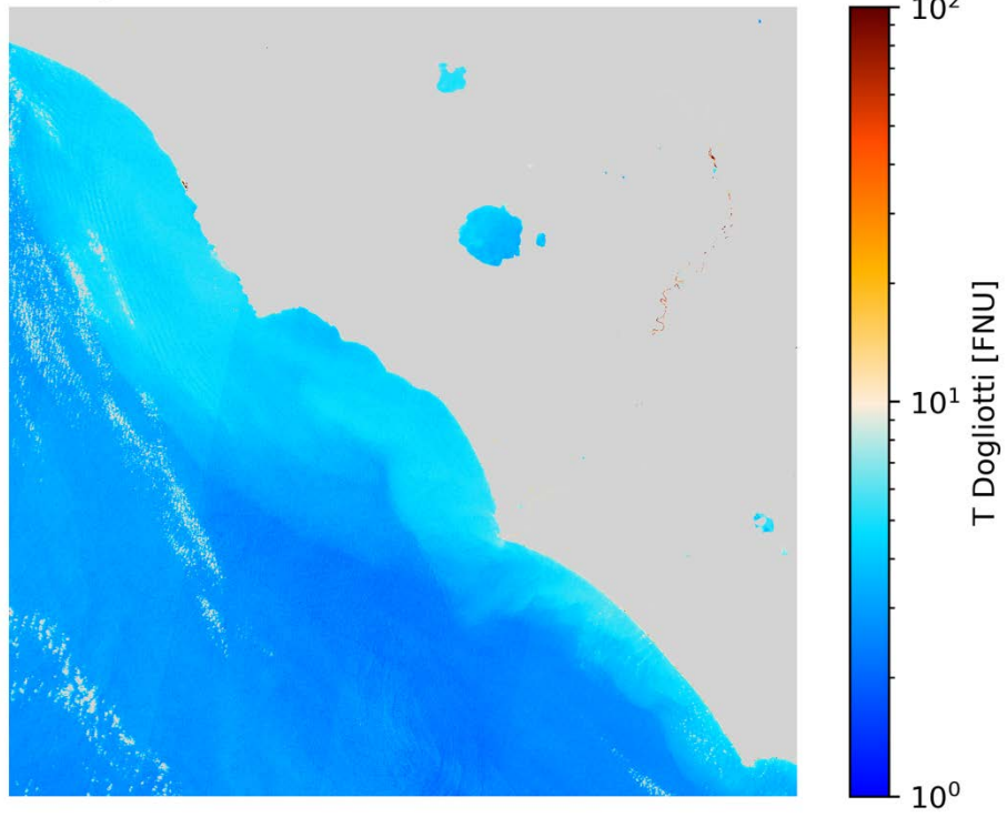
T Dogliotti S2A/MSI 2020-04-25 (10:09 UTC)
