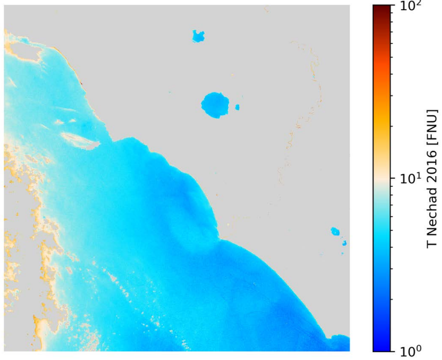
T Nechad 2016 S2B/MSI 2020-09-07 (10:09 UTC)
