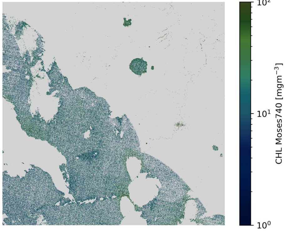
CHL Moses740 S2B/MSI 2020-11-26 (10:09 UTC)
