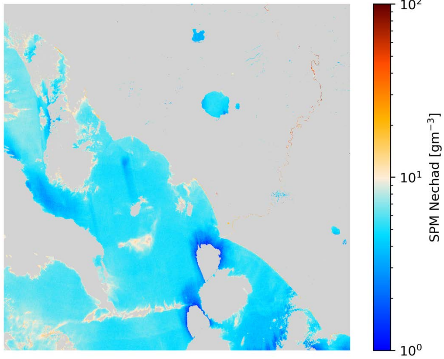
SPM Nechad S2B/MSI 2020-11-26 (10:09 UTC)
