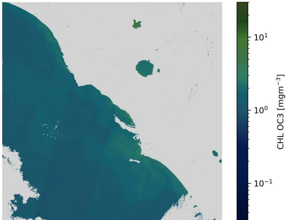
CHL OC3 S2A/MSI 2020-11-01 (10:09 UTC)
