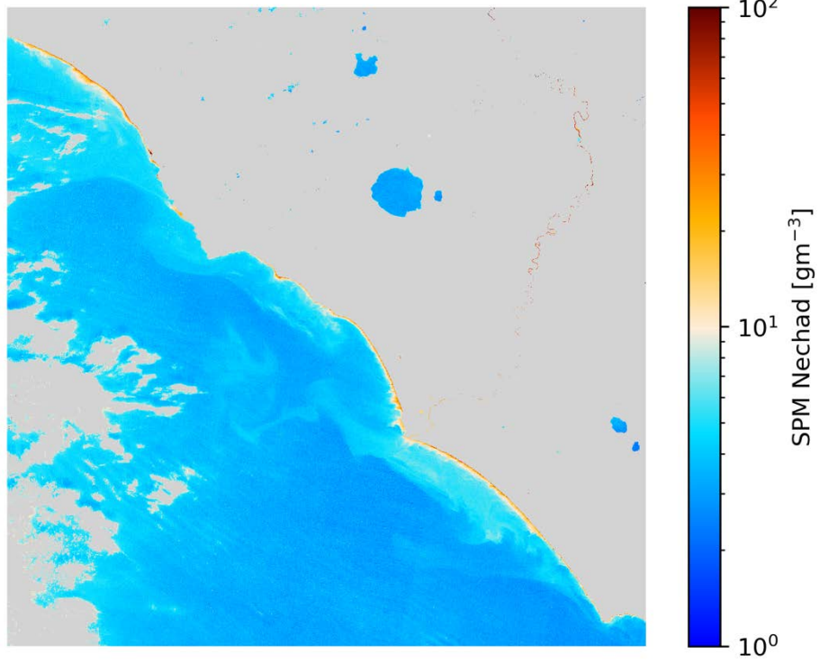
SPM Nechad S2A/MSI 2020-10-22 (10:09 UTC)
