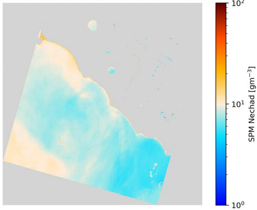
SPM Nechad L8/OLI 2020-09-16 (09:53 UTC)
