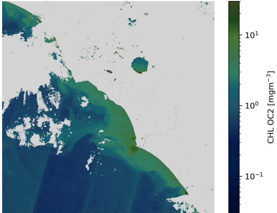
CHL OC2 S2A/MSI 2020-12-31 (10:09 UTC)
