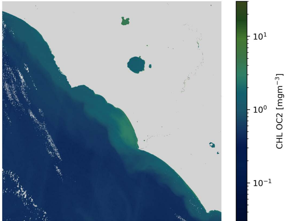
CHL OC2 S2A/MSI 2020-04-25 (10:09 UTC)
