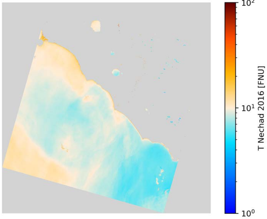
T Nechad 2016 L8/OLI 2020-09-16 (09:53 UTC)
