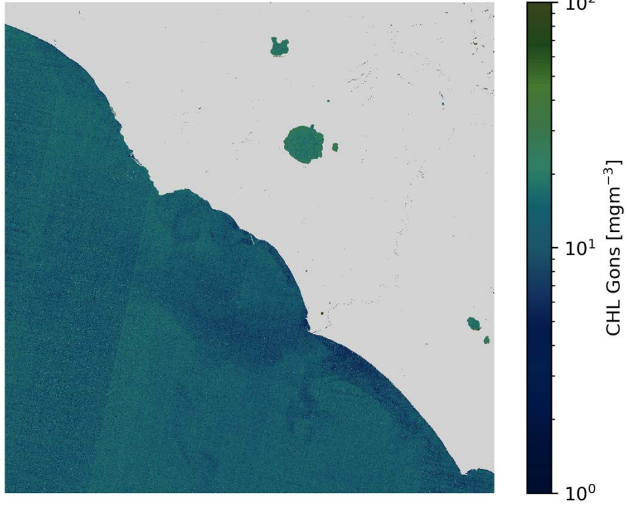
CHL Gons S2B/MSI 2020-11-06 (10:09 UTC)
