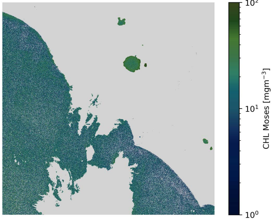
CHL Moses S2A/MSI 2020-04-05 (10:09 UTC)
