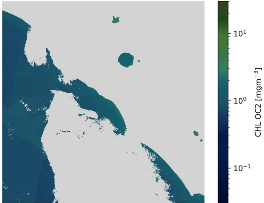
CHL OC2 S2A/MSI 2020-11-11 (10:09 UTC)
