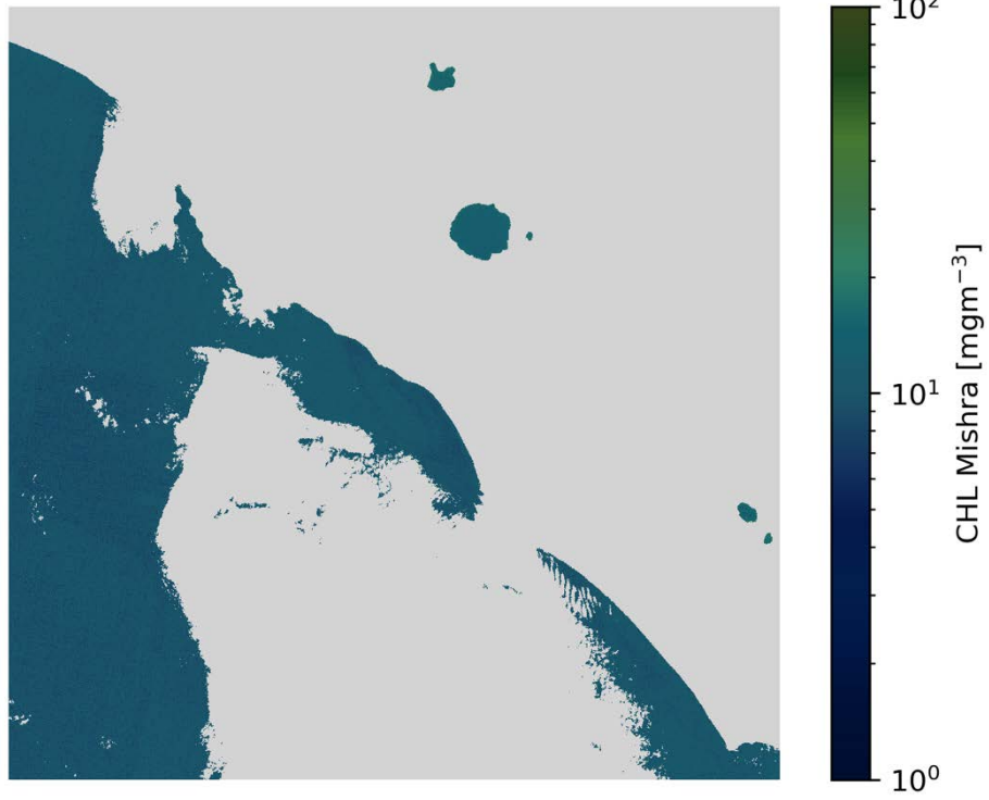
CHL Mishra S2A/MSI 2020-11-11 (10:09 UTC)
