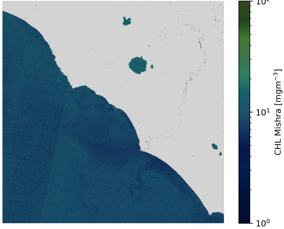
CHL Mishra S2B/MSI 2020-11-06 (10:09 UTC)
