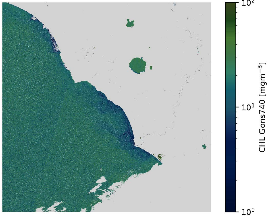
CHL Gons740 S2A/MSI 2020-11-21 (10:09 UTC)
