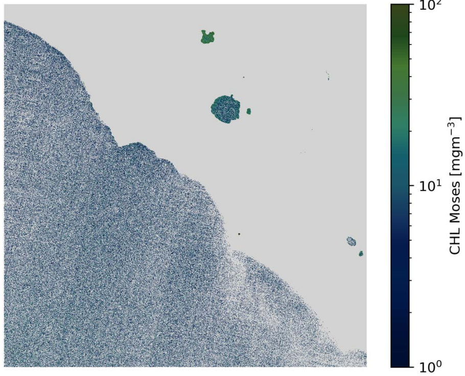
CHL Moses S2B/MSI 2020-09-17 (10:09 UTC)
