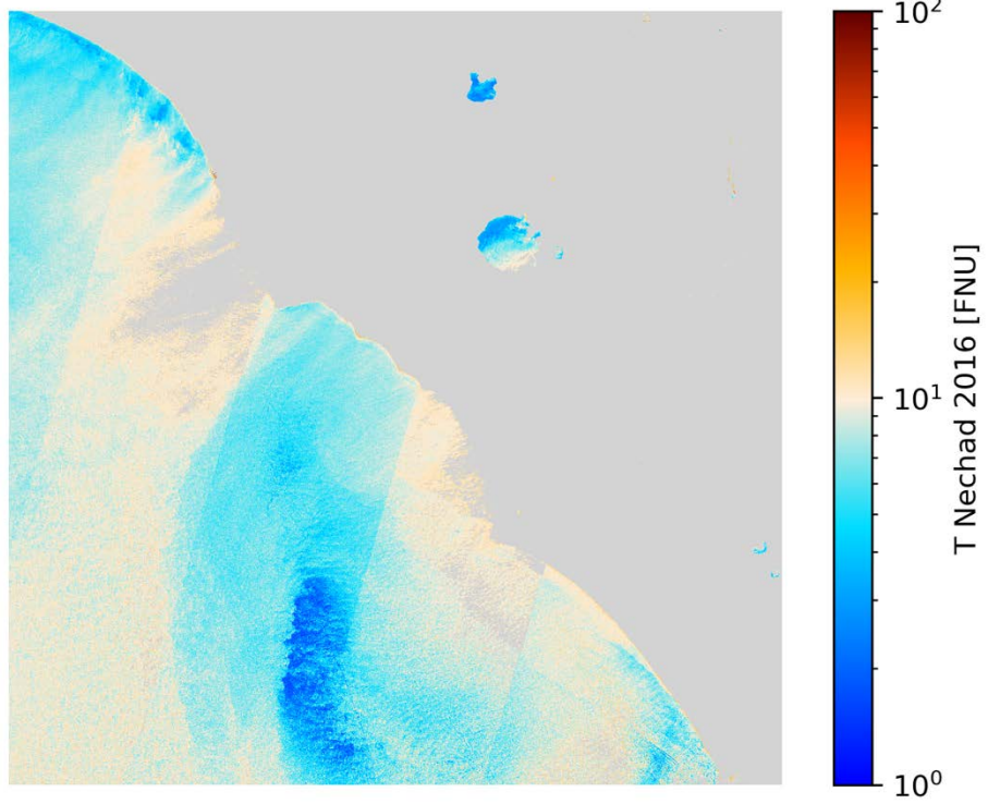
T Nechad 2016 S2A/MSI 2020-07-14 (10:09 UTC)
