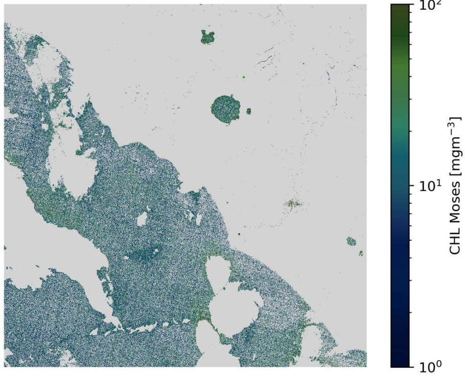
CHL Moses S2B/MSI 2020-11-26 (10:09 UTC)
