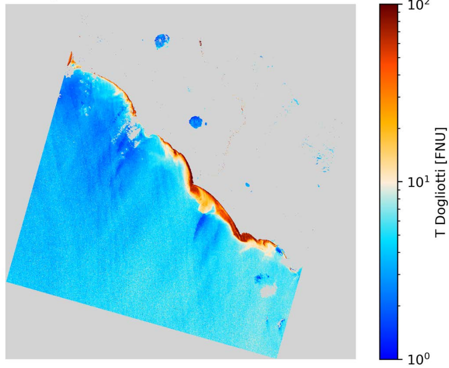
T Dogliotti L8/OLI 2020-02-05 (09:53 UTC)
