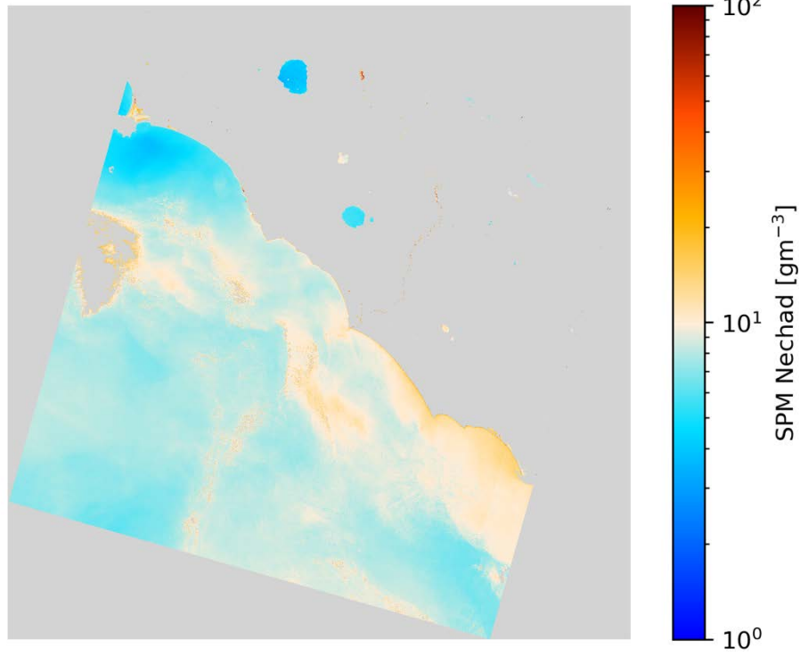
SPM Nechad L8/OLI 2020-04-09 (09:53 UTC)
