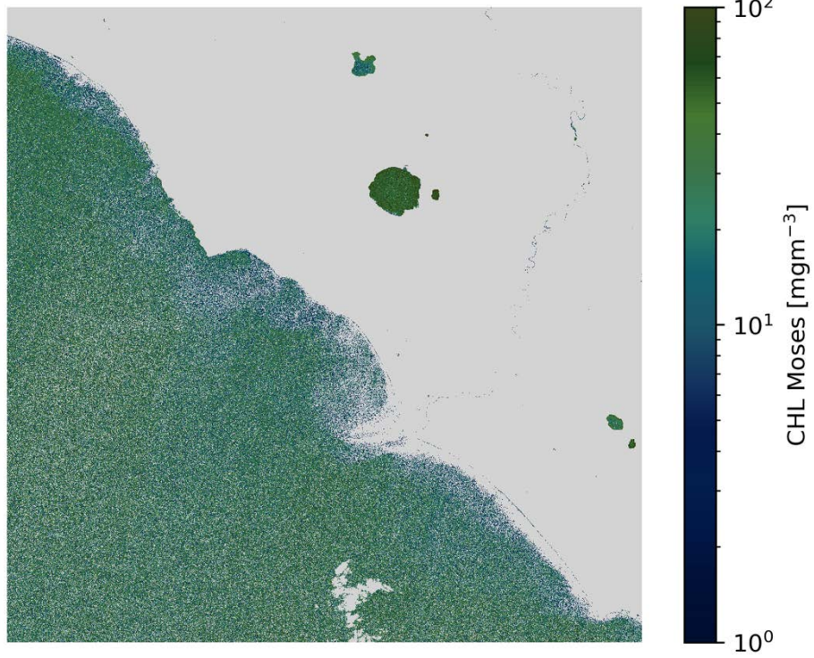
CHL Moses S2A/MSI 2020-04-15 (10:09 UTC)
