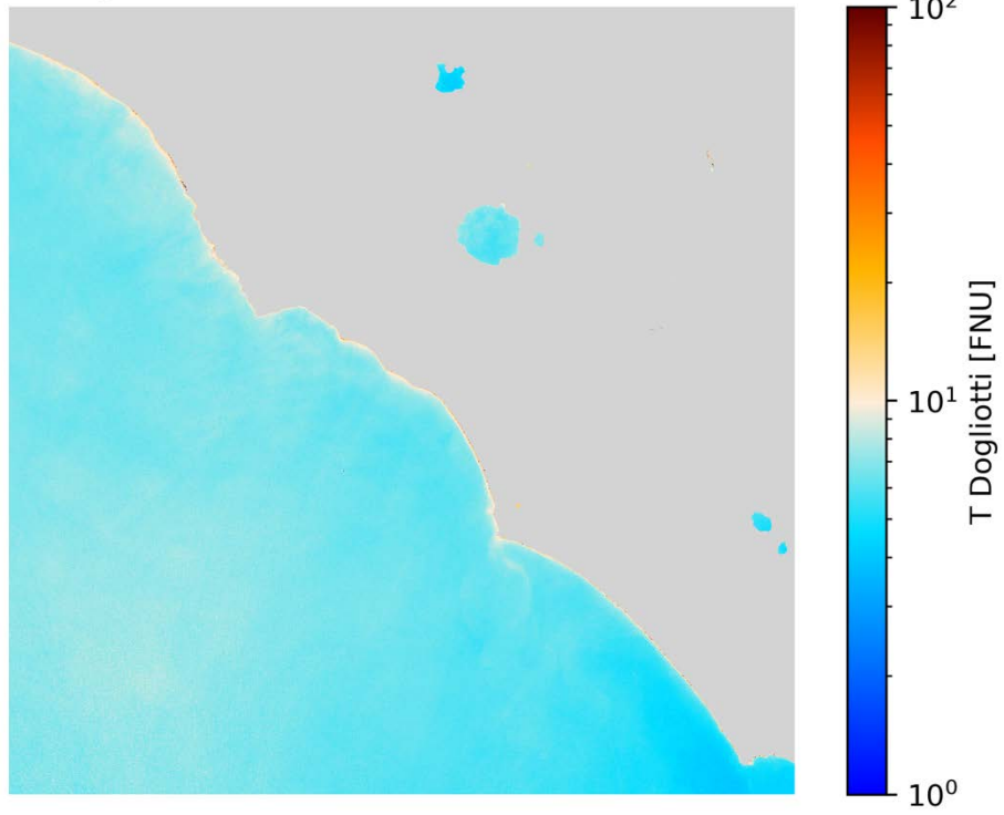
T Dogliotti S2B/MSI 2020-09-17 (10:09 UTC)
