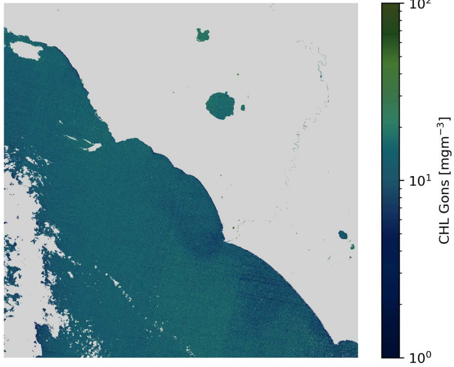
CHL Gons S2B/MSI 2020-09-07 (10:09 UTC)
