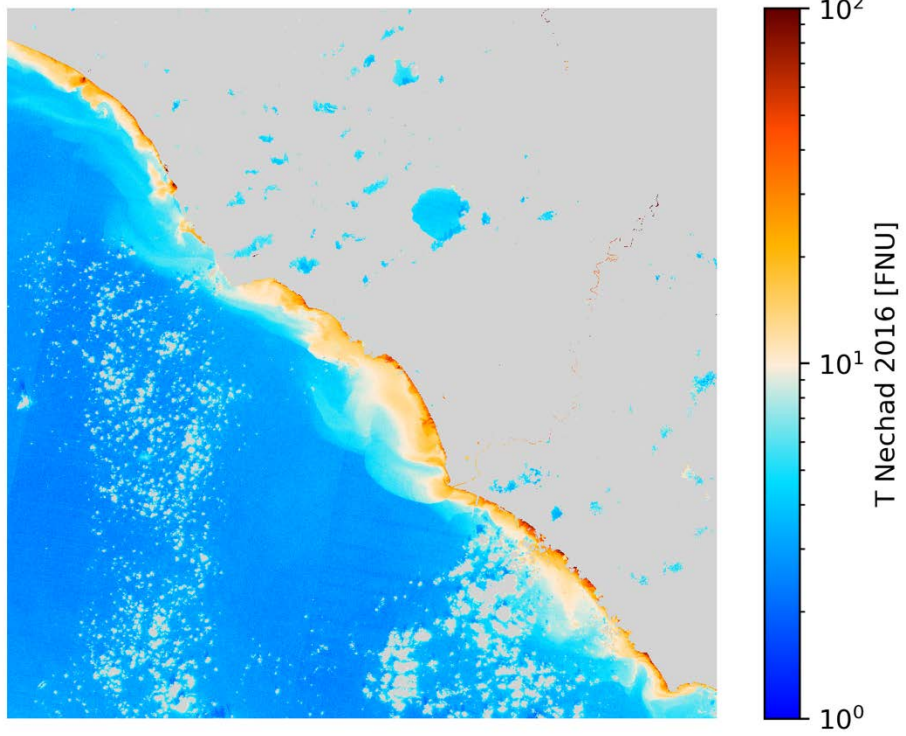
T Nechad 2016 S2B/MSI 2020-10-17 (10:09 UTC)
