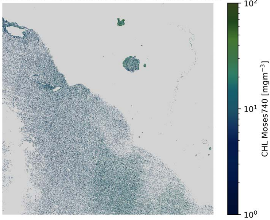
CHL Moses740 S2B/MSI 2020-09-07 (10:09 UTC)
