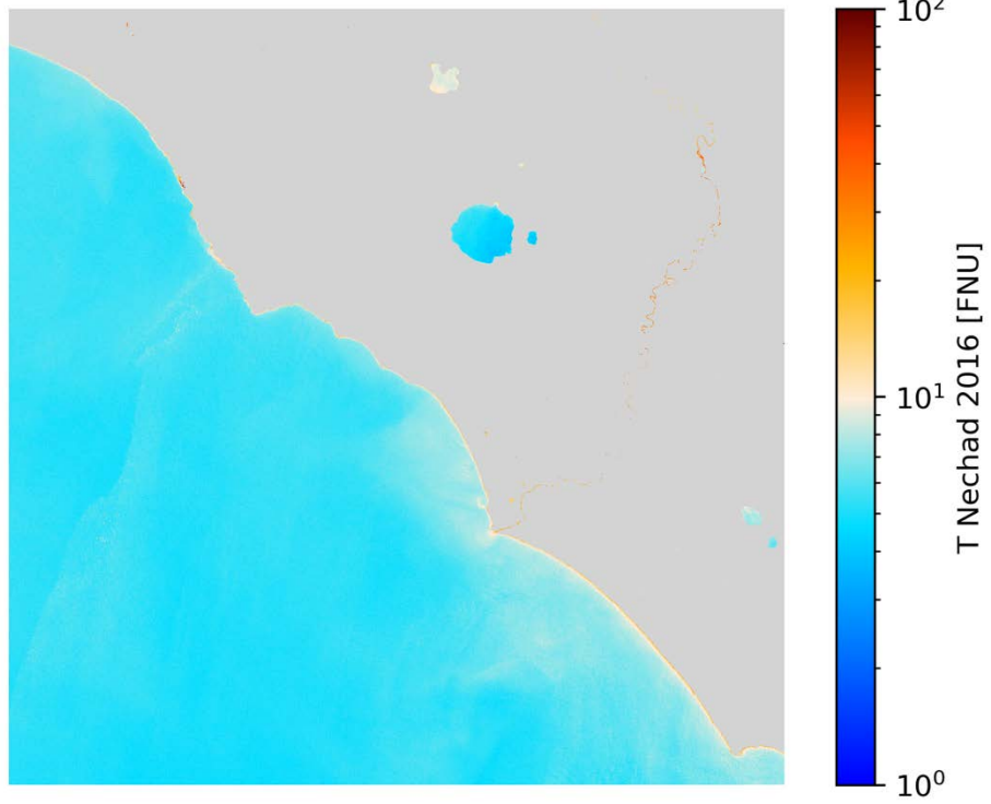
T Nechad 2016 S2B/MSI 2020-04-10 (10:09 UTC)
