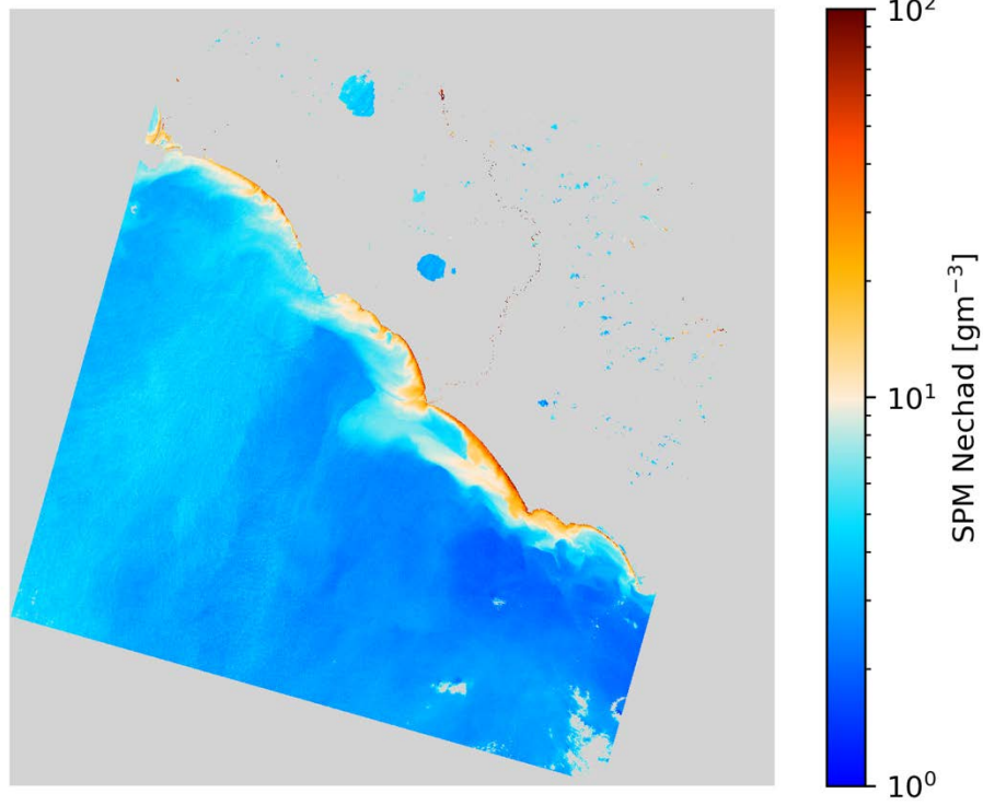
SPM Nechad L8/OLI 2020-03-08 (09:53 UTC)
