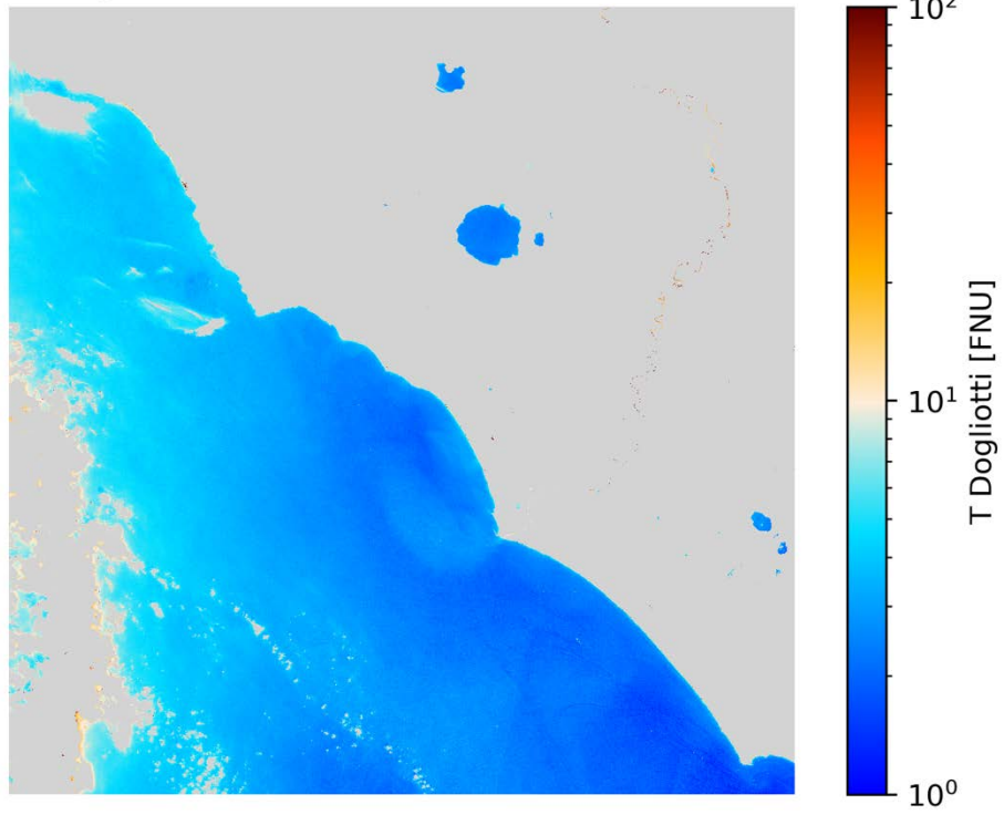
T Dogliotti S2B/MSI 2020-09-07 (10:09 UTC)
