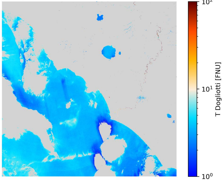
T Dogliotti S2B/MSI 2020-11-26 (10:09 UTC)
