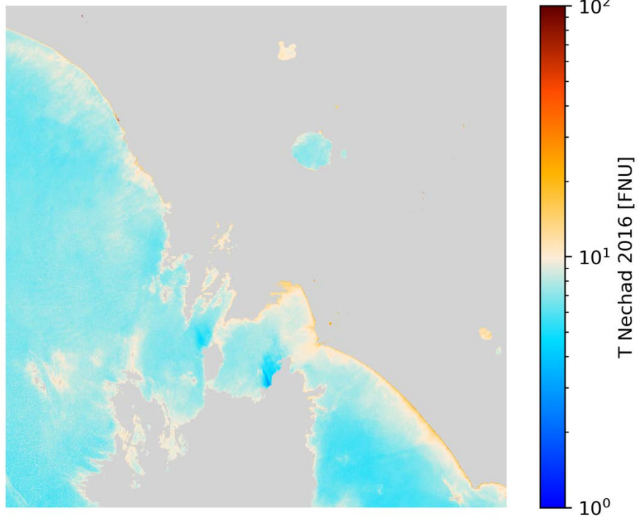
T Nechad 2016 S2A/MSI 2020-04-05 (10:09 UTC)
