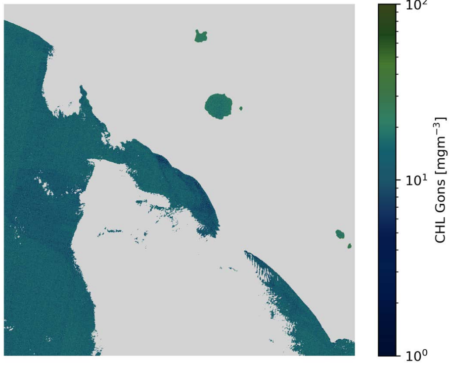
CHL Gons S2A/MSI 2020-11-11 (10:09 UTC)
