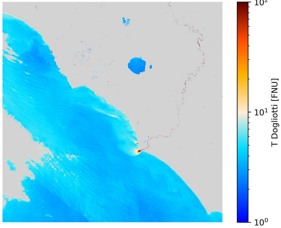
T Dogliotti S2B/MSI 2020-12-16 (10:09 UTC)
