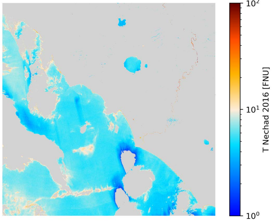
T Nechad 2016 S2B/MSI 2020-11-26 (10:09 UTC)
