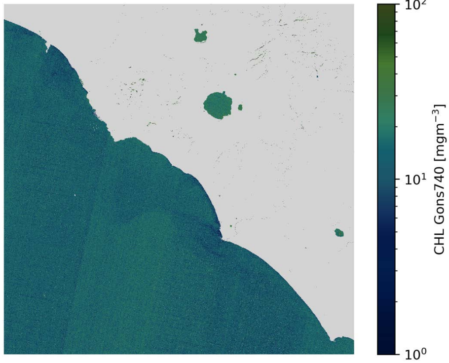
CHL Gons740 S2A/MSI 2020-12-21 (10:09 UTC)
