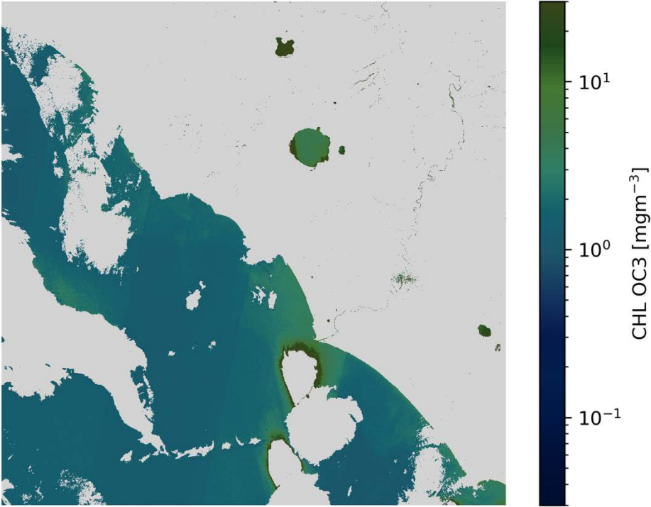
CHL OC3 S2B/MSI 2020-11-26 (10:09 UTC)
