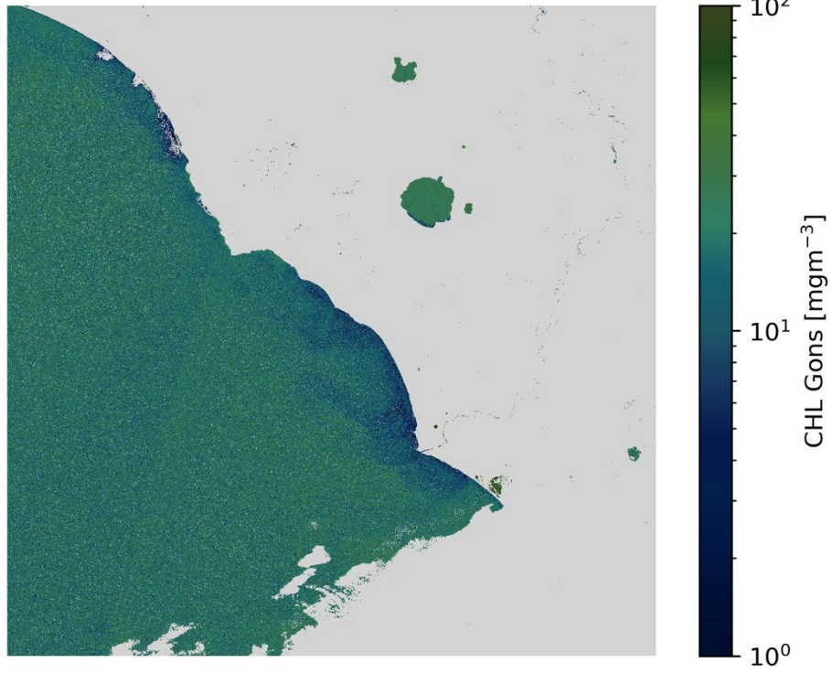
CHL Gons S2A/MSI 2020-11-21 (10:09 UTC)
