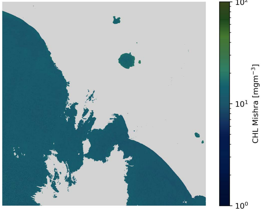
CHL Mishra S2A/MSI 2020-04-05 (10:09 UTC)
