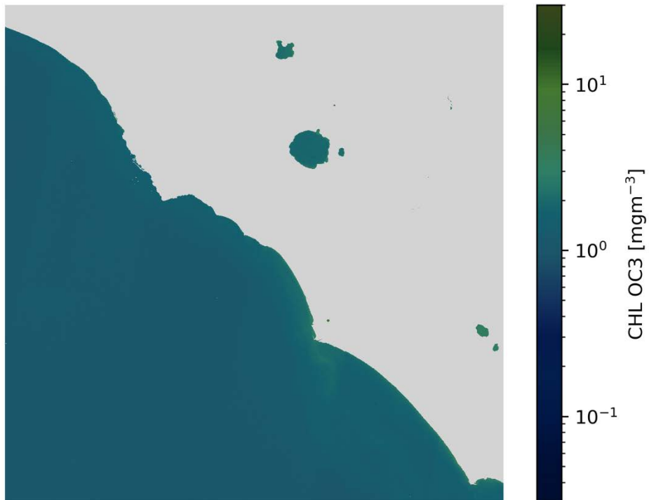
CHL OC3 S2B/MSI 2020-09-17 (10:09 UTC)
