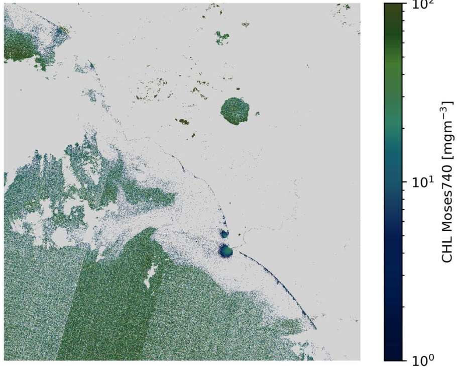
CHL Moses740 S2A/MSI 2020-12-31 (10:09 UTC)
