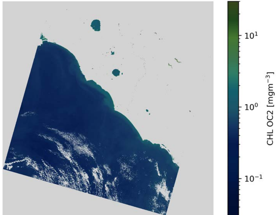
CHL OC2 L8/OLI 2020-08-15 (09:53 UTC)
