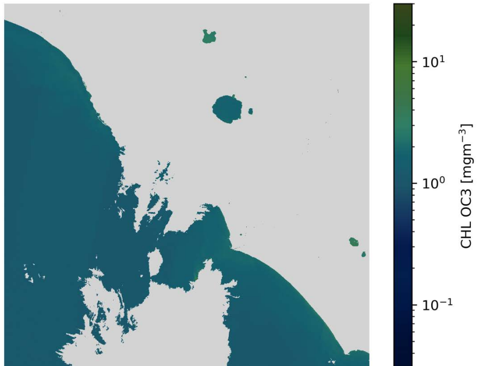
CHL OC3 S2A/MSI 2020-04-05 (10:09 UTC)
