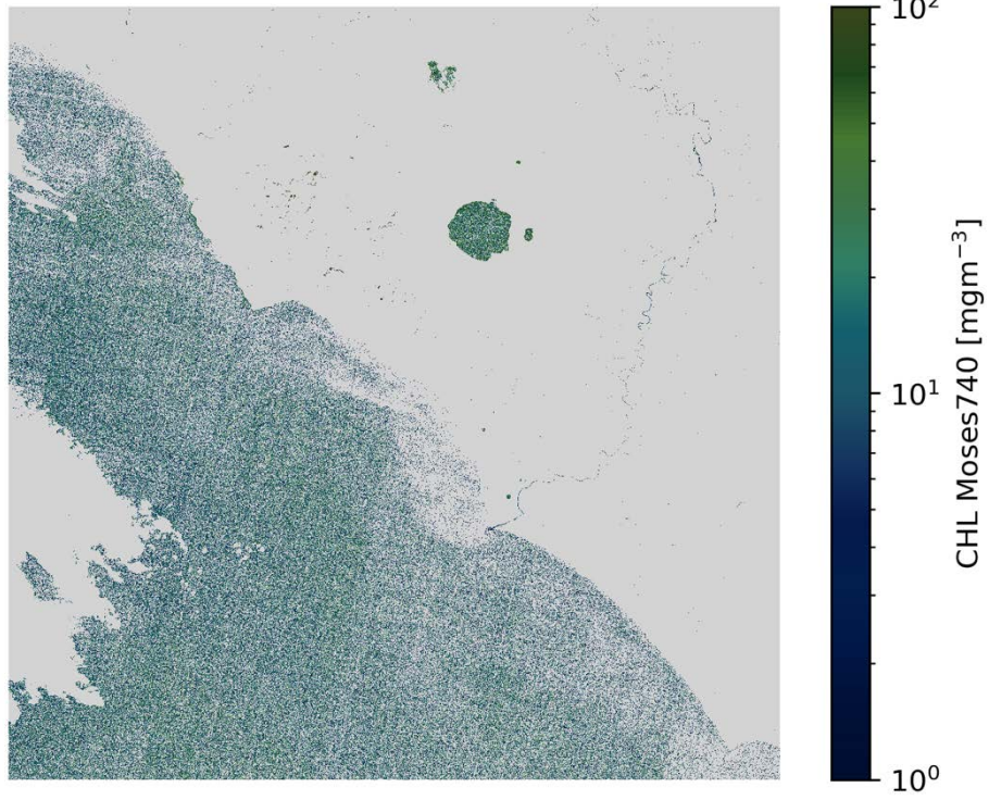
CHL Moses740 S2B/MSI 2020-12-16 (10:09 UTC)
