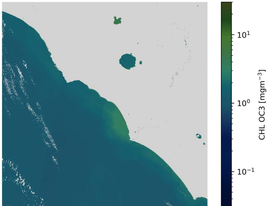
CHL OC3 S2A/MSI 2020-04-25 (10:09 UTC)
