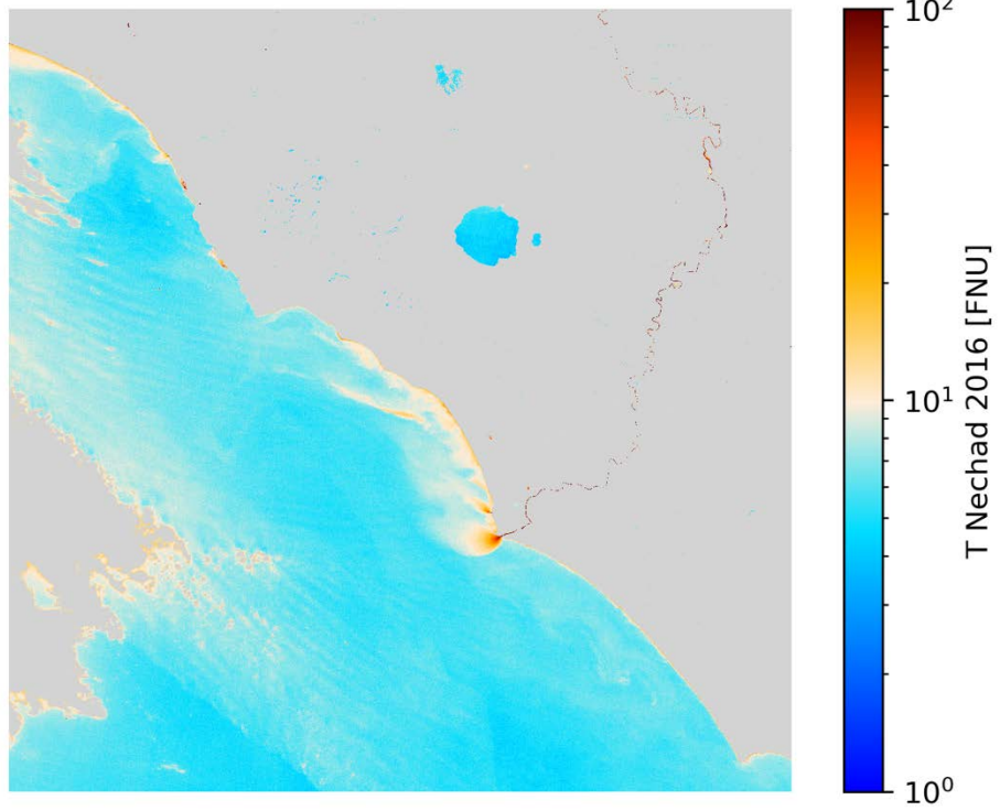
T Nechad 2016 S2B/MSI 2020-12-16 (10:09 UTC)
