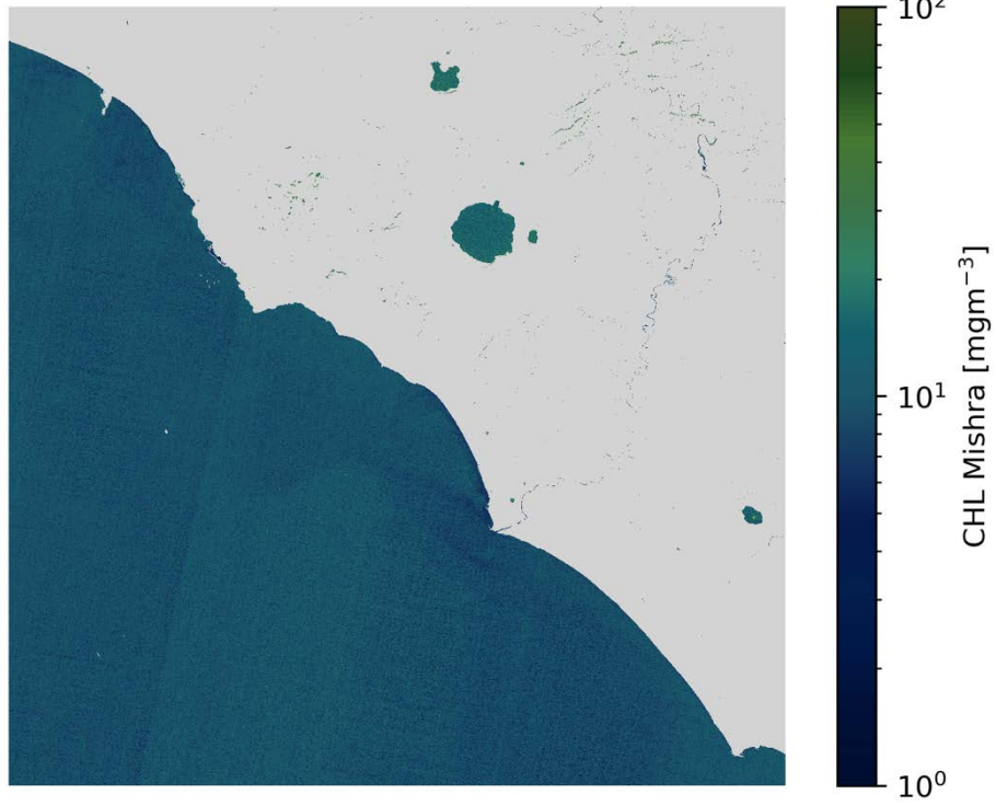
CHL Mishra S2A/MSI 2020-12-21 (10:09 UTC)
