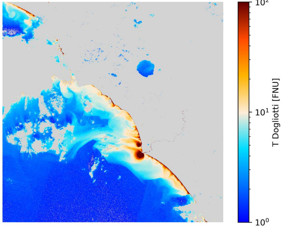
T Dogliotti S2A/MSI 2020-12-31 (10:09 UTC)
