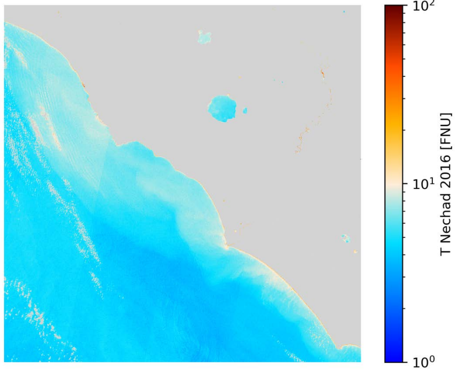
T Nechad 2016 S2A/MSI 2020-04-25 (10:09 UTC)
