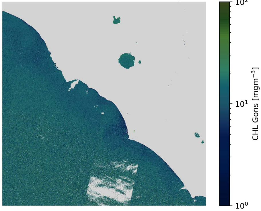
CHL Gons S2B/MSI 2020-08-08 (10:09 UTC)
