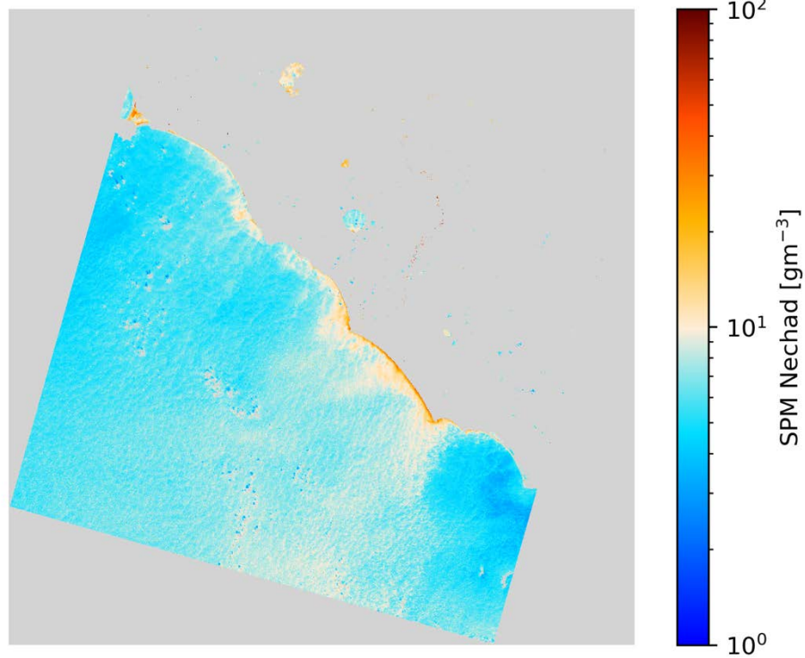
SPM Nechad L8/OLI 2020-03-24 (09:53 UTC)
