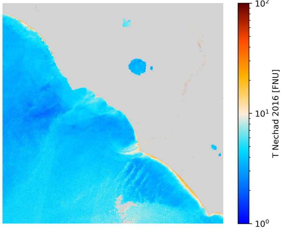
T Nechad 2016 S2A/MSI 2020-04-15 (10:09 UTC)
