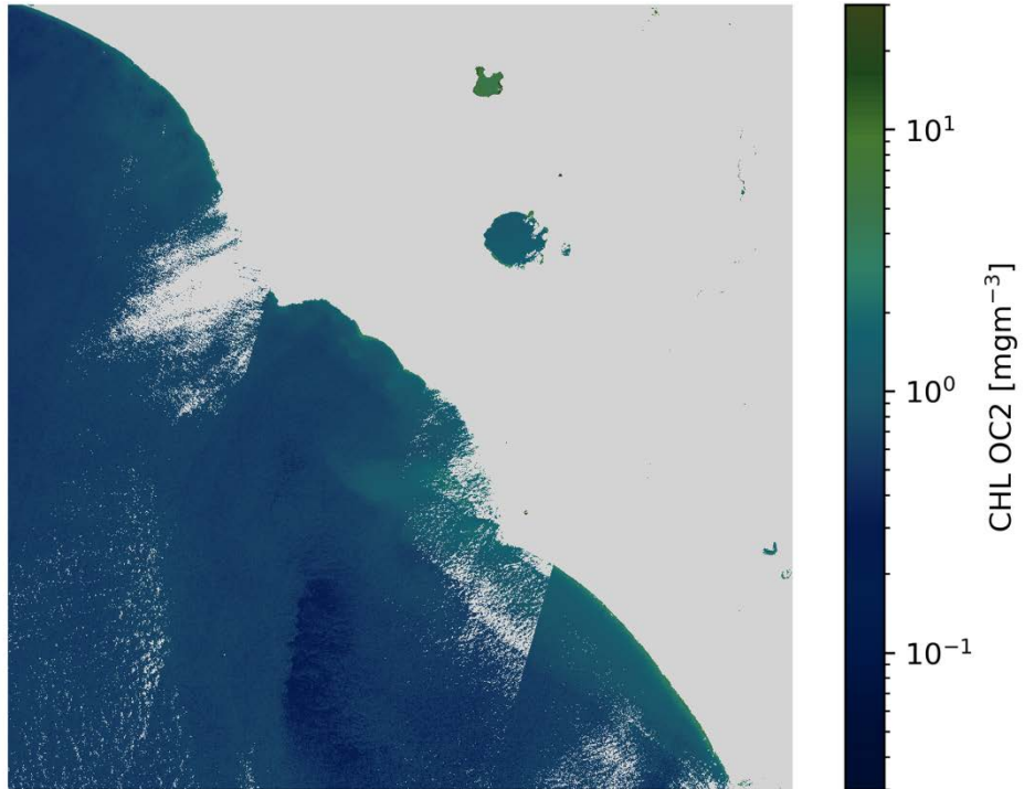
CHL OC2 S2A/MSI 2020-07-14 (10:09 UTC)
