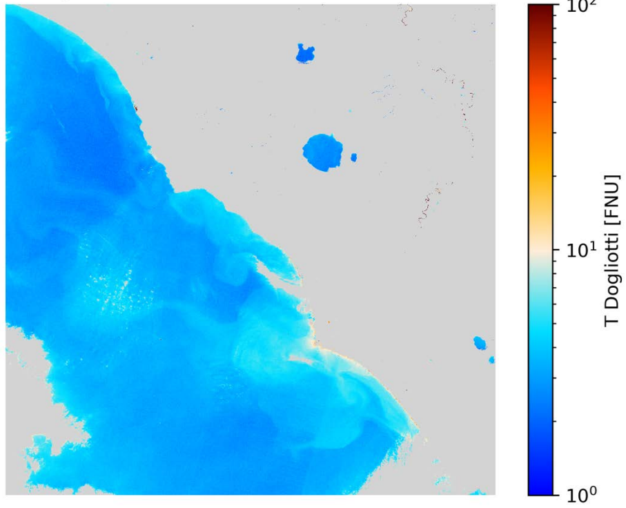
T Dogliotti S2A/MSI 2020-11-01 (10:09 UTC)
