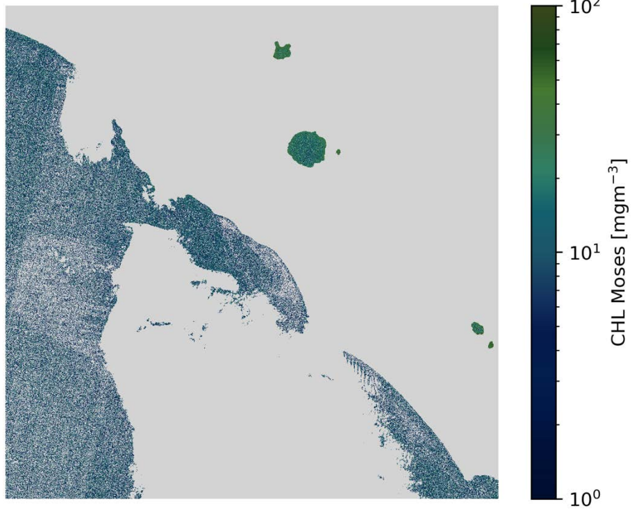
CHL Moses S2A/MSI 2020-11-11 (10:09 UTC)
