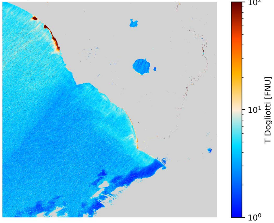
T Dogliotti S2A/MSI 2020-11-21 (10:09 UTC)
