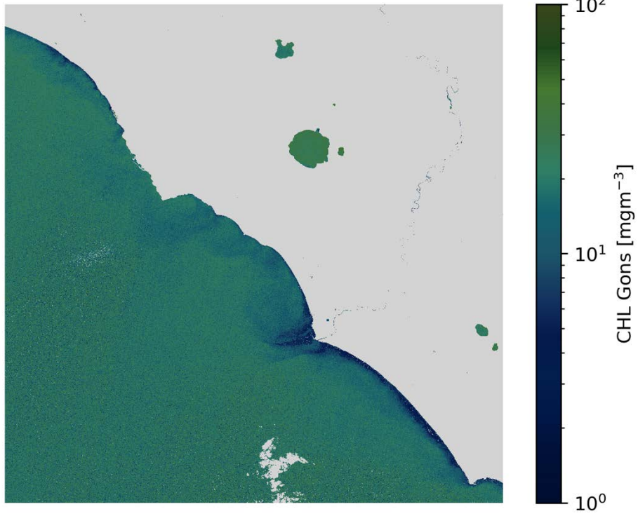
CHL Gons S2A/MSI 2020-04-15 (10:09 UTC)
