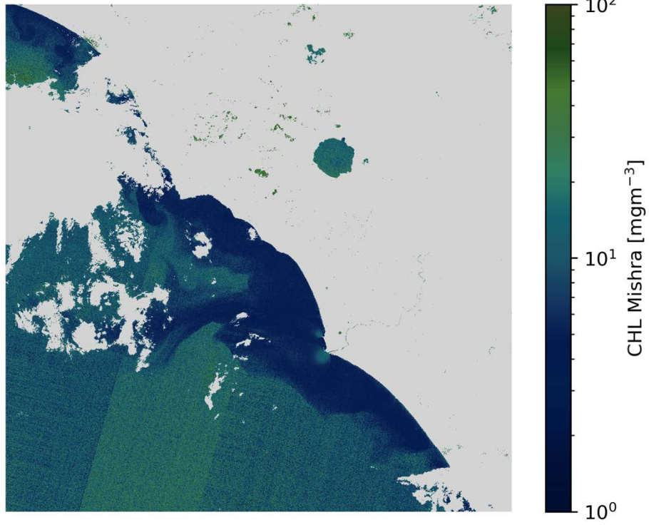
CHL Mishra S2A/MSI 2020-12-31 (10:09 UTC)
