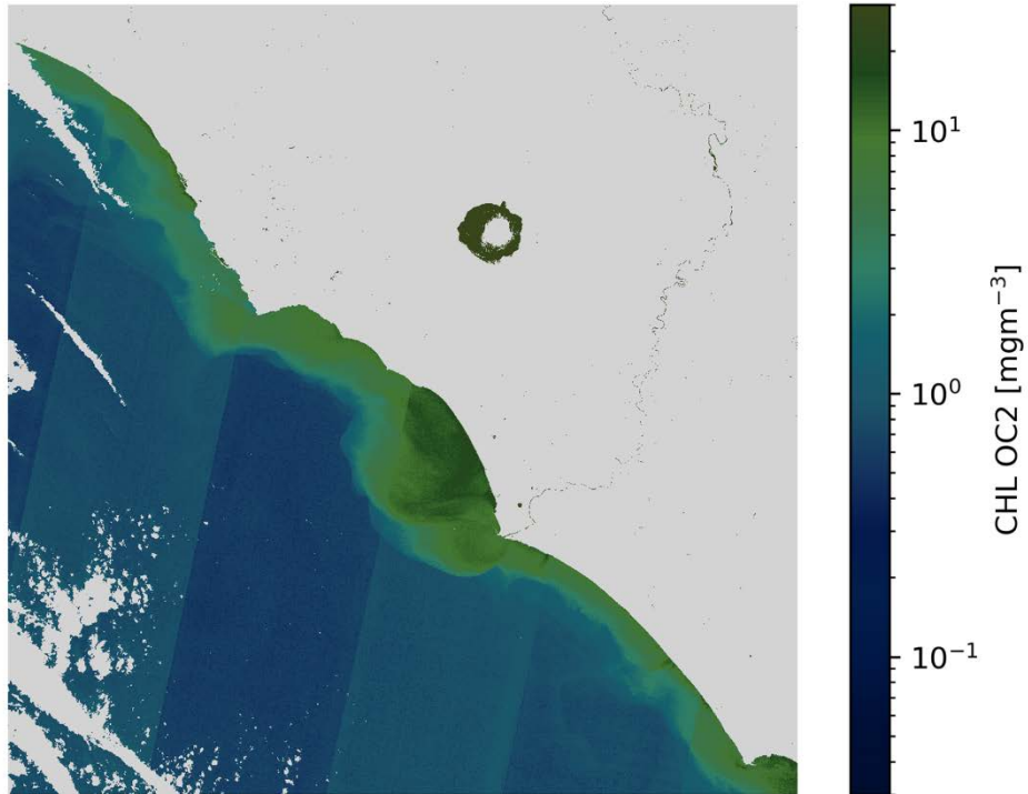
CHL OC2 S2A/MSI 2020-12-11 (10:09 UTC)
