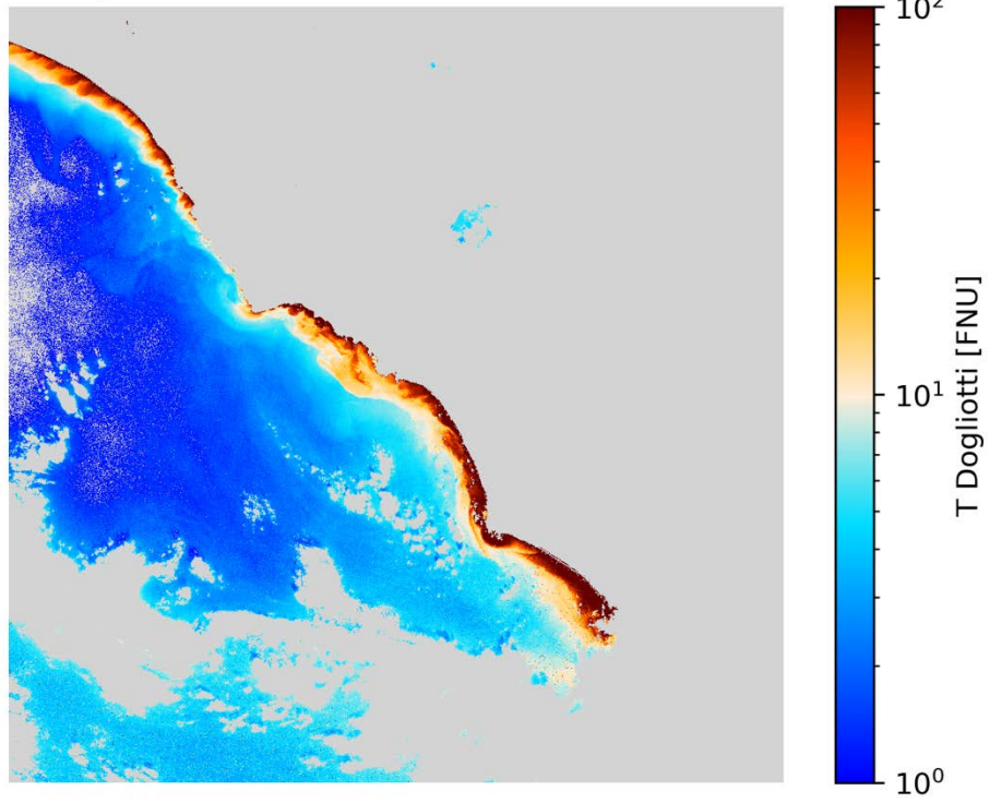
T Dogliotti S2A/MSI 2020-03-06 (10:09 UTC)
