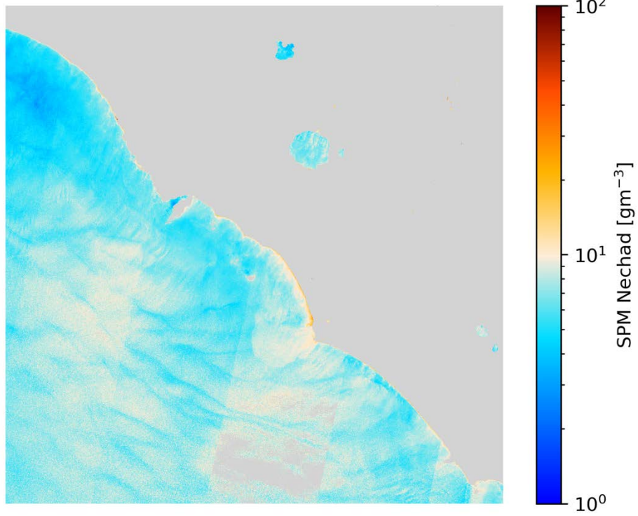
SPM Nechad S2B/MSI 2020-08-08 (10:09 UTC)
