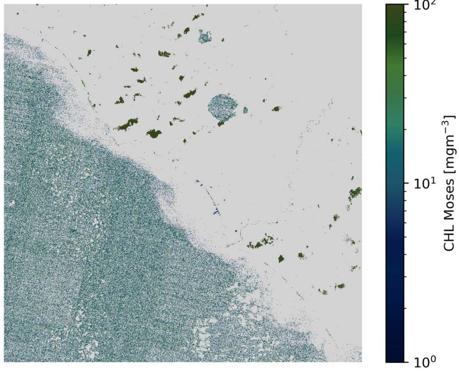
CHL Moses S2B/MSI 2020-10-17 (10:09 UTC)
