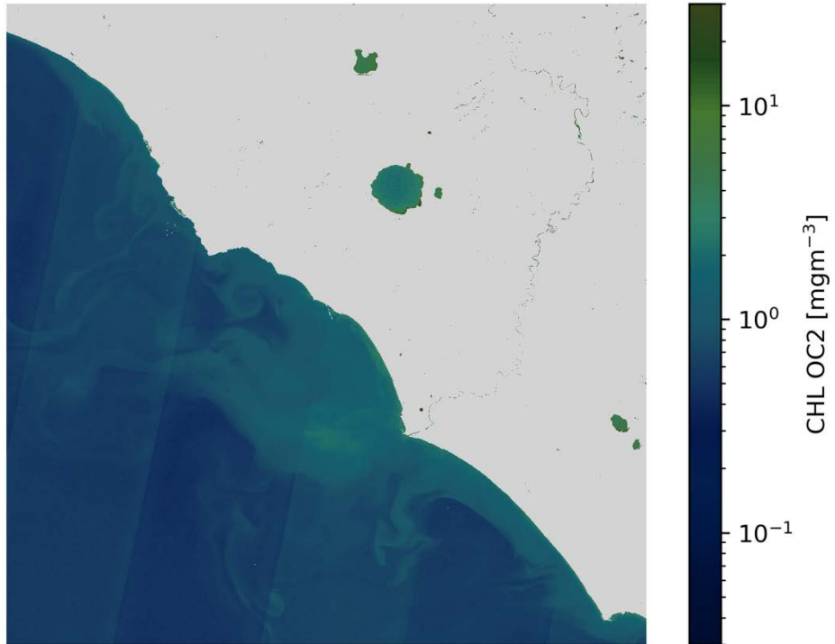
CHL OC2 S2B/MSI 2020-11-06 (10:09 UTC)
