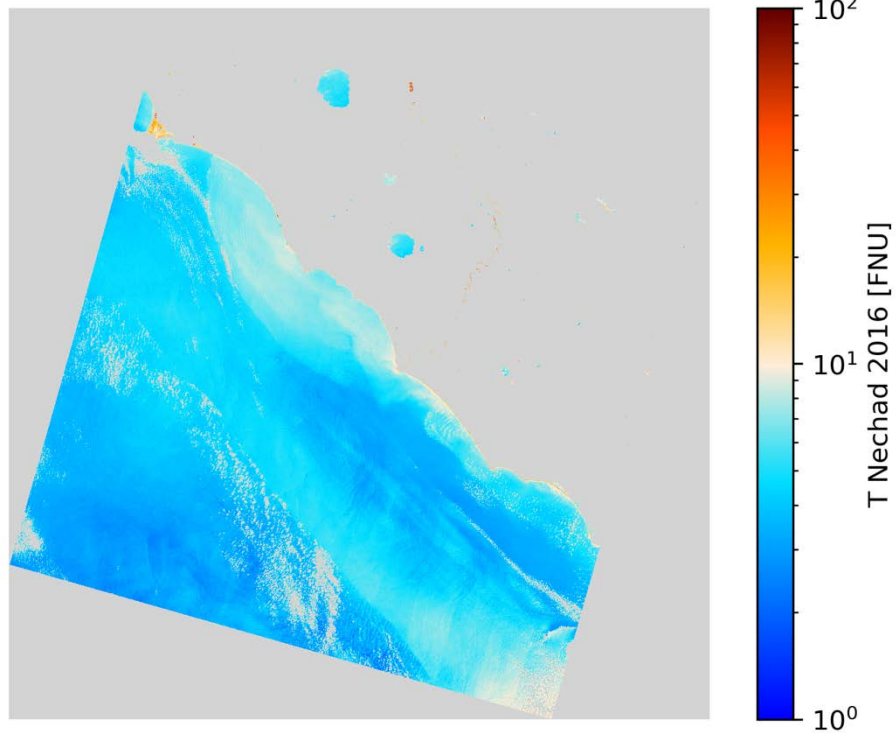
T Nechad 2016 L8/OLI 2020-04-25 (09:52 UTC)
