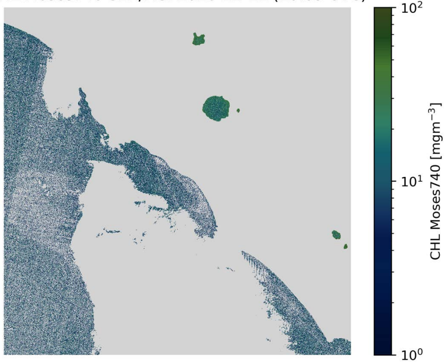
CHL Moses740 S2A/MSI 2020-11-11 (10:09 UTC)
