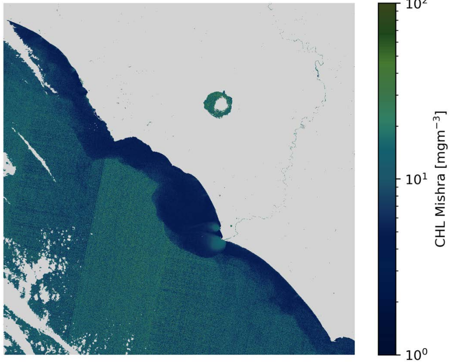
CHL Mishra S2A/MSI 2020-12-11 (10:09 UTC)
