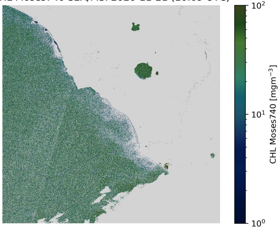
CHL Moses740 S2A/MSI 2020-11-21 (10:09 UTC)
