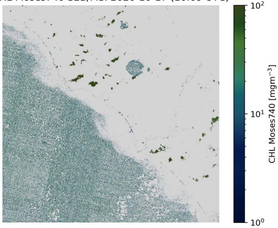
CHL Moses740 S2B/MSI 2020-10-17 (10:09 UTC)
