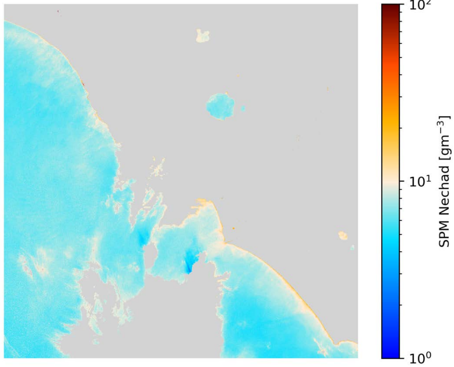
SPM Nechad S2A/MSI 2020-04-05 (10:09 UTC)
