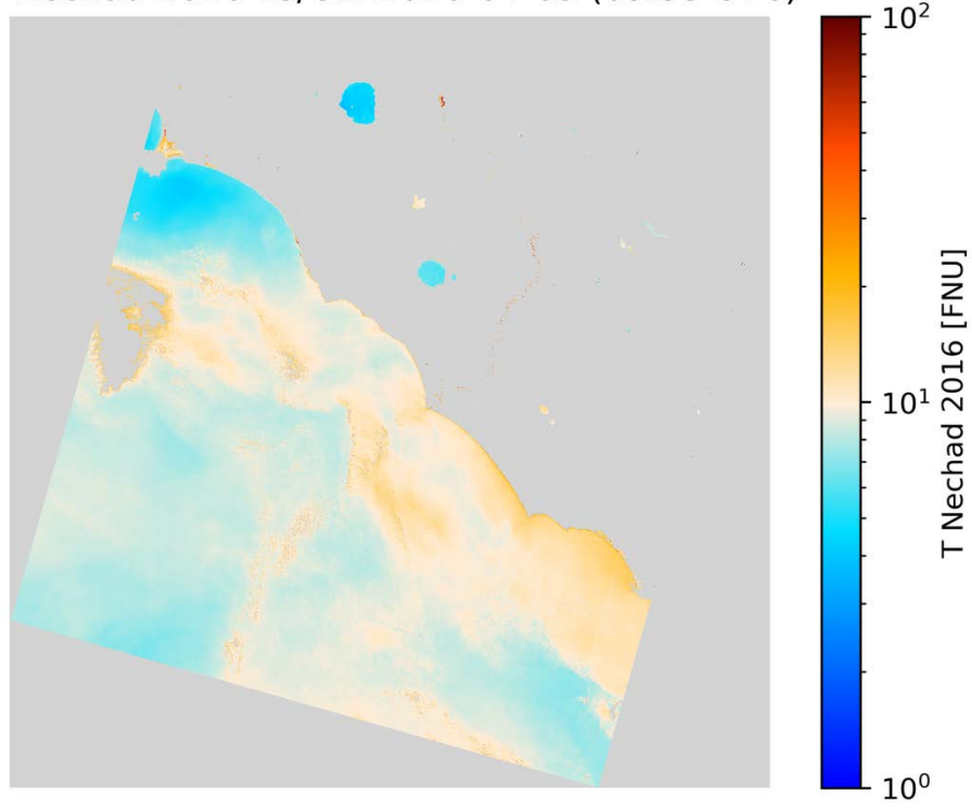
T Nechad 2016 L8/OLI 2020-04-09 (09:53 UTC)
