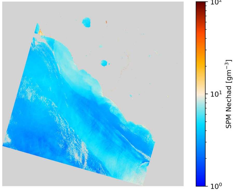
SPM Nechad L8/OLI 2020-04-25 (09:52 UTC)
