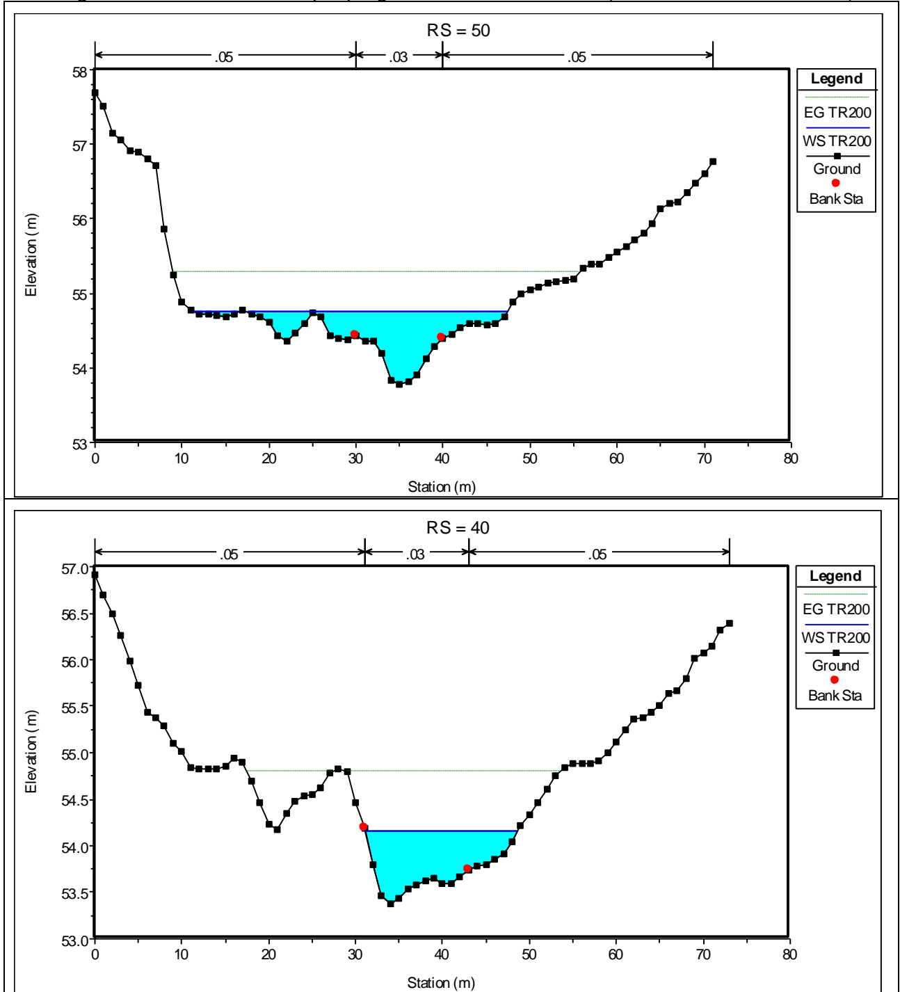
Fig.5.4/C: Schermate di Output programma – Cross Section (RS50: monte /RS10: valle)
