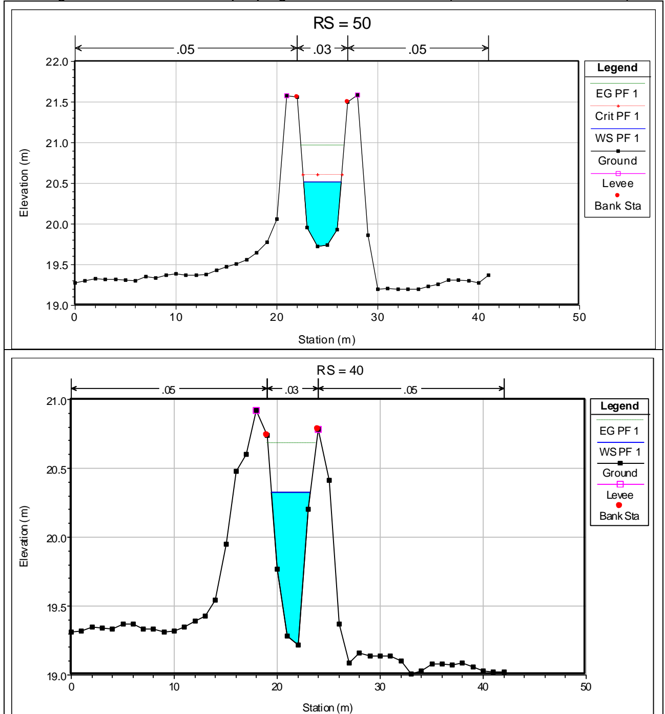
Fig.5.3/C: Schermate di Output programma – Cross Section (RS50: monte /RS10: valle)
