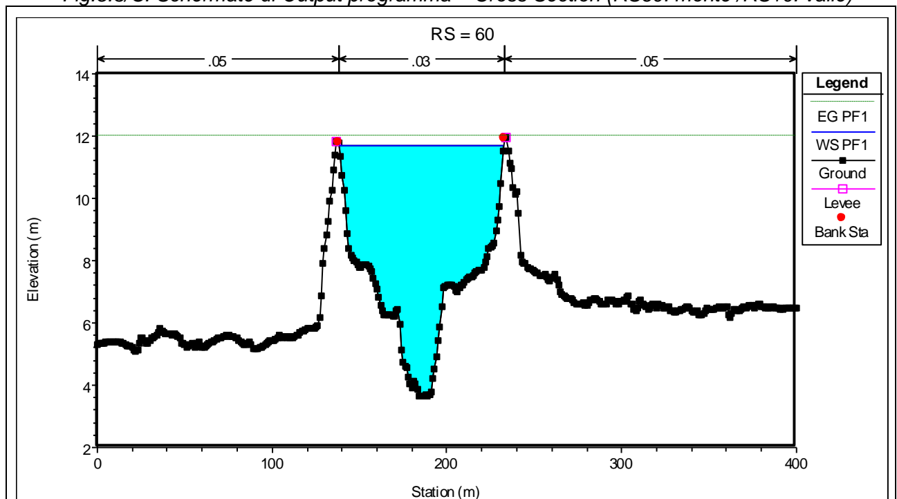
Fig.5.3/C: Schermate di Output programma – Cross Section (RS60: monte /RS10: valle)
