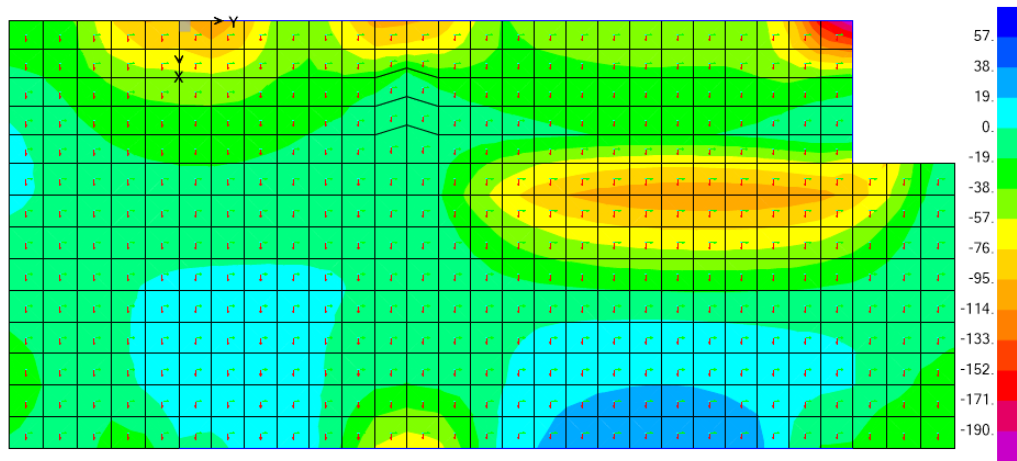
Figura 39: Diagramma taglio V13,min; comb. env_SLU/1.1SLV/SLD
