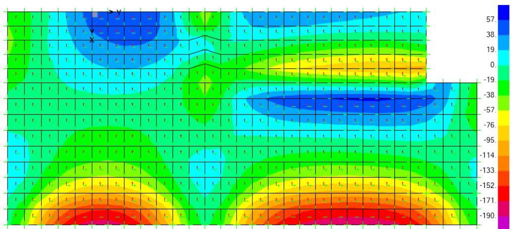
Figura 57: Diagramma taglio V13,min; comb. env_SLU/1.1SLV/SLD
