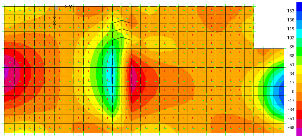
Figura 58: Diagramma taglio V23,max; comb. env_SLU/1.1SLV/SLD
