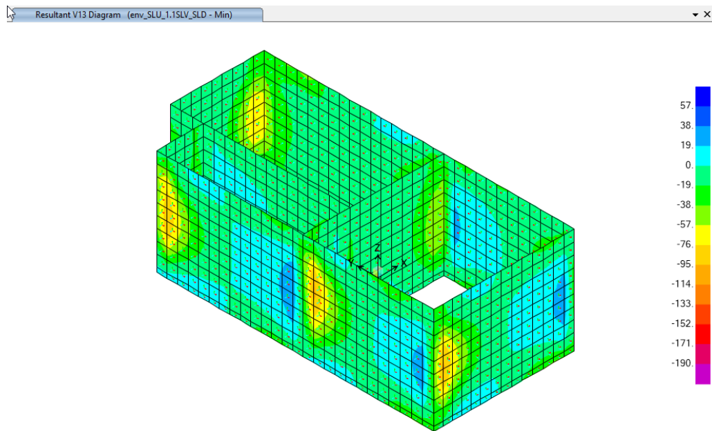
Figura 49: Diagramma taglio V13,min; comb. env_SLU/1.1SLV/SLD
