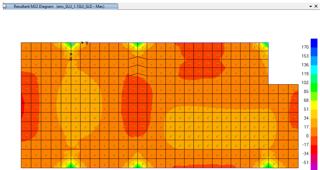
Figura 36: Diagramma momento flettente M_{22,max} ; comb. env_SLU/1.1SLV/SLD
