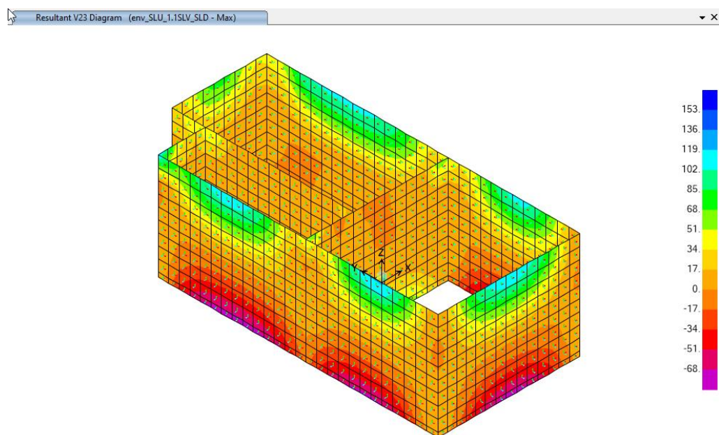
Figura 50: Diagramma taglio V23,max; comb. env_SLU/1.1SLV/SLD
