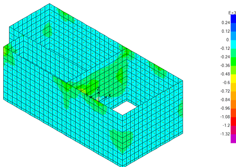
Figura 42: Diagramma sforzo normale N11,,min; comb. env_SLU/1.1SLV/SLD
