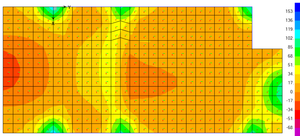
Figura 40: Diagramma taglio V23,max; comb. env_SLU/1.1SLV/SLD
