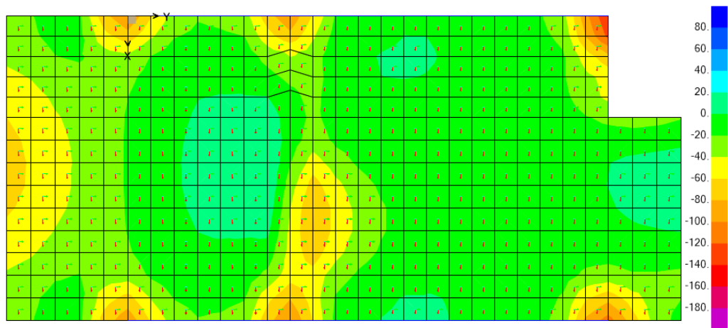
Figura 41: Diagramma taglio V23,min; comb. env_SLU/1.1SLV/SLD
