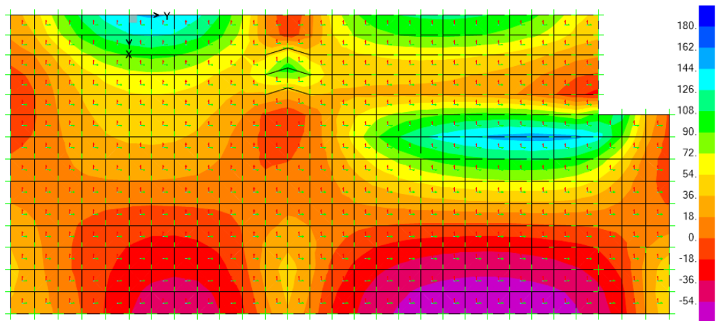
Figura 56: Diagramma taglio V13,max; comb. env_SLU/1.1SLV/SLD
