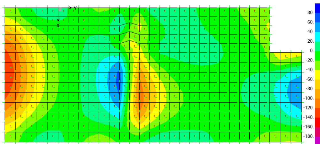
Figura 59: Diagramma taglio V23,min; comb. env_SLU/1.1SLV/SLD
