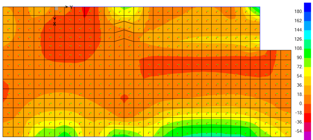
Figura 38: Diagramma taglio V13,max; comb. env_SLU/1.1SLV/SLD
