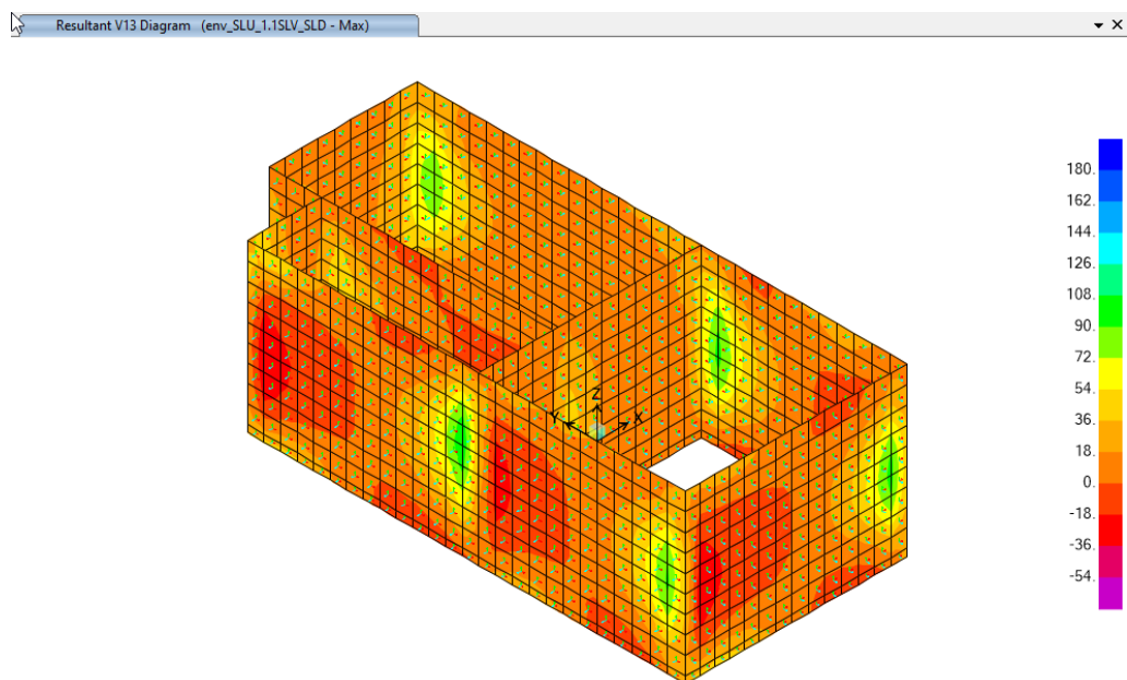
Figura 48: Diagramma taglio V13,max; comb. env_SLU/1.1SLV/SLD
