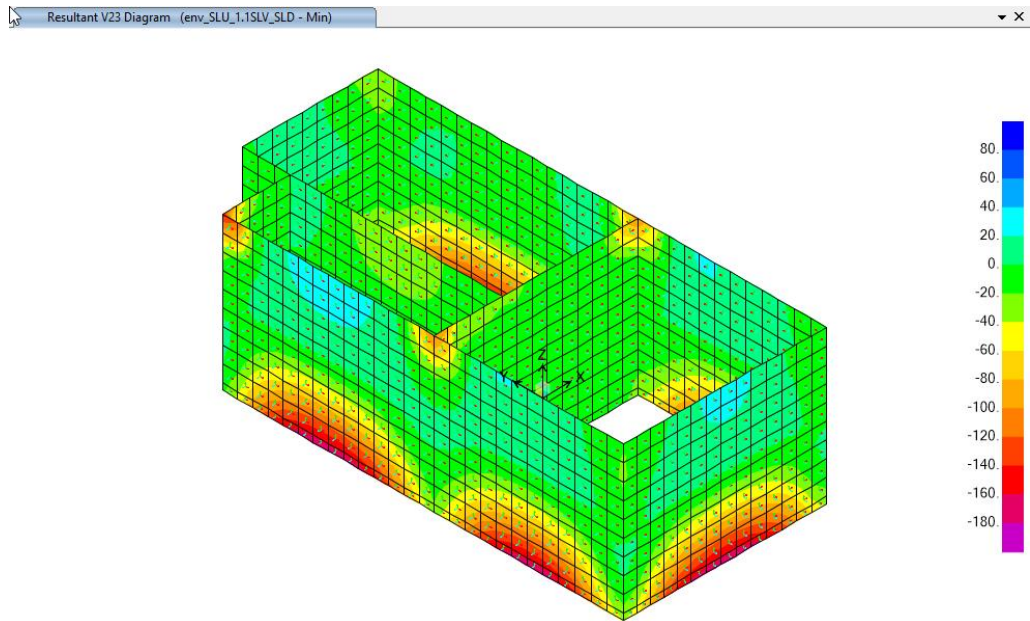
Figura 51: Diagramma taglio V23,min; comb. env_SLU/1.1SLV/SLD
