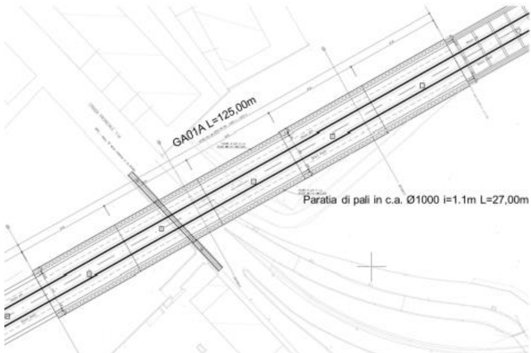
Figura 5-17 – GA01A Pianta (NM2701D26P9GA0100001).
