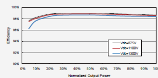
Inverter Efficiency Curve
