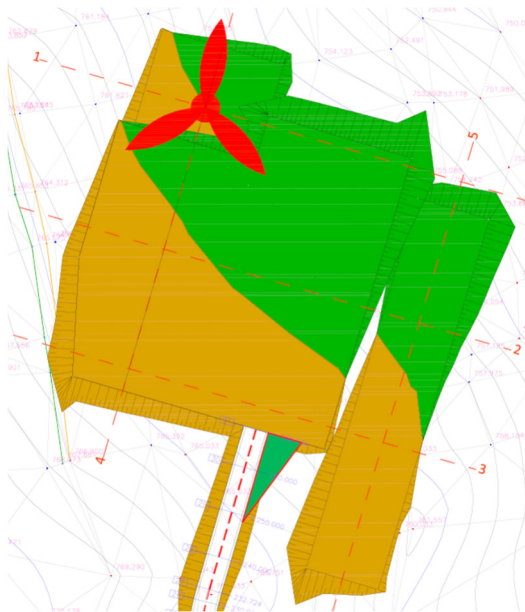
Figura 6: Planimetria BCN01
